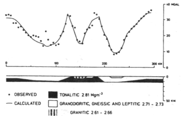
Fig. 3. Gravity profile of the Uppland structure.
