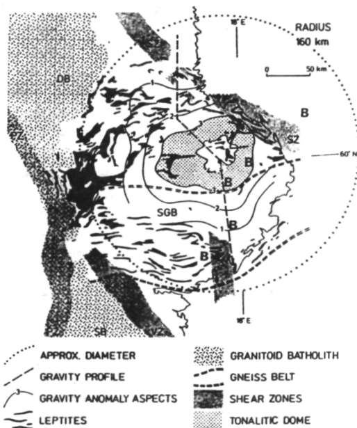
Fig. 2. Uppland structure. SGB = Sormland Gneiss Belt; SZ = Singö Shear Zone; PZ = Protogin Zone; VZ = Västerås Shear Zone; DB = Dala Batholiths; SB = Småland Batholiths; B = breccia dyke occurrences.
