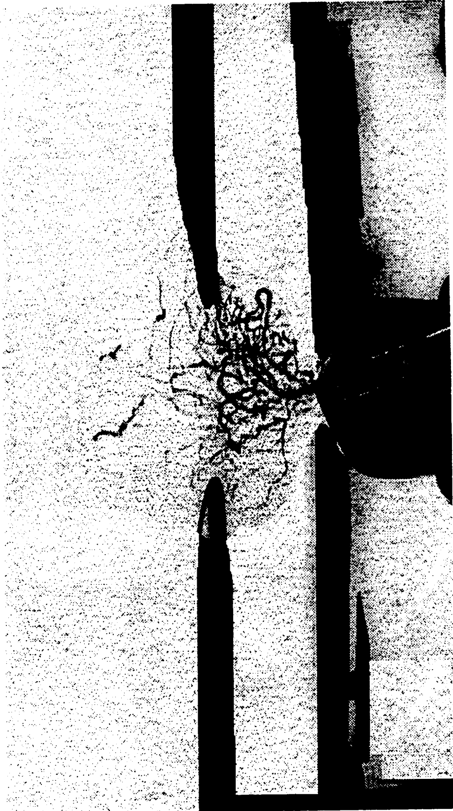
Figure 2.7 Computer enhanced digitized photo of fountain flow. Viewer in front of model. Bubbles are injected into the stagnation region on the center of the wing on the rotor/rotor axis showing highly turbulent up-flow between rotors and recirculating flow. 1/2 second exposure time.
