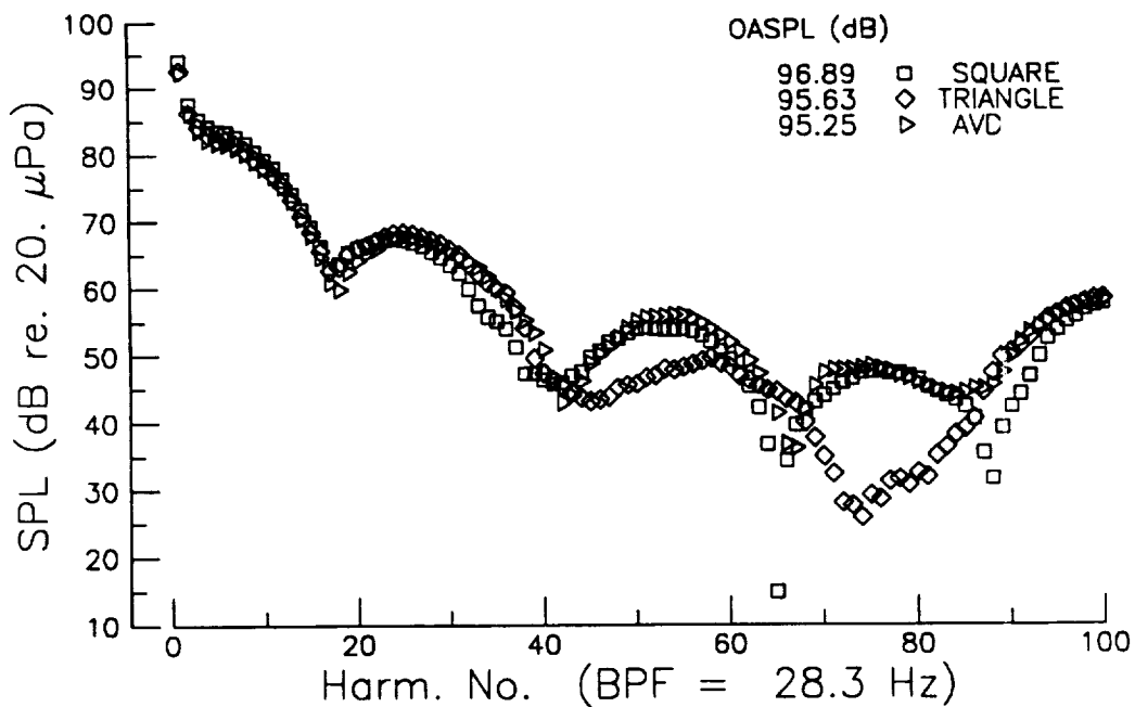
Figure 3.13 Comparison of predictions with different chordwise loading distributions. Loading noise. Square: constant chordwise loading. Triangle: triangular loading distribution. AVD: chordwise accurate loading distribution. Levels not corrected for comparison to experiment.
