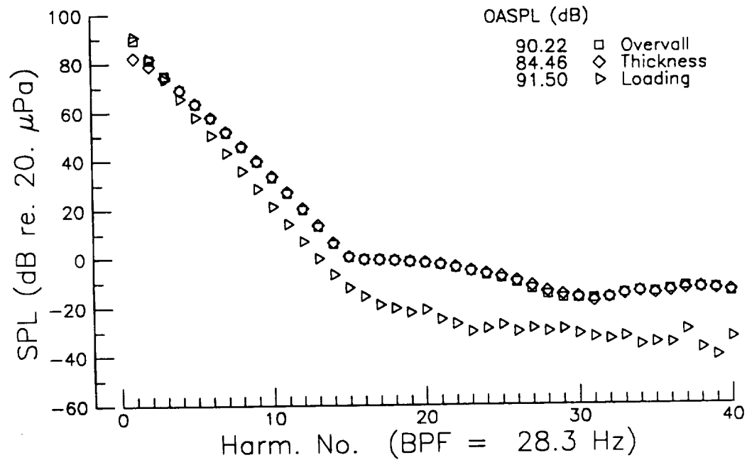
Figure 3.9 Prediction without the fountain model showing thickness, loading and overall sound levels. Acoustic pressure time history and sound spectrum. Levels not corrected for comparison to experiment.
