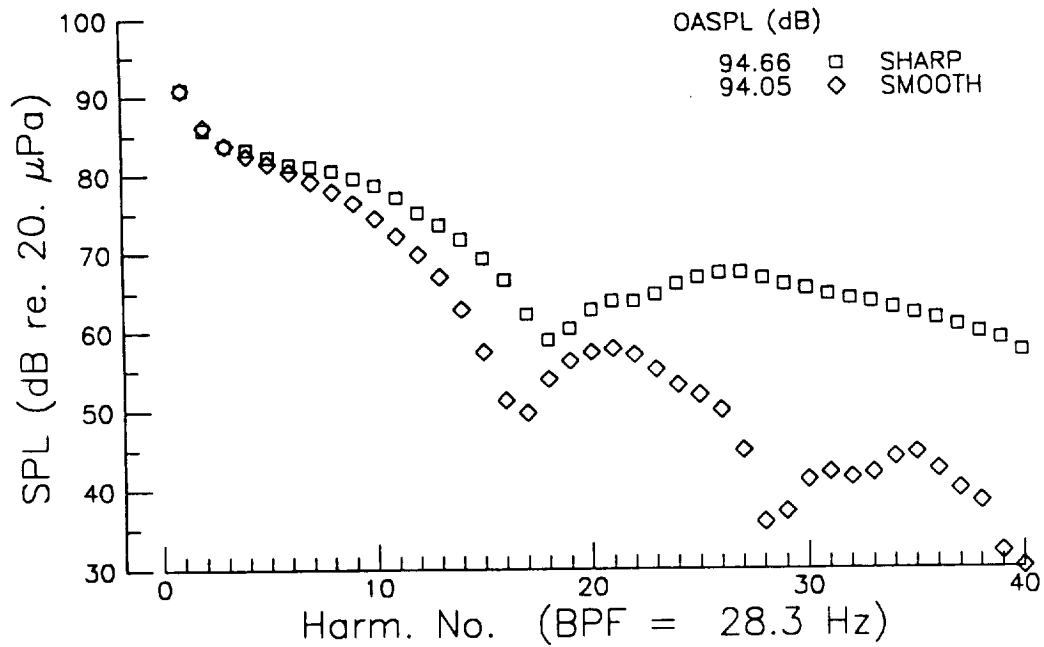
Figure 3.12 Comparison of predictions with 'sharp' and 'smooth' fountain models. Overall noise. Acoustic pressure time history and sound spectrum. Near in-plane rear aircraft acoustics. Levels not corrected for comparison to experiment.
