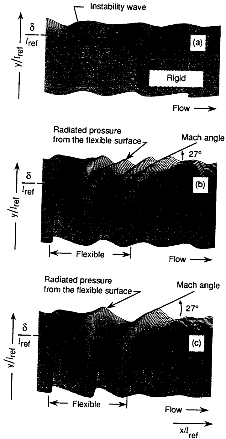
Fig. 5: Instantaneous pressure distribution in the flow-field. (a) TS type waves over a rigid surface, (b) TS type waves over a vibrating flexible surface, sound source frequency f/4 , (c) sound source frequency f/8 .
