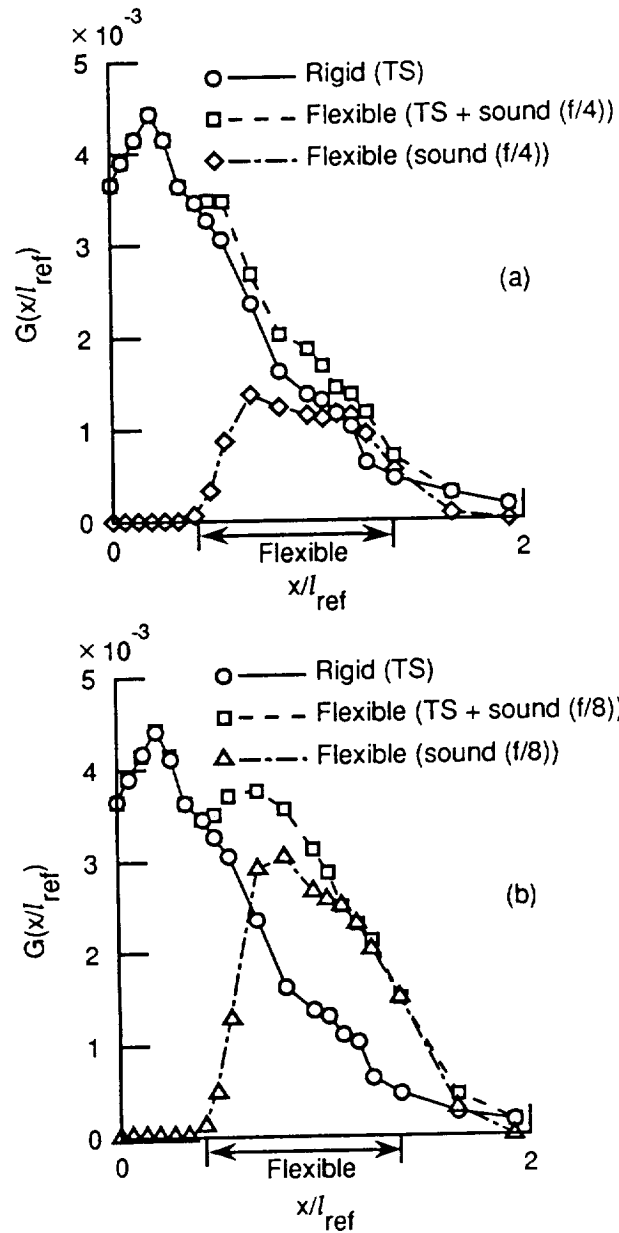
Fig. 4: Comparison of disturbance levels generated by a TS type waves over a rigid surface to that generated by a vibrating flexible surface (no TS waves) and to that generated by the interaction of the TS waves with the vibrating surface. (a) Sound source frequency of f/4 , (b) Sound source frequency of f/8 .
