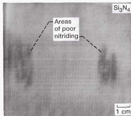
Figure 3.—Ultrasonic, 10 MHz, through transmission c-scan of monolithic \text{Si}_3\text{N}_4 , actively cooled panel.
