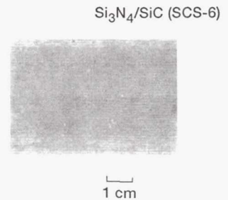
Figure 19.—Radiographed section of \text{Si}_3\text{N}_4/\text{SiC} SCS-6 [0] RBSN tensile test bar.
