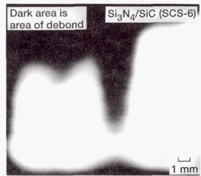
Figure 25.—Ultrasonic, 10 MHz, through transmission c-scan of section of \text{Si}_3\text{N}_4/\text{SiC} SCS-6 [0] RBSN tensile test bar.
