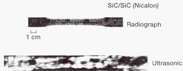
Figure 10.—Ultrasonic, 10 MHz through transmission c-scan and radiograph of SiC/SiC (Nicalon) woven laminated composite.
