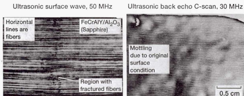
Figure 32.—Ultrasonic surface wave and back echo images of FeCrAlY/Al 2 O 3 (sapphire fiber) composite.
