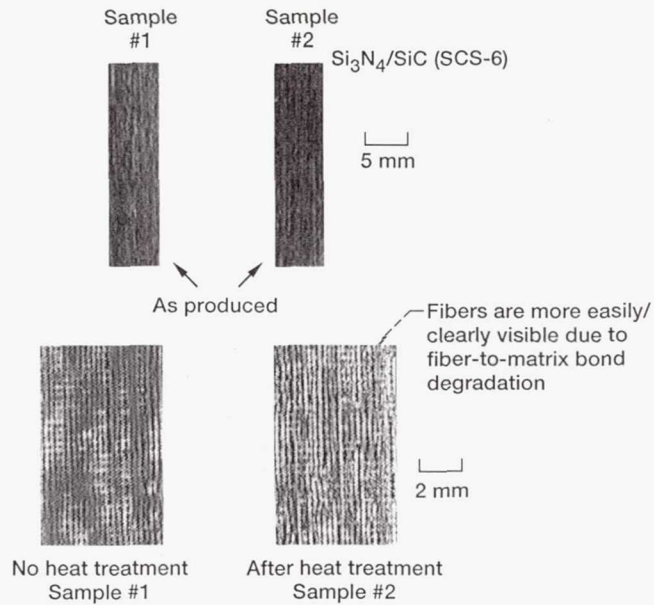
Figure 26.—DERCI images of \text{Si}_3\text{N}_4/\text{SiC} SCS-6 [0] RBSN at 50 MHz before and after heat treatment.
