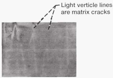
Figure 22.—Fluorescent penetrant image of section of \text{Si}_3\text{N}_4/\text{SiC} SCS-6 [0] RBSN tensile test bar.
