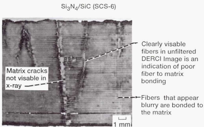
Figure 20.—Ultrasonic DERC I unfiltered image at 50 MHz of section of \text{Si}_3\text{N}_4/\text{SiC} SCS-6 [0] RBSN tensile test bar.
