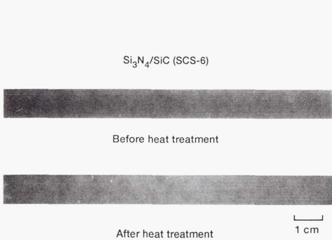
Figure 28.—Radiographs of \text{Si}_3\text{N}_4/\text{SiC} SCS-6 [0] RBSN sample #2 before and after heat treatment.
