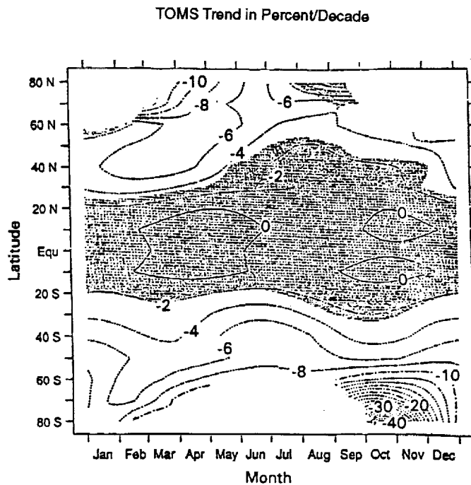
Figure 2-11 Trend obtained from TOMS total ozone data as a function of latitude and season. Data included extends from November 1978 through March 1991. Unshaded area indicates where trends are statistically significant at the 2σ level (Bloomfield, personal communication, 1991).
