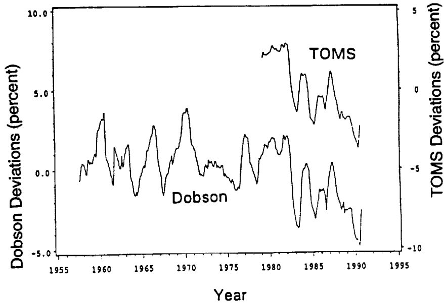
Figure 2-10 A comparison of TOMS and Dobson data for northern middle latitudes. The TOMS series is deseasonalized mean ozone over 40°–52° N. The Dobson series is the composite series constructed from deseasonalized ozone for stations in the latitude range 40°–52° N. The data plotted are a 1-year moving mean, which smooths high-frequency variations, but broadens and decreases the amplitude of large excursions such as that of the winter of 1982–1983.
