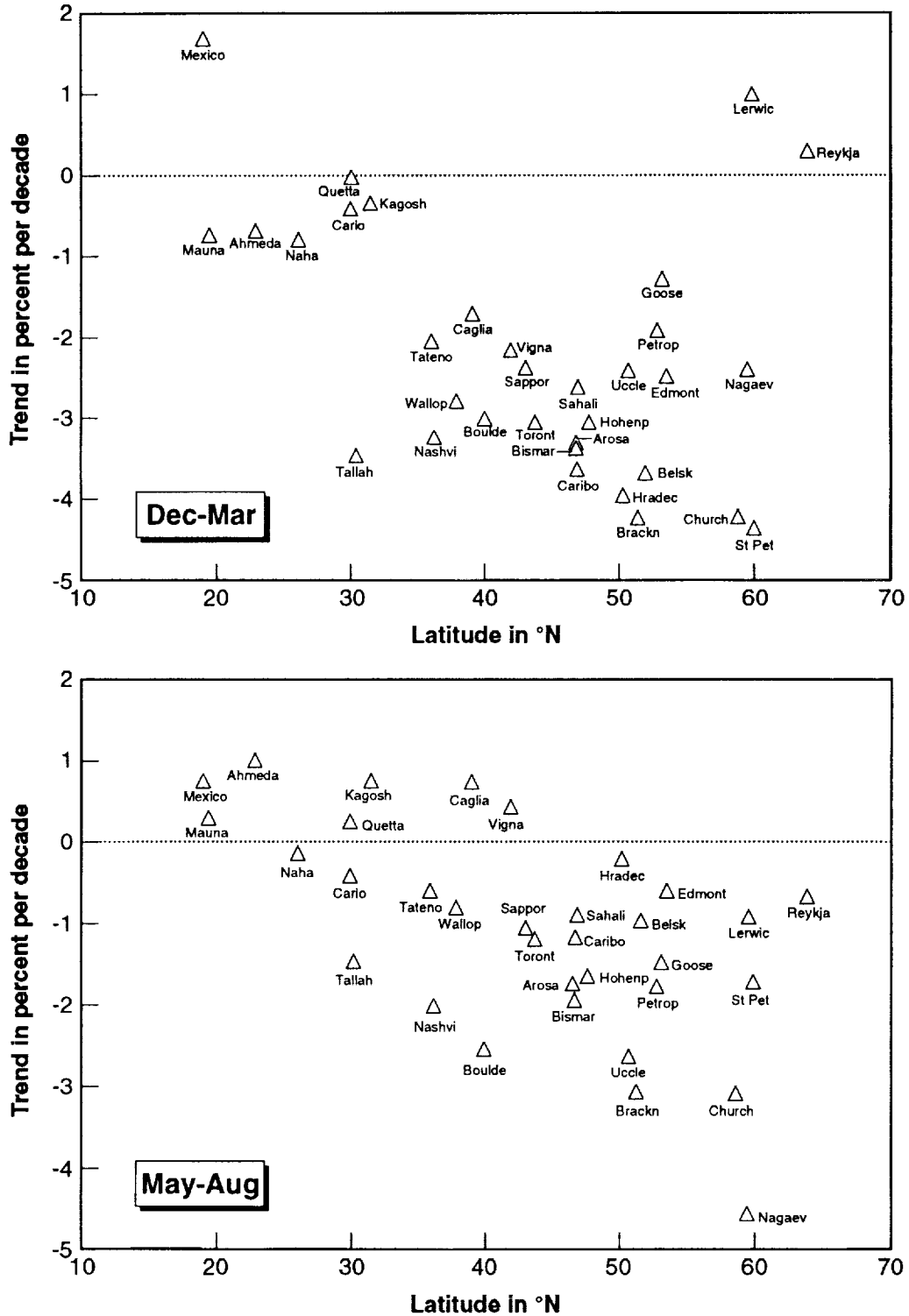
Figure 2-6a Individual station long-term trends, by season, for 39 Northern Hemisphere stations, versus station latitude. The estimates were derived from the standard seasonal model using data from 1958 through 1969 as a baseline, and monthly linear trends over the period 1970 through March 1991.
