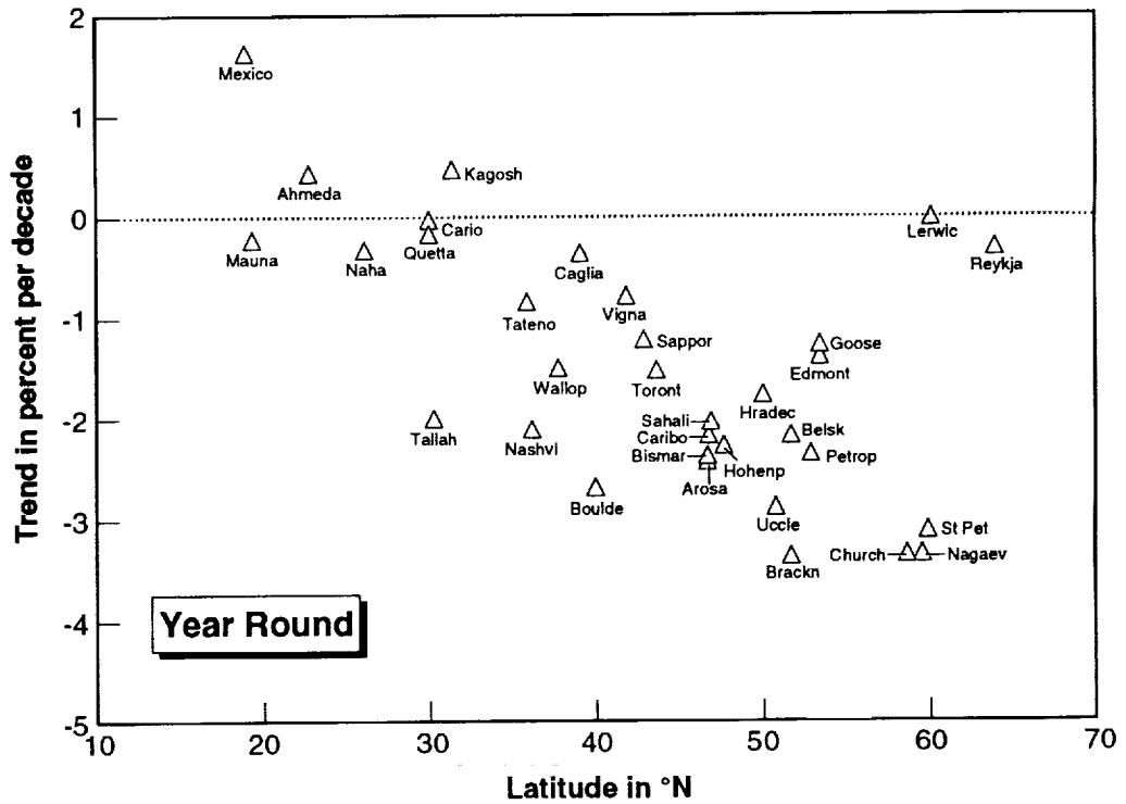
Figure 2-6b Individual station long-term trends, by season, for 39 Northern Hemisphere stations, versus station latitude. The estimates were derived from the standard seasonal model using data from 1958 through 1969 as a baseline, and monthly linear trends over the period 1970 through March 1991.
