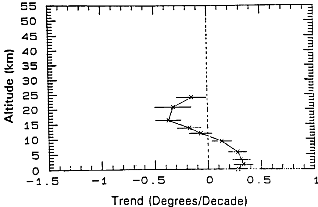
Figure 2-19 Rawinsonde temperature trend estimates in ^\circ\text{C} per decade as a function of altitude. Horizontal bars represent 95 percent confidence limits of estimated trends (Miller et al. , 1991).
