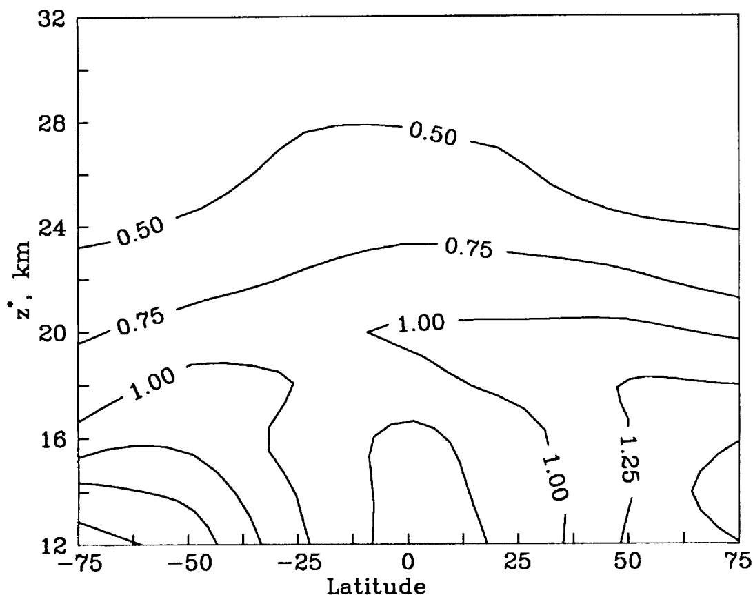
Figure 3-5 Sulfate aerosol surface area ( \mu\text{m}^2\text{cm}^{-3} ) derived from SAGE II data for January to March 1989 using segmented power law size distribution model. z^* = 16 \log_{10}(1000/\text{pressure [mbar]}) .
