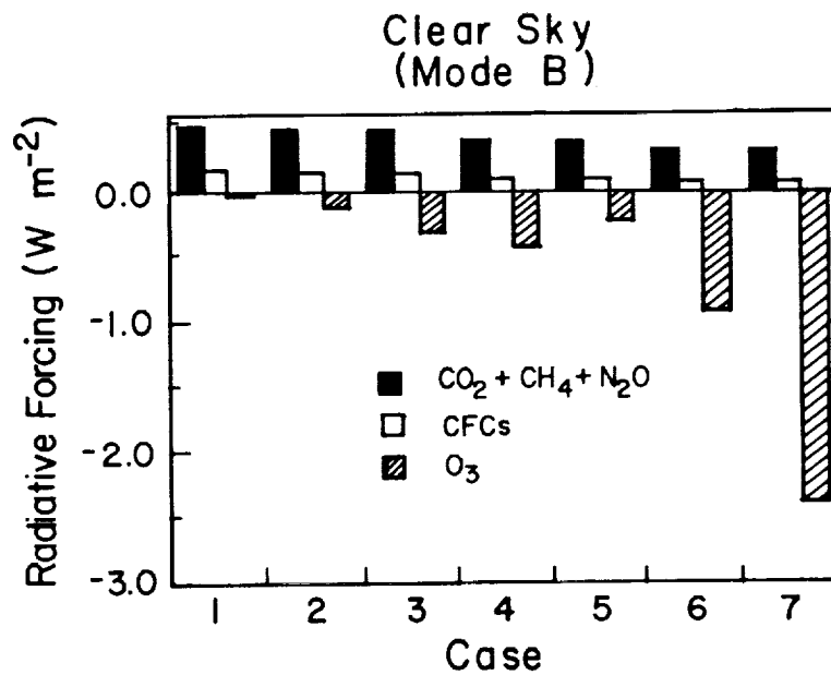
Figure 7-2 Radiative forcing due to CO 2 +CH 4 +N 2 O, CFCs only, and that due to lower stratospheric ozone losses (see 7.5.1) at various locations and times of the year listed in Table 7-6. The seven cases employ clear-sky atmospheric profiles (McClatchey et al. , 1972). Upper panel shows Mode A results and the lower panel Mode B results (Model I computations). Numerical values are tabulated in Table 7-7.
