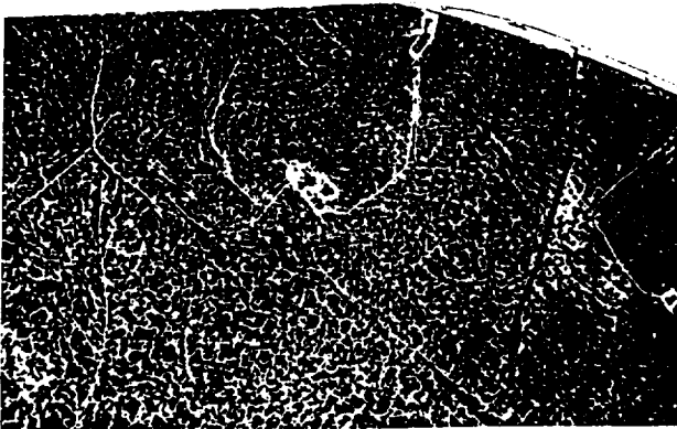
Figure 1. Polygonization area in a (001) KOH etched wafer.
