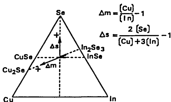
Figure 1. Triangle diagram for the system \text{Cu-In-Se} .
