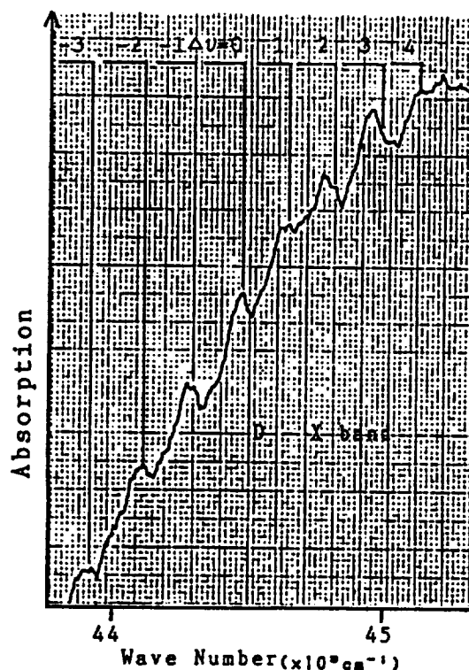
Figure 1. Absorption spectrum of D-X band system of Au 2
