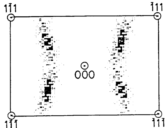
Figure 2. Step // [\bar{1}10] .
