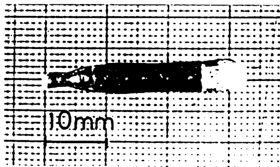
Figure 1. As-grown boule of Ba_{0.985}Sr_{0.015}TiO_3 .
