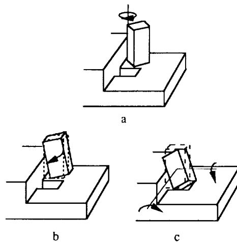
Figure 13: Combined Compliant Motions
