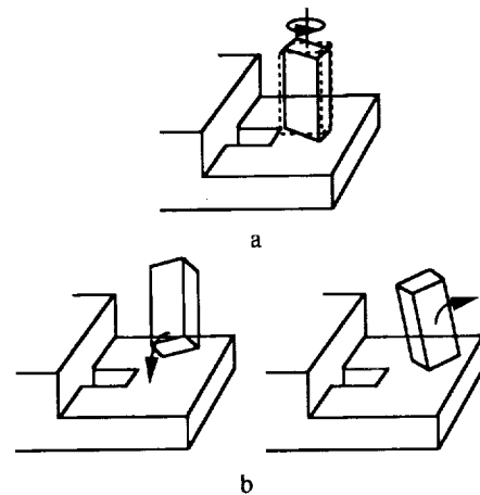
Figure 12: Compliant Rotations
