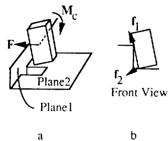
Figure 14: Force/Moment for a Combined Motion of Translation/Frictional-Rotation
