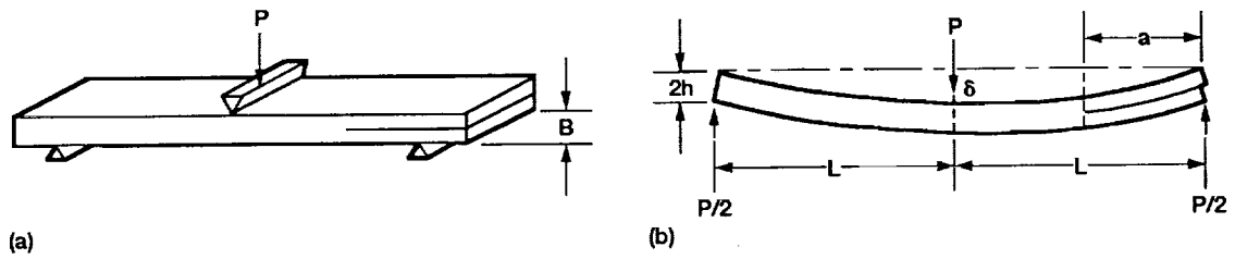
(a) Test specimen geometry. (b) Deformed shape.
