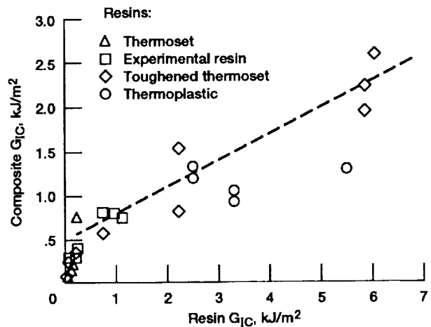
Figure 43.—Strain energy release rates for steady interlaminar crack growth versus neat resin toughness (adapted from ref. 30).
