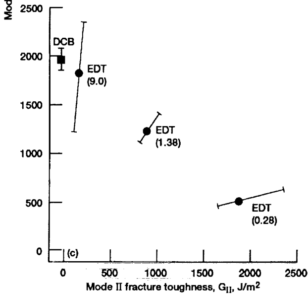
Figure 32.—Fracture toughness calculated with linear mixed-mode failure criterion (adapted from ref. 39).
