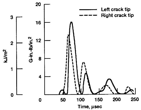
Figure 41.— G_{IIIc} is calculated from finite element analysis of impact test (adapted from ref. 74).
