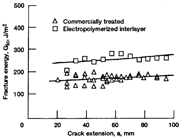
Figure 46.—Increase in G_{IIc} due to electropolymerized interlayer on fiber surface (adapted from ref. 88).
