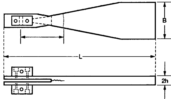
Figure 13.—Width-tapered double cantilever beam (adapted from ref. 17).
