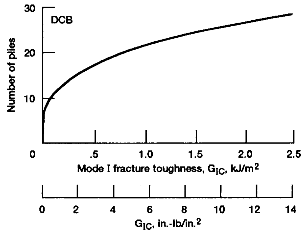
Figure 17.—Minimum DCB specimen thickness required to maintain linear elastic behavior (adapted from ref. 29). a = 152.4 mm (6 in.); E = 138 GPa ( 20 \times 10^6 psi).
