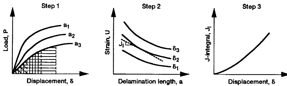
Figure 11.—Experimental procedure for J-integral calculation (adapted form ref. 12).
