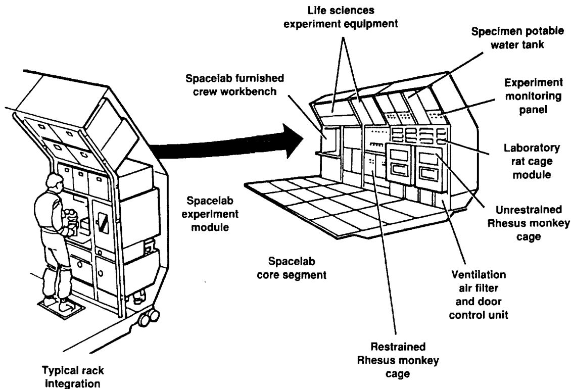
Figure 4. Sketch of Spacelab showing a typical set of Spacelab racks with integrated equipment.
