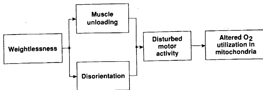
Figure 8. Preliminary integration of the hypothetical main pathways by which microgravity alters the physiology of metazoa as phylogenetically diverse as insects and mammals.
