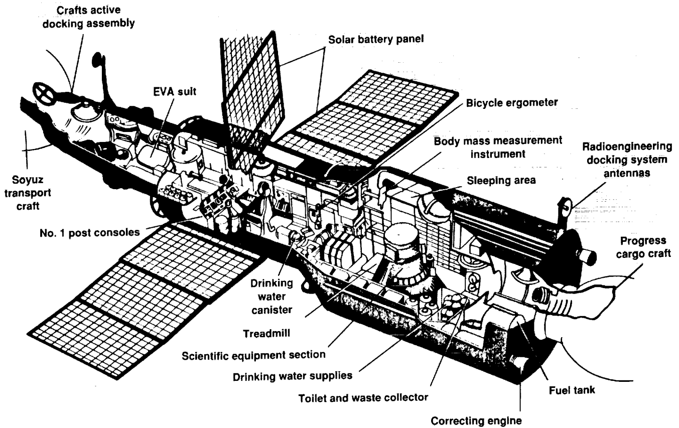
Figure 2. Salyut-6 space station. (Reproduced from ref. 16.)
