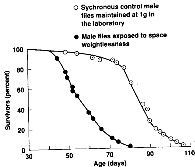
Figure 6. Effects of weightlessness on the life span of Drosophila melanogaster .
