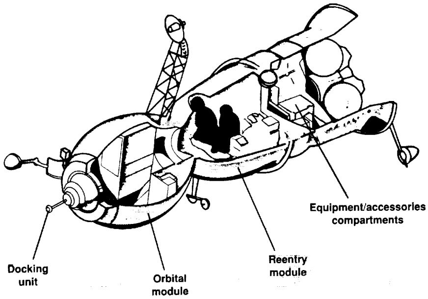
Figure 1. Soyuz vehicle. (Reproduced from ref. 16.)
