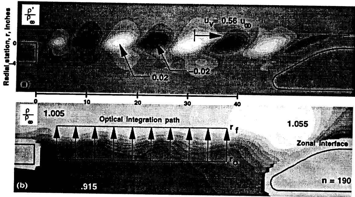
Figure 34: 2-d treated cavity, low lip-blowing rate: instantaneous contours of (a) \frac{\rho'}{\rho_0} and (b) \frac{\rho}{\rho_\infty} with schematic of optical model
