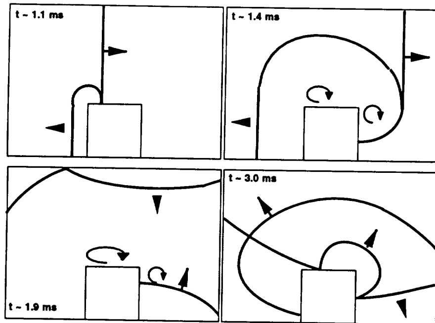
Figure 18: Hemicylinder case: schematic of shock interaction
