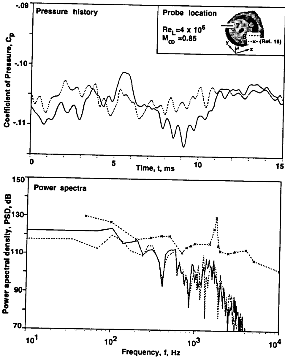
Figure 48: Configuration 100: pressure history and power spectra on primary mirror
