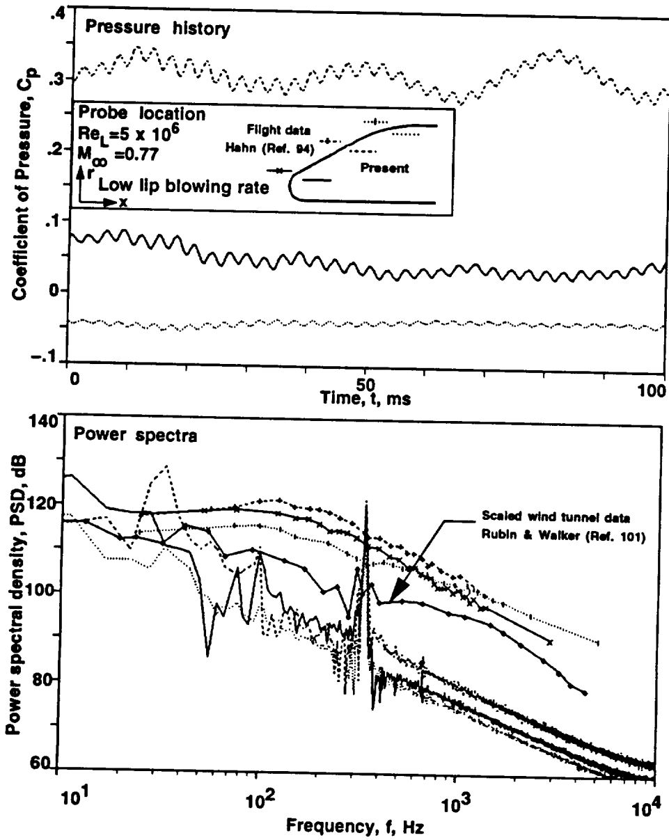
Figure 30: 2-d treated cavity: power spectra, low lip-blowing rate
