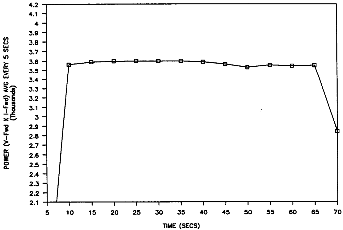
Figure 20. Examples of Power Fluctuations During Constant Parameter Welds
