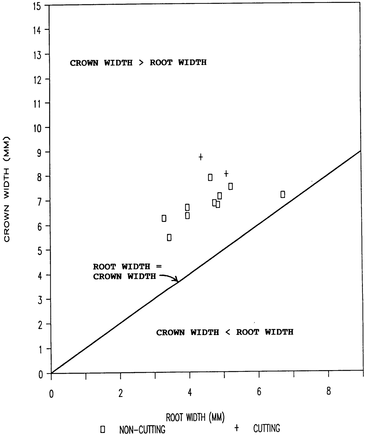
Figure 10. Root Width vs Crown Width, 3/16" Stainless Steel
