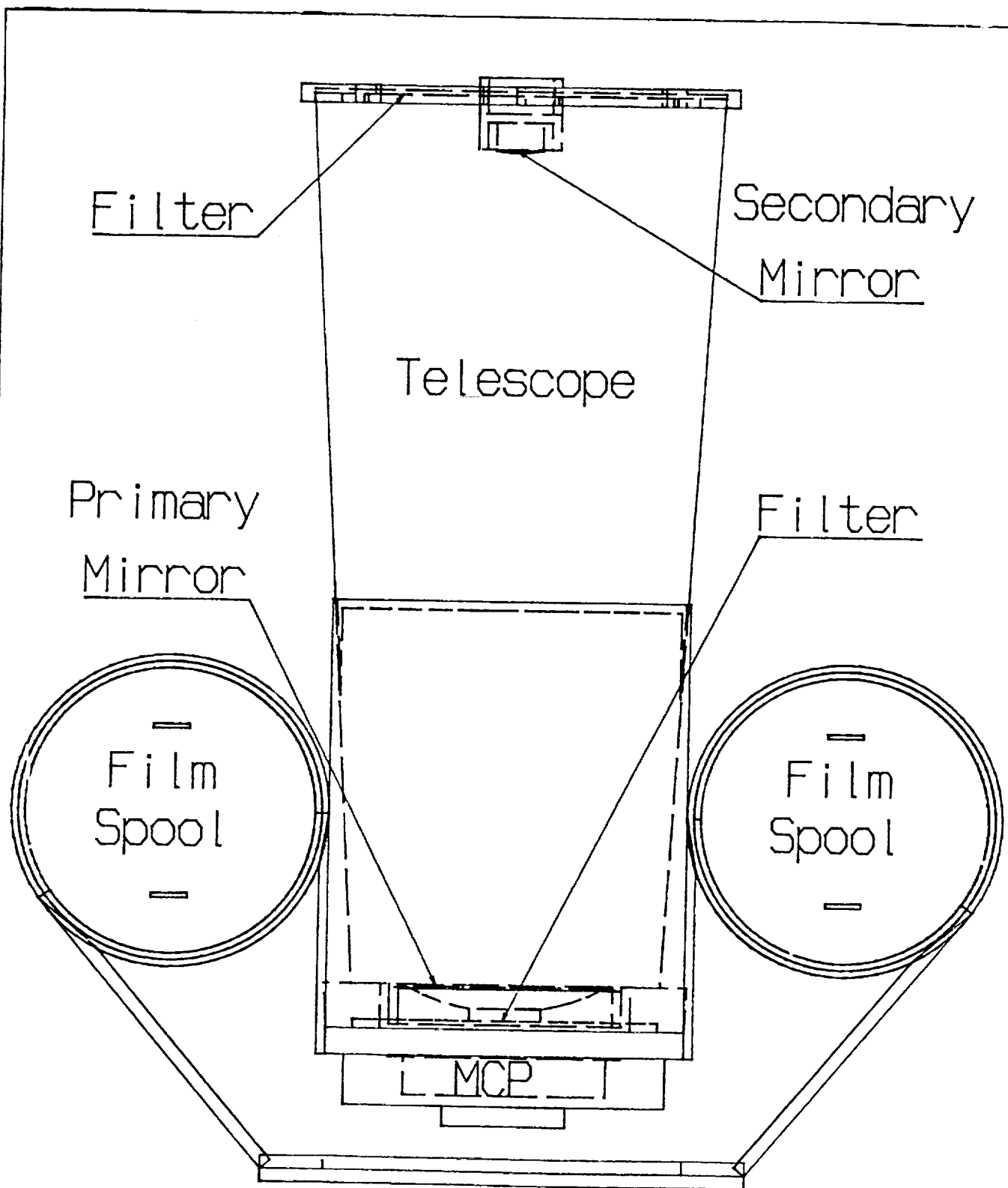
FIGURE 2: A cross-sectional side view of the GOLDHELOX telescope, with all optical components indicated. Dimensions are not to scale.
