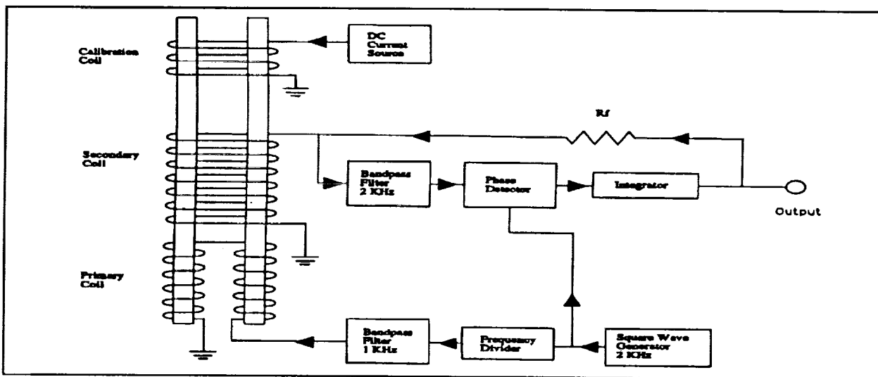
Figure 5. The Fluxgate Magnetometer
