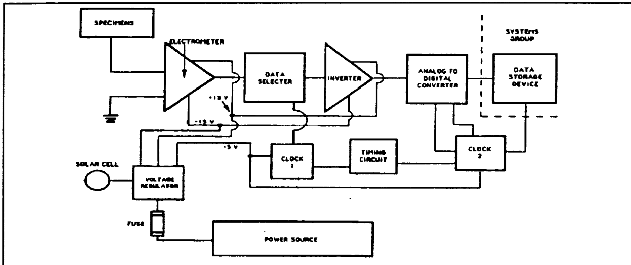
Figure 6. The Photoelectric Effect Experimental Block Diagram.
