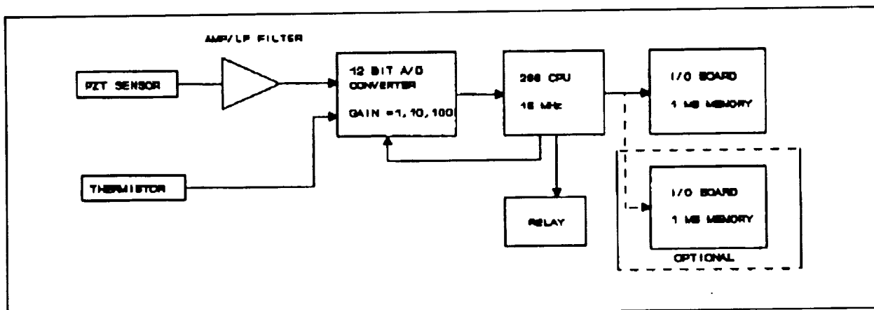
Figure 4. Orbital Debris Detection Experimental Block Diagram
