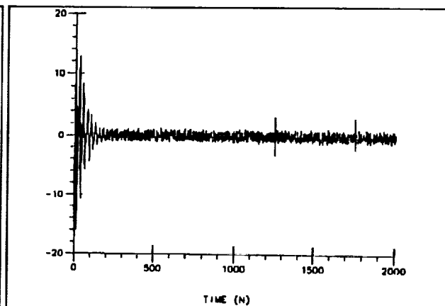
Figure 3. Processed Signal using LMS Algorithm.
