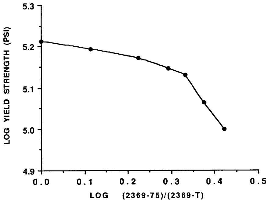
Fig. 9 Effect of Temperature ( ^{\circ} F) on Yield Strength for Inconel 718. (Log-Log Plot)
