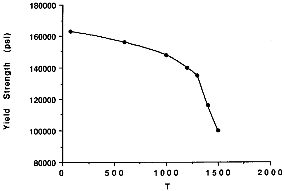
Fig. 8 Effect of Temperature ( ^{\circ} F) on Yield Strength for Inconel 718. (Linear Plot)
