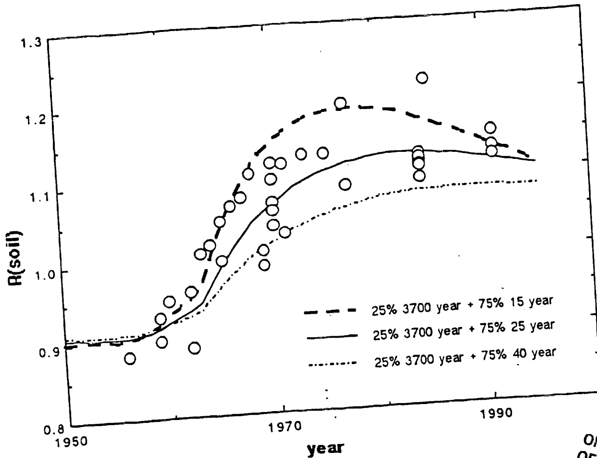
Figure 7: Title: R(soil) model predictions and R(soil) observations vs time
