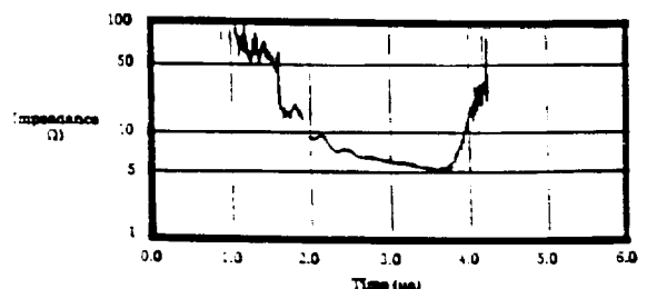
Figure 16: Discharge impedance.
