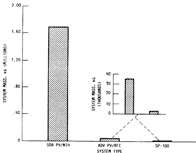
Fig. 1. Power systems mass comparison.
