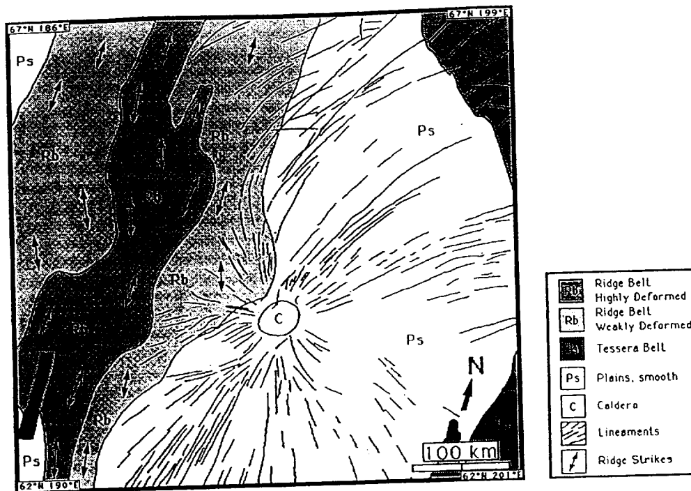
Fig. 1. Arachnoid in Vinmara Planitia. The lineaments shown include graben, fissures, and fractures. Note the right-angle intersection with the adjacent tessera belt, as well as the unusual behavior to the northwest of the caldera. For details, see text.
