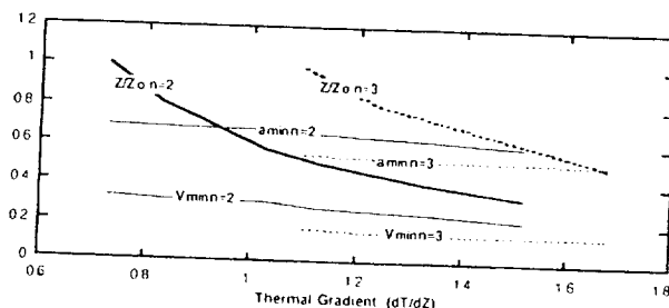
Fig. 2. Plot of the results for basaltic pluton ascent on Venus. The results are nondimensionalized by the corresponding terrestrial values, and the source depth values are the direct result of the assumed planetary thermal structure (equation (1)). For example, for a Venus thermal gradient the same as the terrestrial thermal gradient and n = 2 , the corresponding minimum source depth is about 60% of the terrestrial value the minimum ascent velocity is about 30% of Earth's and the minimum body size is about 70% of Earth's. Thermal structure parameters: n = 2 ; dT/dZ = 1.0 ( dT/dZ of Earth); Z_0 = 1.0 ( Z_0 of Earth).
