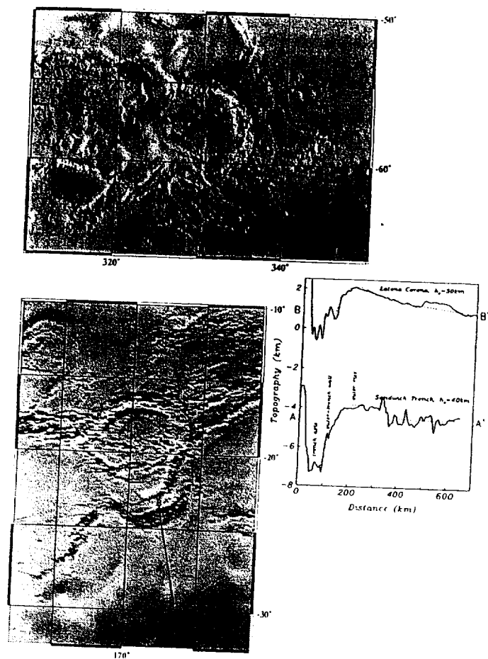
Fig. 1. (Top image) Bathymetry of South Sandwich Trench (Earth) as a tall volcanic ridge, a deep ocean trench, and the characteristic trench/outer rise signature associated with lithospheric flexure prior to subduction (A-A'). (Bottom image) Topography of Latona Corona (East Aphrodite, Venus) at the same horizontal and vertical scale as the Sandwich Trench (top). The southern arc displays a prominent ridge-trench-outer rise signature (B-B'). The southernmost ridge is not massive enough to maintain the bending moment of the trench/outer rise flexure. Additional bending moment can be supplied by a subducted slab or by the second interior ridge.
