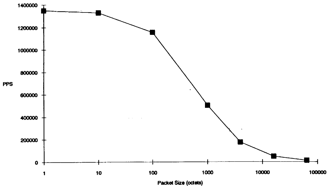
HIPPI Switch Packet Throughput
