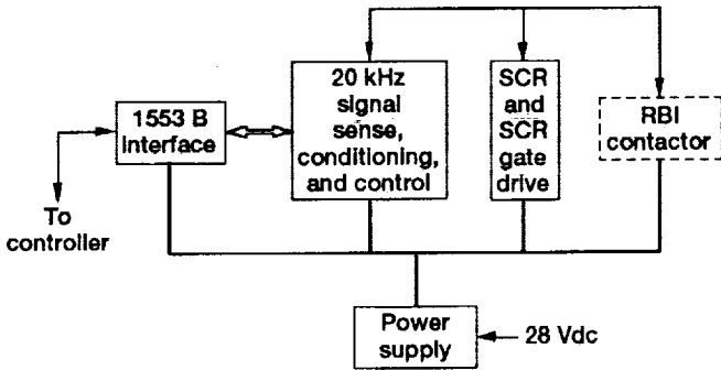
Figure 2.—Basic functional circuits used for each remote power controller (RPC) and remote bus isolator (RBI), including the RBI's contactors.
