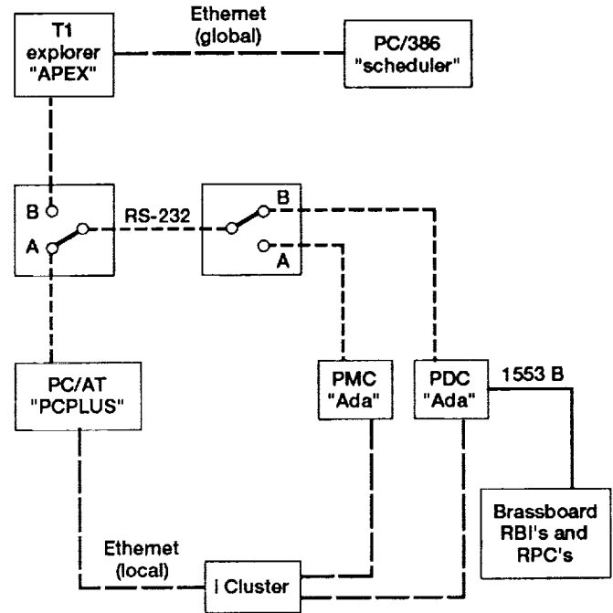
Figure 3.—Brassboard control elements, interfaces, and software.
