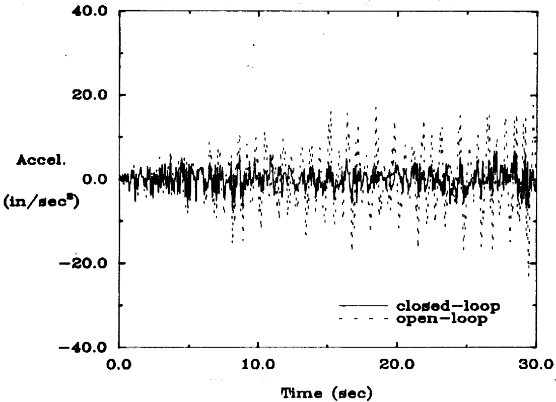
Figure 55: Open/closed-loop experimental results and FEM simulations of the frequency matched AVA controller at sensor 8 under random input at all 8 actuators.
