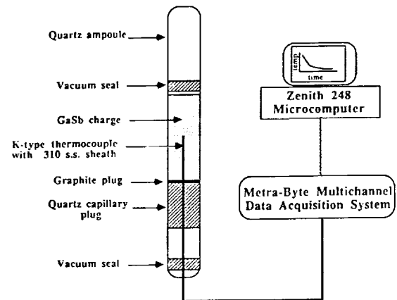
Fig. 3. Schematic diagram of ampoule and thermocouple arrangement with data acquisition system for in-situ temperature measurements.
