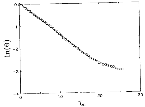
Fig. 5. Experimental data and the resulting linear fit ( R^2 = 0.9993 ) for experiment 1.
