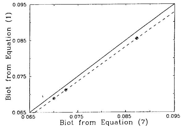
Fig. 6. Comparison between the Biot numbers calculated from the slope using eq. (1) (lumped-capacity model) and using eq. (7). The horizontal and vertical lines in the figure represent 95% confidence limits on the values of the Biot number. The dashed line represents the calculated relative error between the two models and is given by eq. (10).
