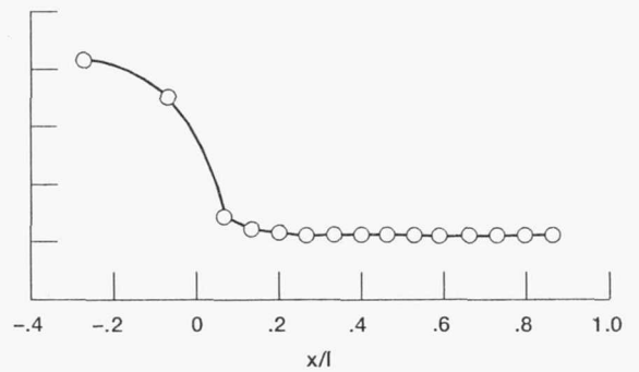
Figure 29.—Effect of ramp curvature on ramp centerline pressure distributions—short ramps.
