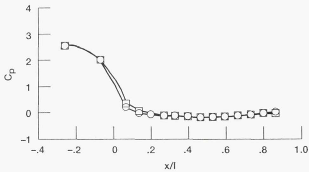
Figure 29.—Effect of ramp curvature on ramp centerline pressure distributions—short ramps.
