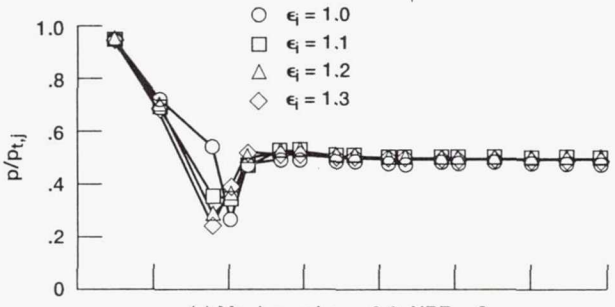
(a) Mach number = 0.0, NPR = 2.
