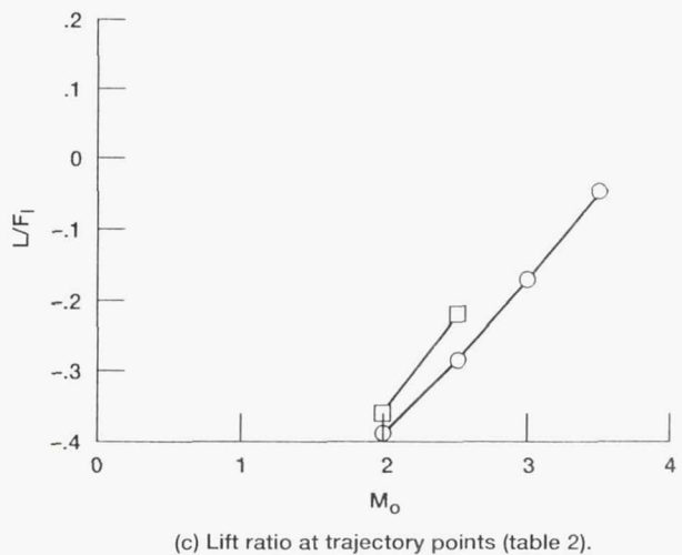
Figure 31.—Effect of ramp curvature on installed performance—long ramps ( \epsilon_i = 1.0 , long sidewalls).
