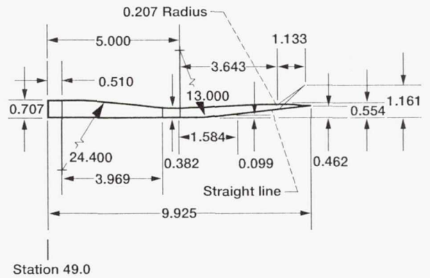
(b) Cowl boattail angle geometry variations (dimensions in in.).
