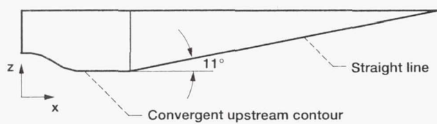
(b) Long straight 11° ramp.
