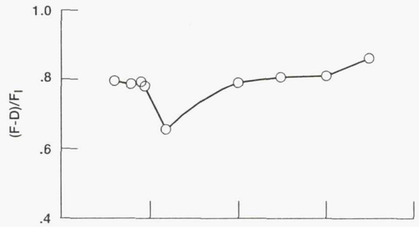
(a) Net thrust ratio at points along NPR-Mach number schedule (table 2).
