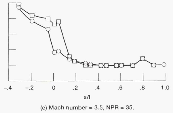
Figure 26.—Effect of boattail angle on ramp centerline pressure distributions.
