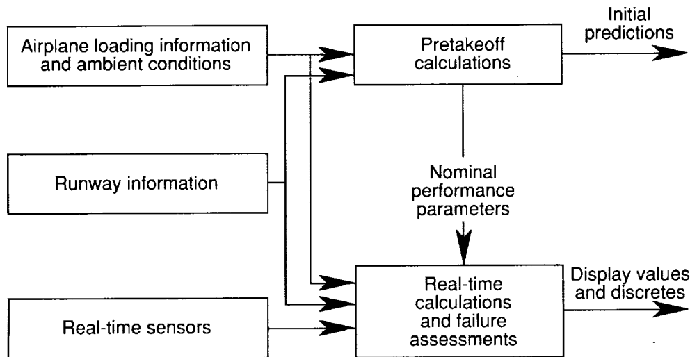
Figure 1. Block diagram of TOPMS algorithm functions.
