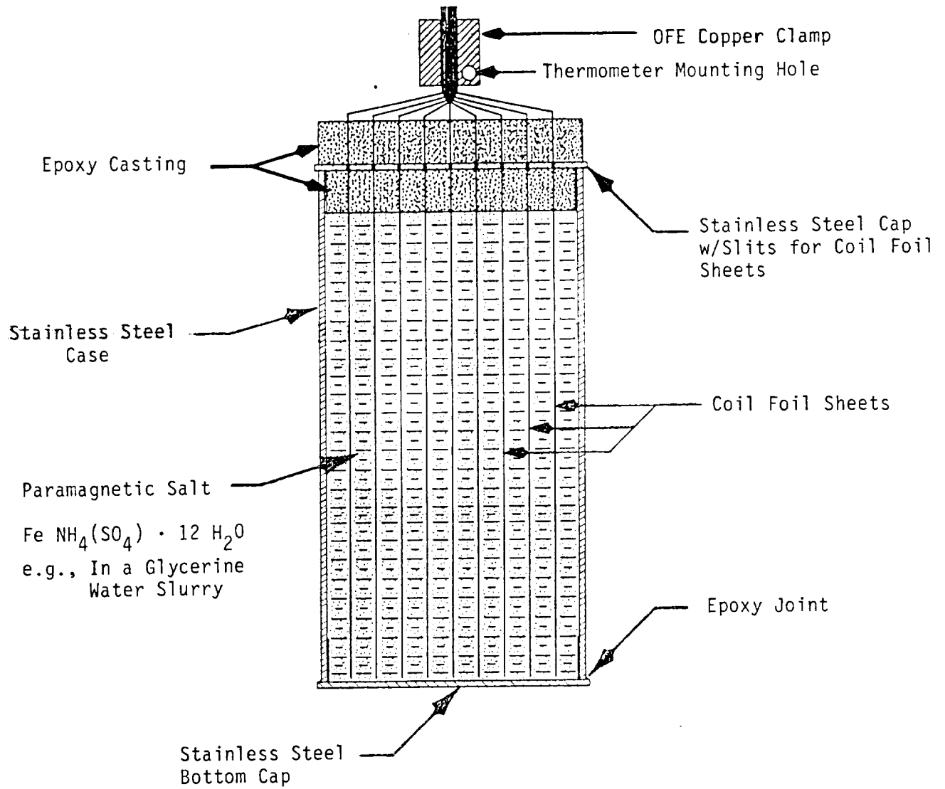
Figure 27 Schematic Representation of ADR Salt Pill
