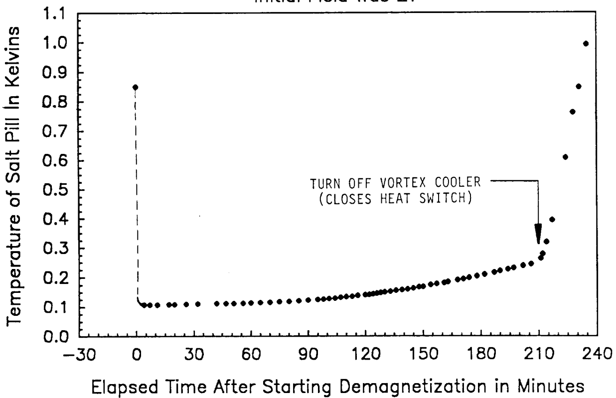
Figure 29 Cooling curve for the ACE, Inc. Adiabatic Demagnetization Refrigerator
