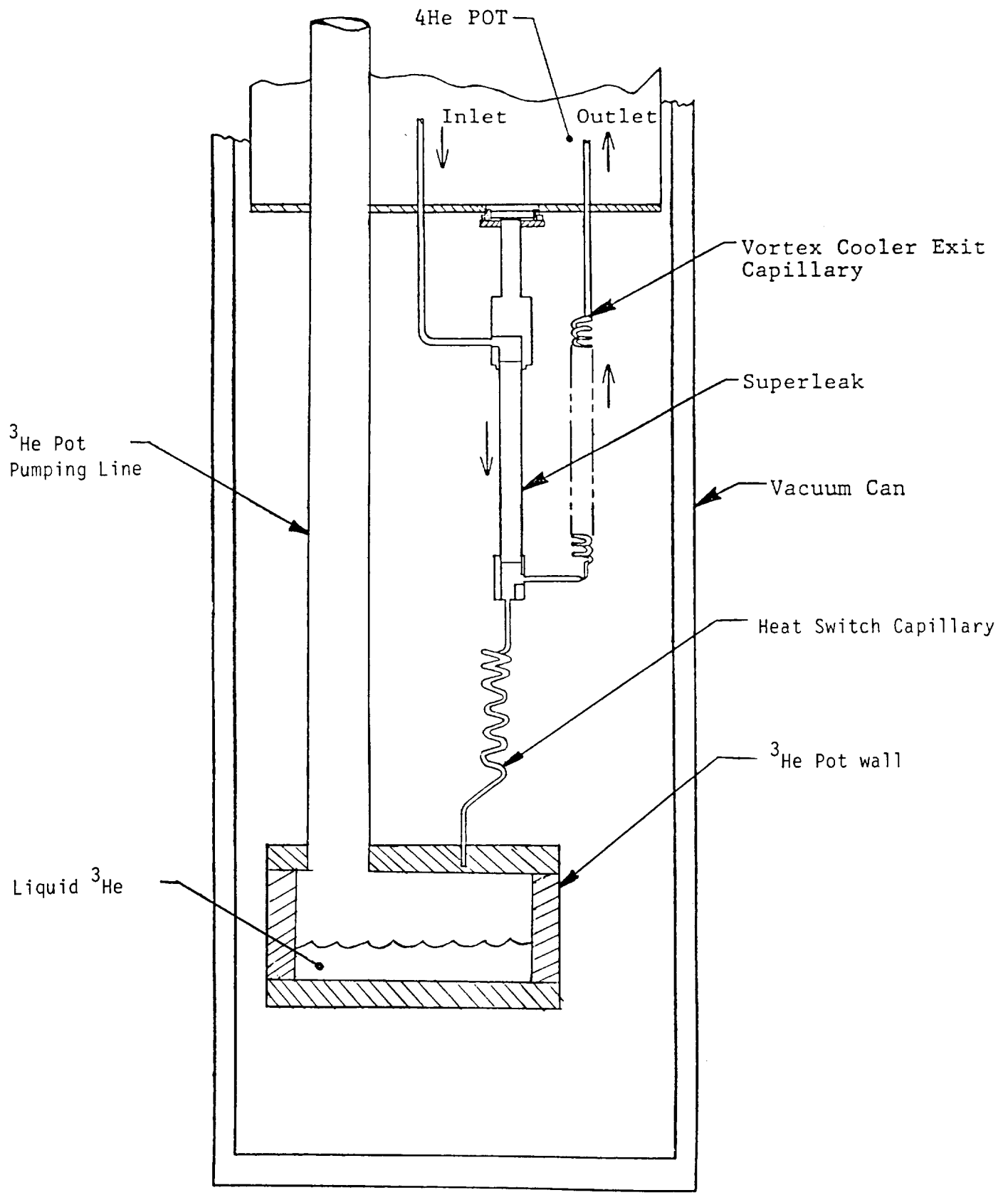
Figure 24 Auxillary Test Facility for evaluating the Conduction of Superfluid filled Capillaries. The Fountain Pump and Heat Exchanger are omitted from the drawing for clarity. 56
