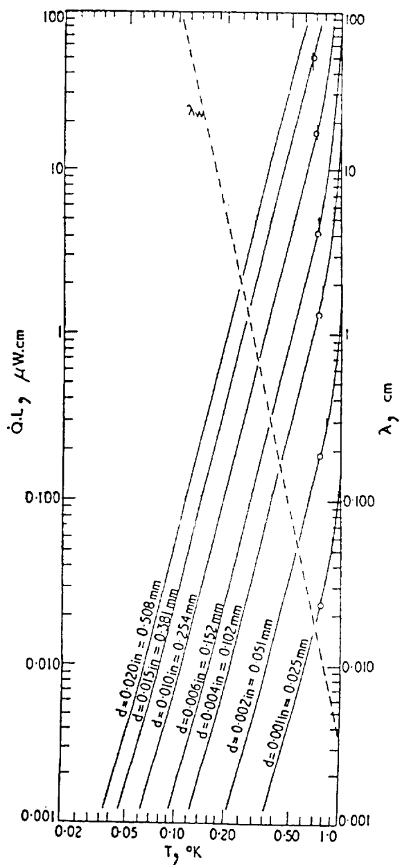
Figure 12 Heat Leak Along Superfluid Filled Capillaries as a Function of Temperature for ( 0.02 \text{ K} < T < 1.0 \text{ K} ). The data is shown for different capillary diameters.
