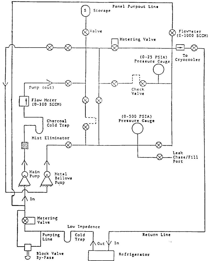
Figure 10 ^3\text{He} Cryocooler Gas Handling System
