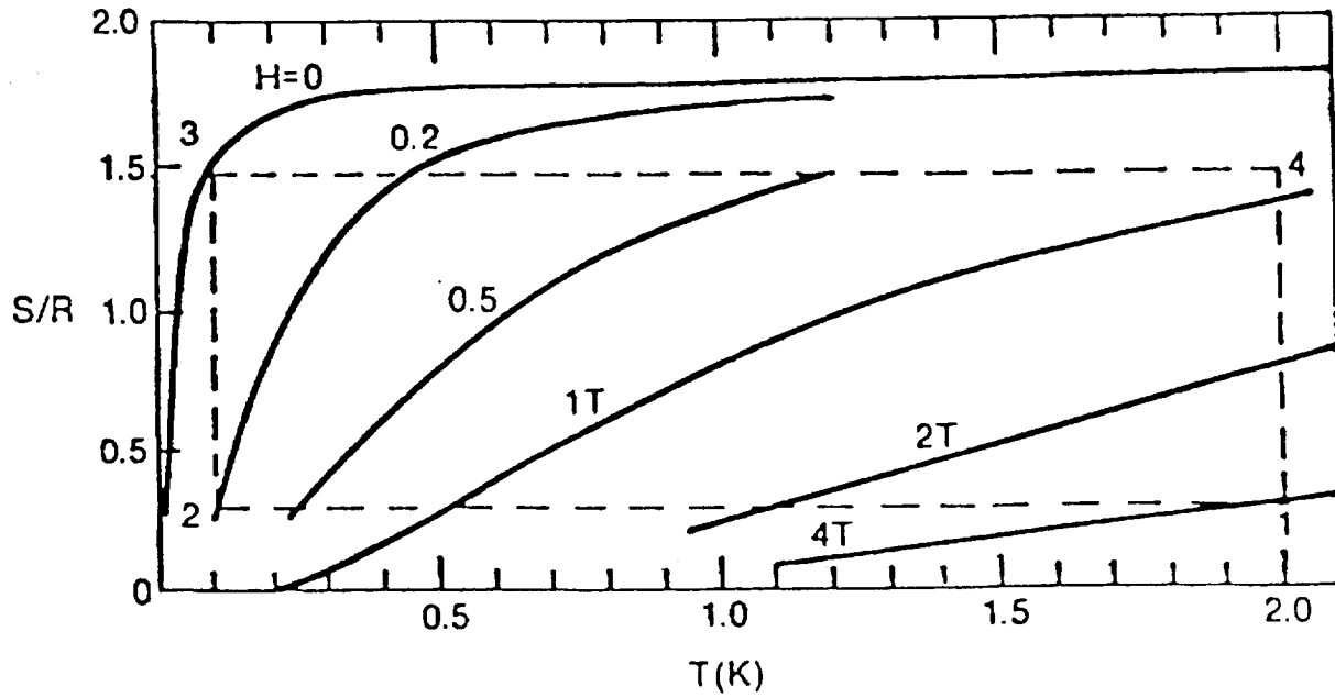
Figure 1 Entropy versus Temperature Chart for Ferric Ammonium Alum. From Castles (1980)
