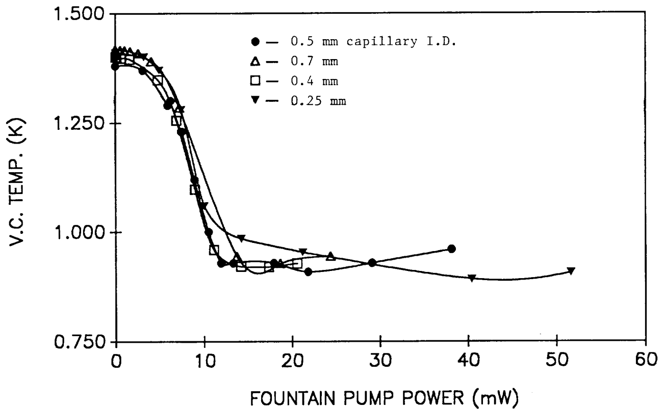
Figure 14 Vortex Cooler Temperature as a function of Fountain Pump Power for various diameter Vortex Cooler Exit Capillaries.
