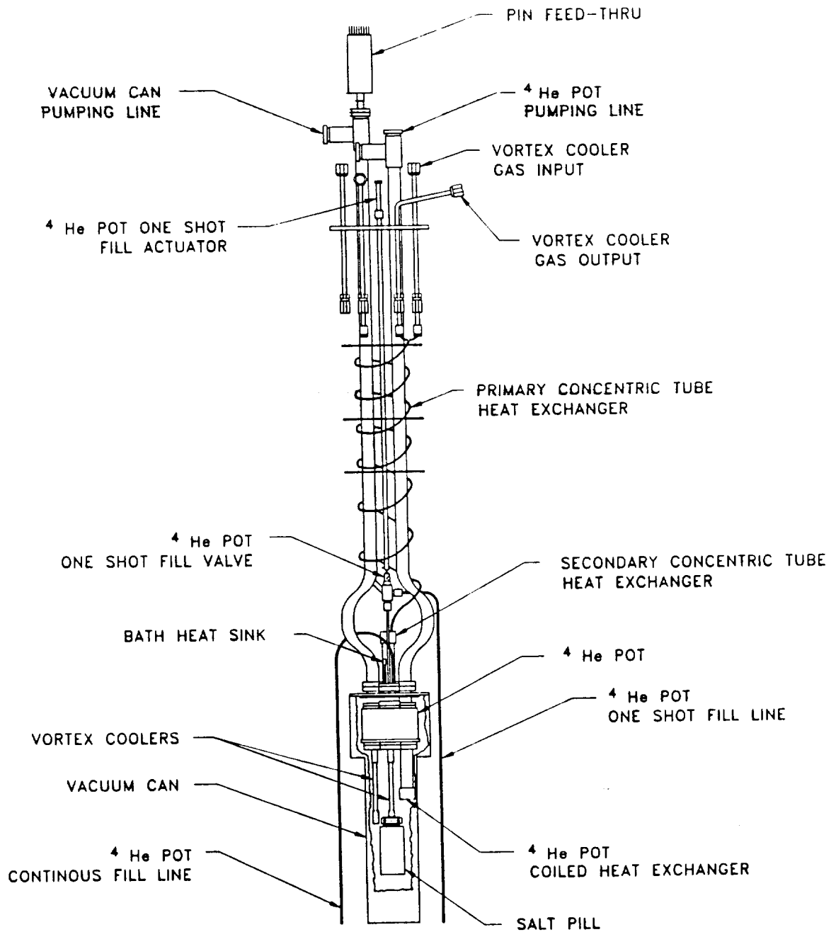
Figure 4 ADR Cryostat Configuration
