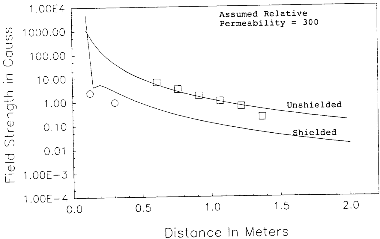
Figure 33 Effect of the Soft Iron shield on the magnetic field of the Superconducting magnet. Field strength is plotted as a function of radial distance from the center of the magnet. The upper solid line represents the field strength in the unshielded case evaluated by the ACE, Inc. Computer Program SHIELDIN . The square symbols are direct measurements of the unshielded field. The lower line gives the predicted shielded field, and the circles represent measured shielded value. The central field of the magnet is 2 Tesla.
