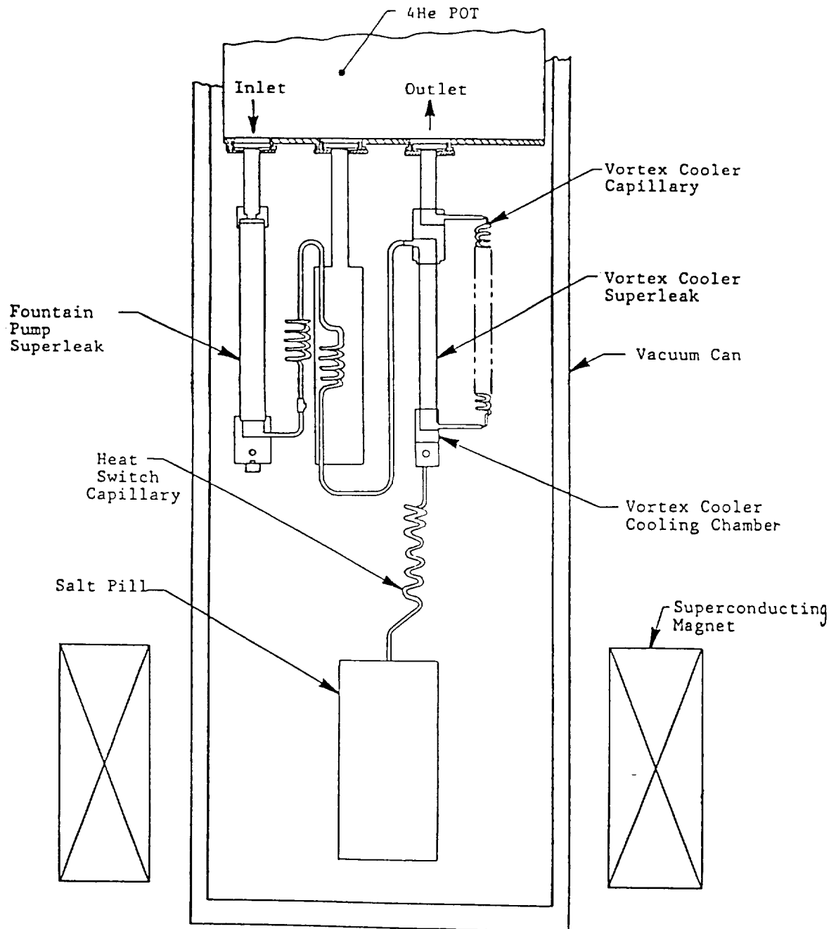
Figure 26 ADR Configuration
