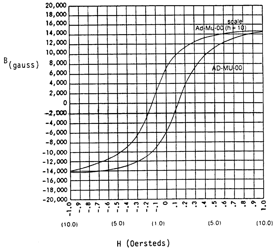
Figure 32 Magnetic flux density B vs. Magnetizing Force H for the Ad-Vance Magnetics, Inc. Alloy AD-MU-00.
