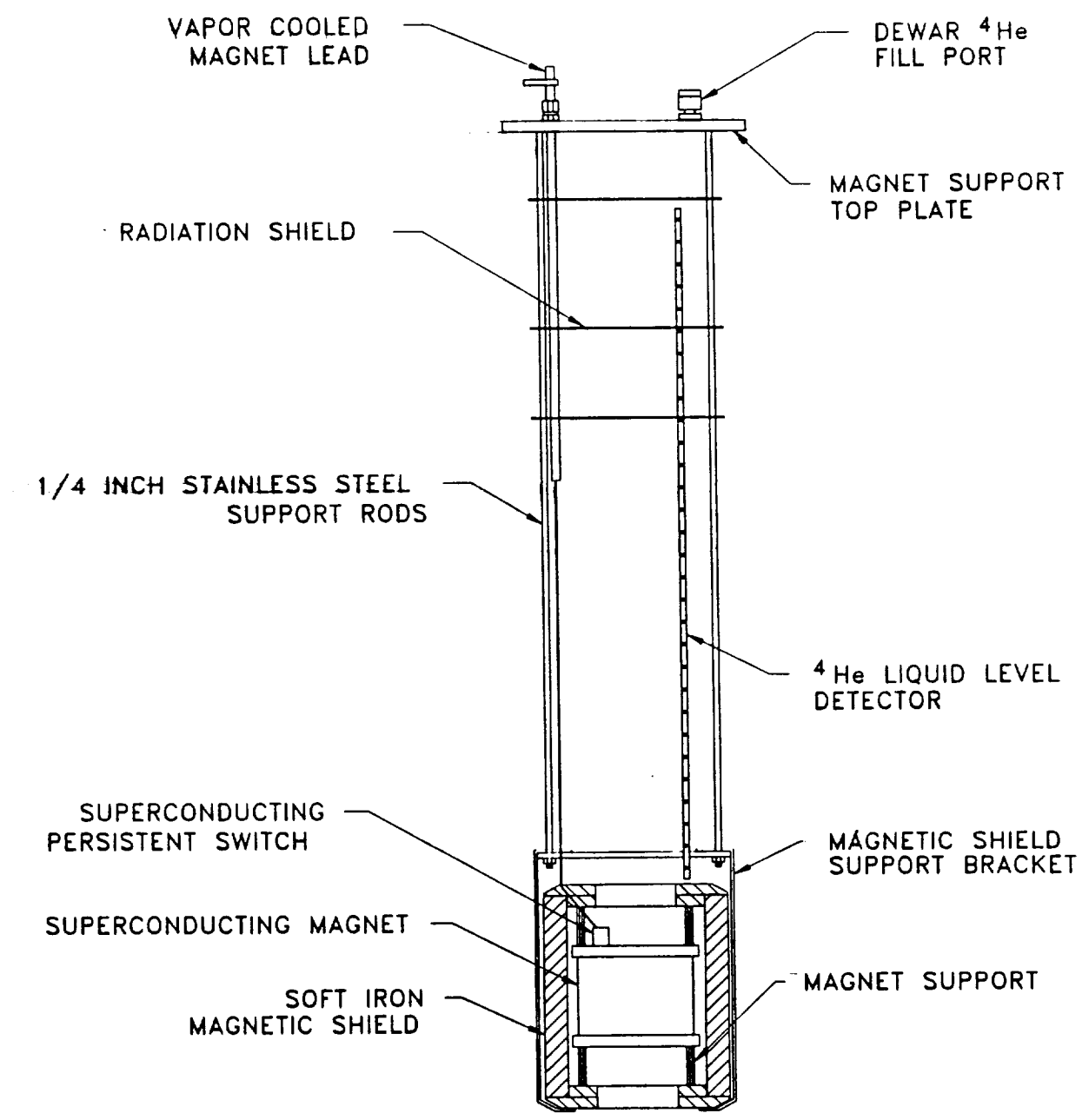
Figure 8 Superconducting Magnet Support with Soft Iron Shield in place.
