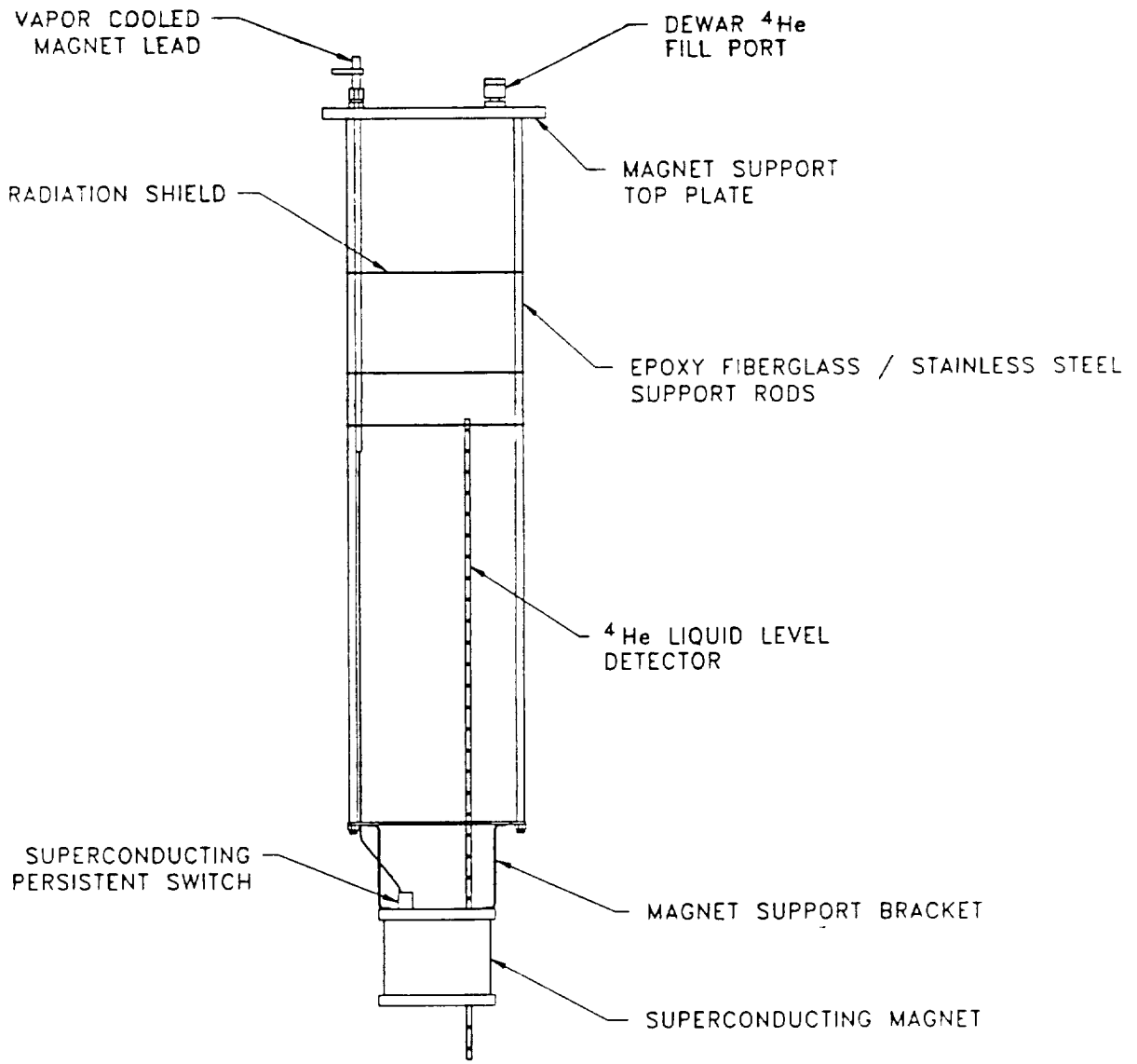
Figure 7 Superconducting Magnet Support
