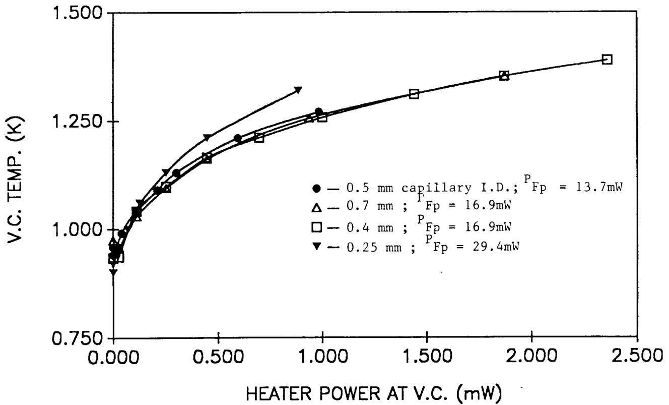
Figure 15 Vortex Cooler Temperature as a function of Heat Load applied to the Vortex Cooler for various Vortex Cooler Exit Capillary Sizes. The Fountain Pump Power P_{Fp} for each curve has been adjusted to minimize the temperature of the Vortex Cooler under zero Heat Load.
