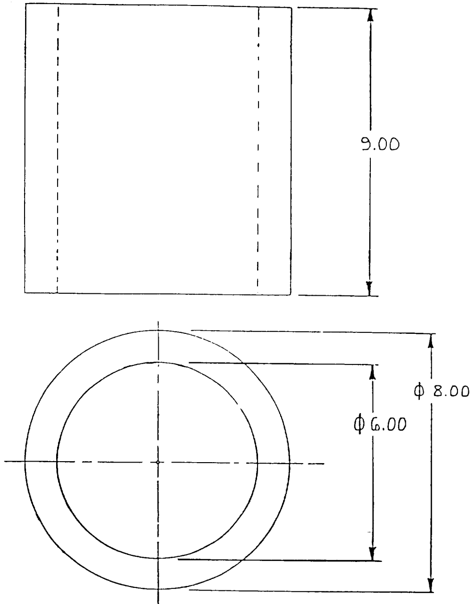
Figure 31 Side View of Magnetic Shield
