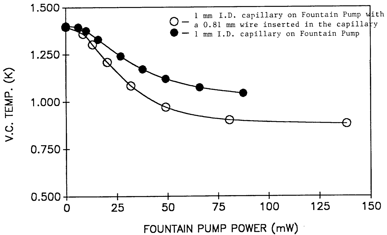
Figure 16 Vortex Cooler Temperature as a function of Fountain Pump power for two different Fountain Pump Capillary Configurations
