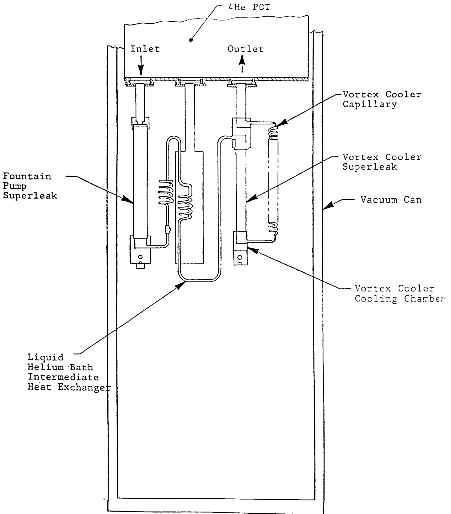
Figure 21 Fountain Pump/Vortex Cooler Configuration
