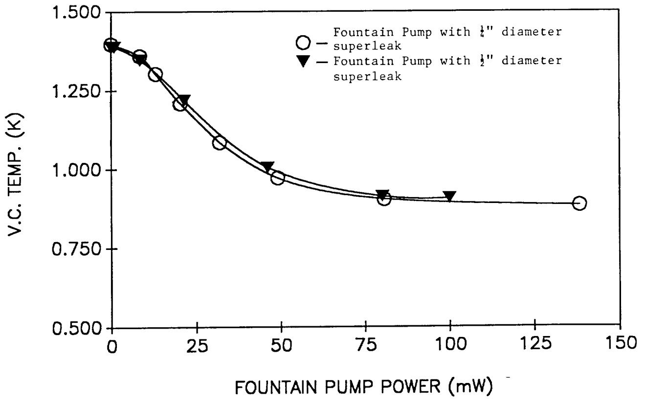
Figure 17 Vortex Cooler temperature as a function of Fountain Pump power for two different Fountain Pump Superleak diameters.
