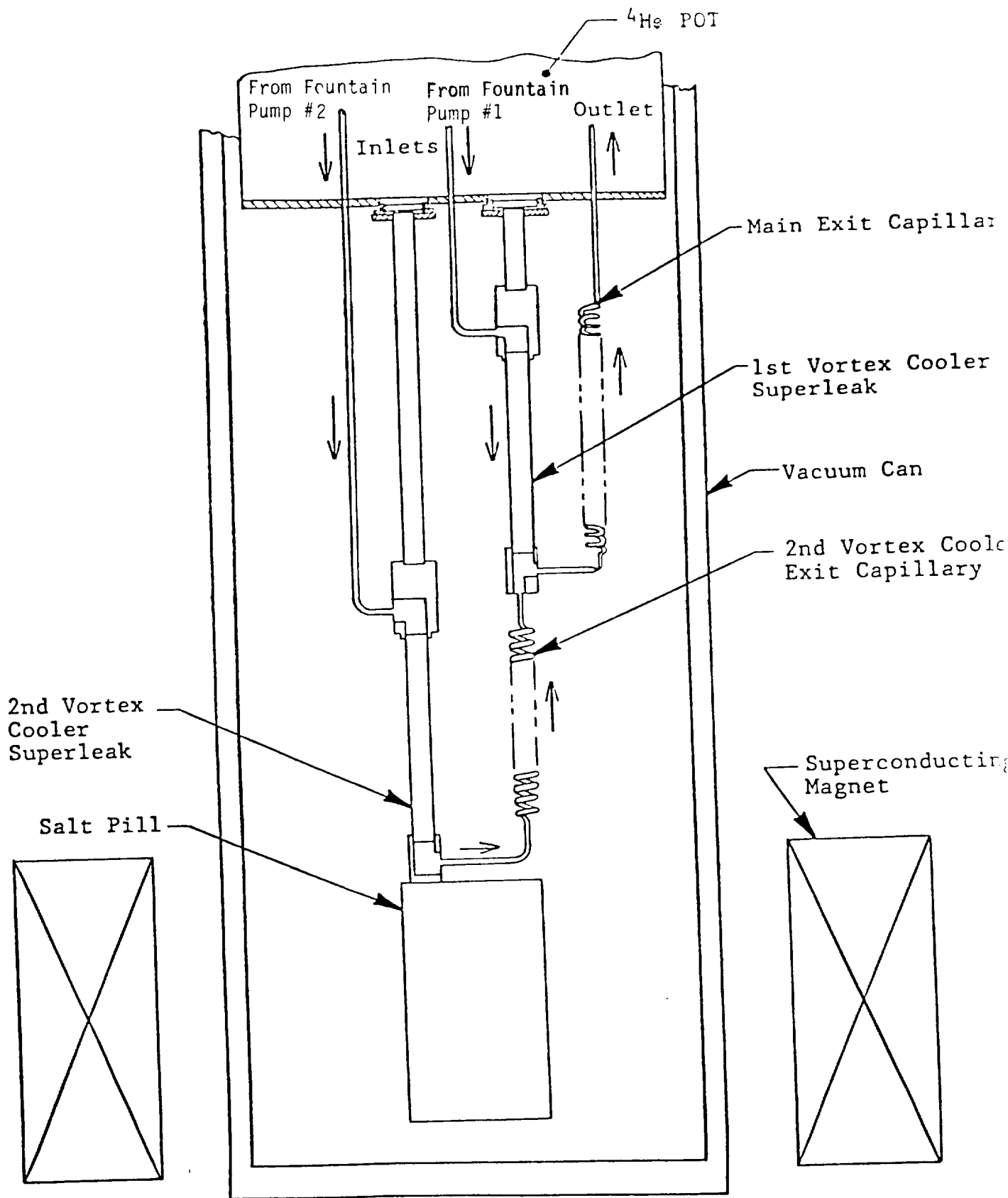
ADR Configuration Using Two Vortex Coolers
