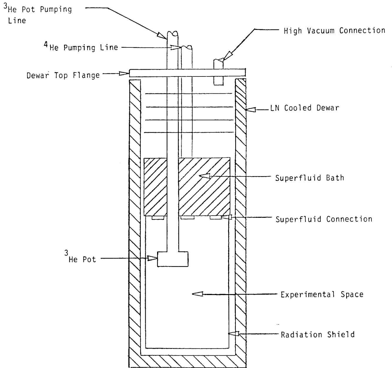
Figure 9 Auxillary Test Facility
