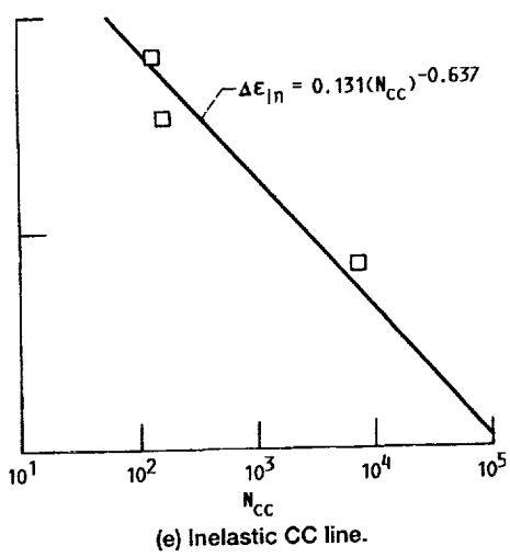
Figure 5.—Example of graphical depiction of output from program FAIL. Material, AF2-1DA; temperature, 760 °C (data from ref. 2).
