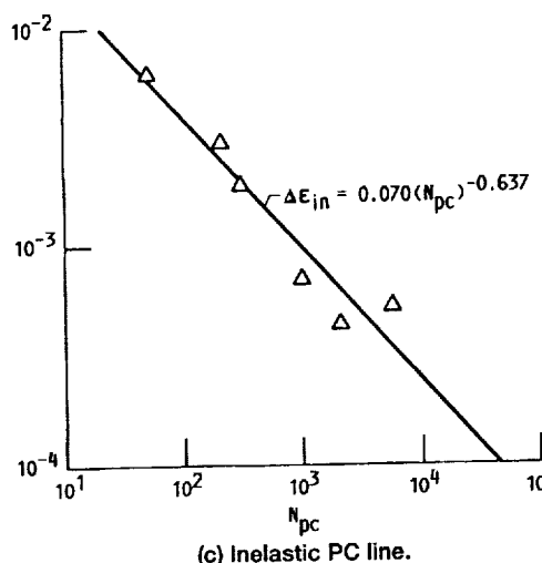
Figure 5.—Example of graphical depiction of output from program FAIL. Material, AF2-1DA; temperature, 760 °C (data from ref. 2).
