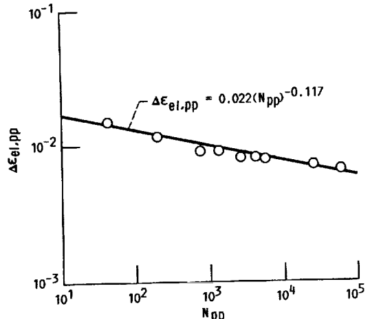
(a) Elastic PP line.
