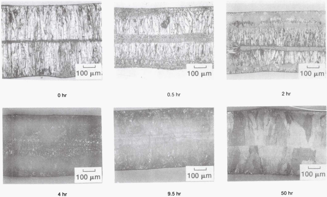
Figure 6.—Optical micrographs of polished and etched surfaces of hexacelsian \text{SrAl}_2\text{Si}_2\text{O}_8 flakes heat treated at 1100^\circ\text{C} for various times.
