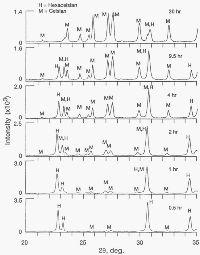
Figure 4.—Powder x-ray diffraction spectra of bulk hexacelsian \text{SrAl}_2\text{Si}_2\text{O}_8 heat treated at 1100^\circ\text{C} for various times.
