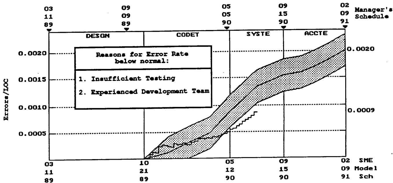
Figure 7: Analysis of 'Reported Errors/Lines of Code' for Project A
