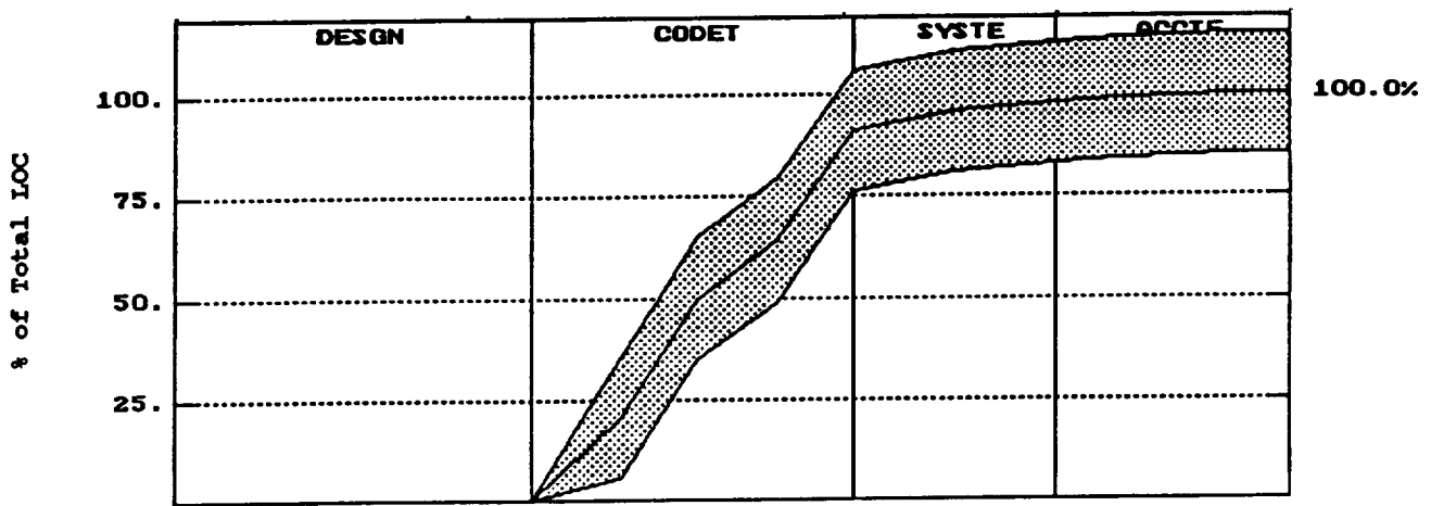
Figure 1: Model of Source Code Growth
