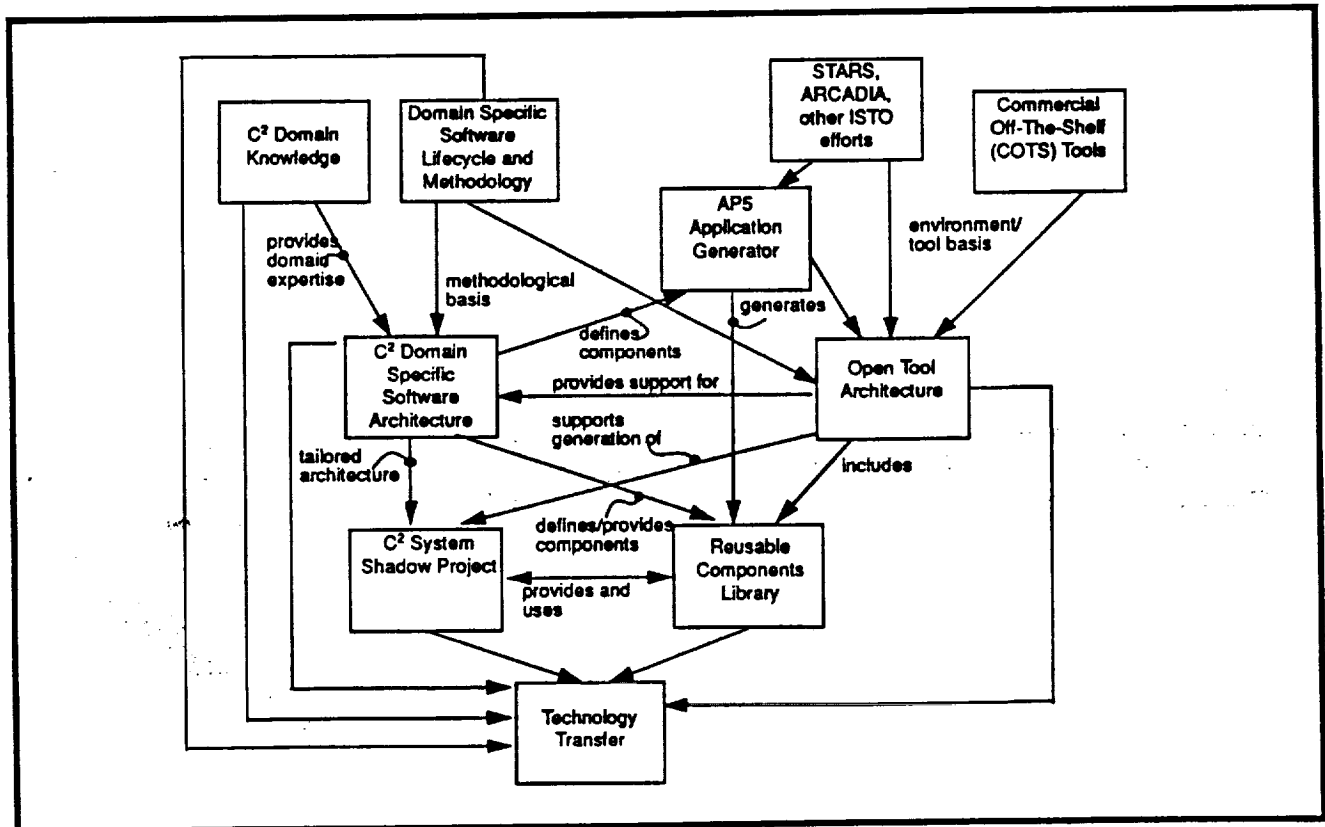
Figure 1. GTE's DSSA Approach
