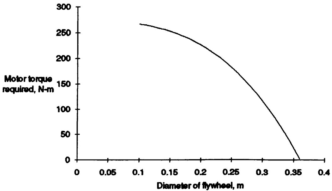
Figure F7. Motor torque as a function of flywheel diameter.
