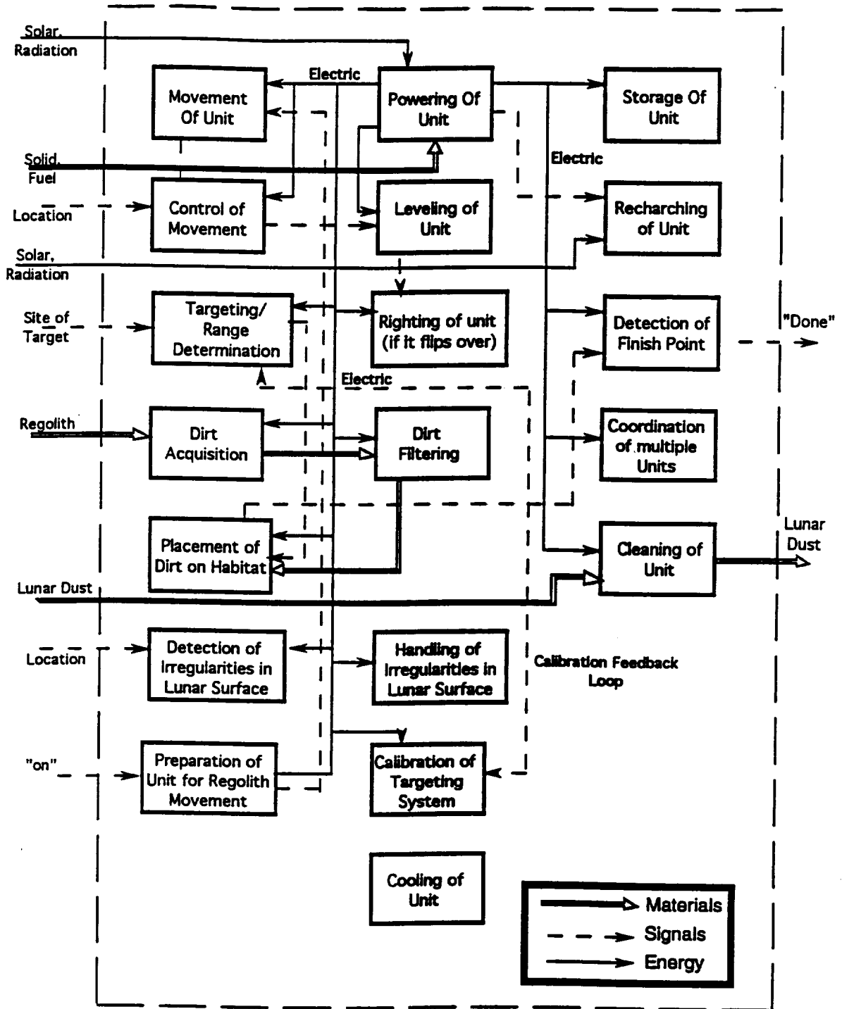
Figure A1. Function Structure of Lunar Device.
