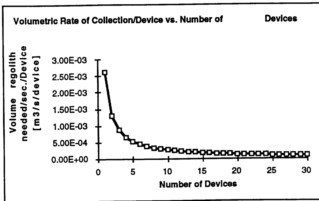
Figure 32. Volumetric rate of collection per unit vs. number of units
