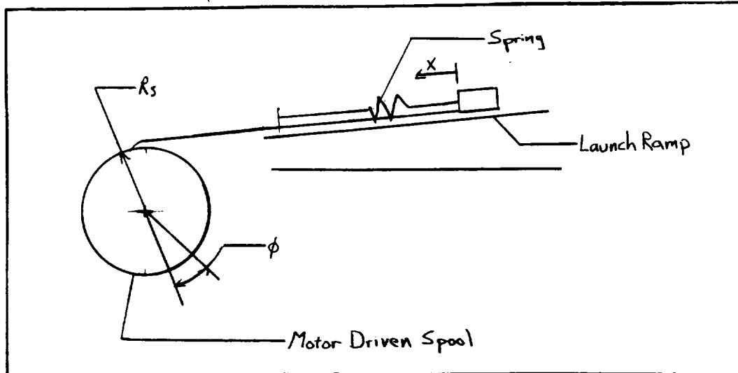
Figure F2. Spring motor arrangement.
