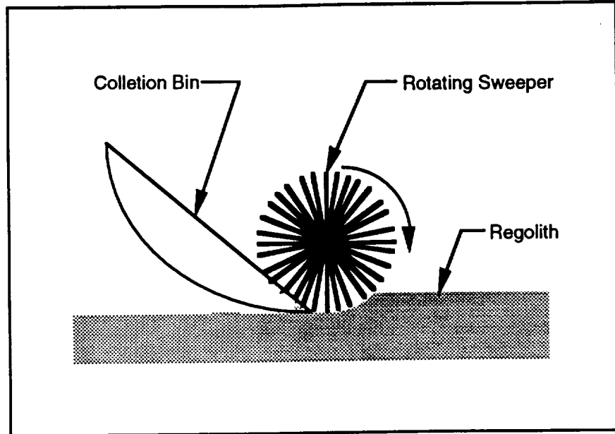
Figure 14. Sweeping mechanism.
