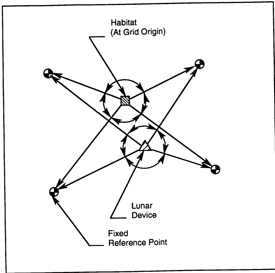
Figure 19. Angle measurements for multiple point resection calculations
