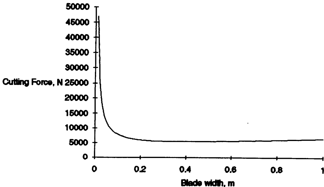
Figure J6. Cutting force as a function of blade width.
