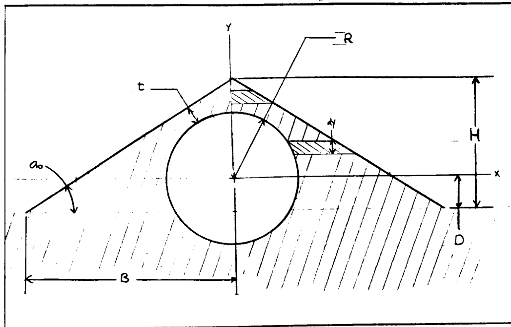
Figure G1. Variable definition for volume of regolith
