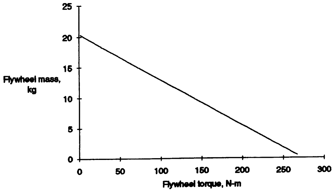
Figure F6. Flywheel mass as a function of the torque required.
