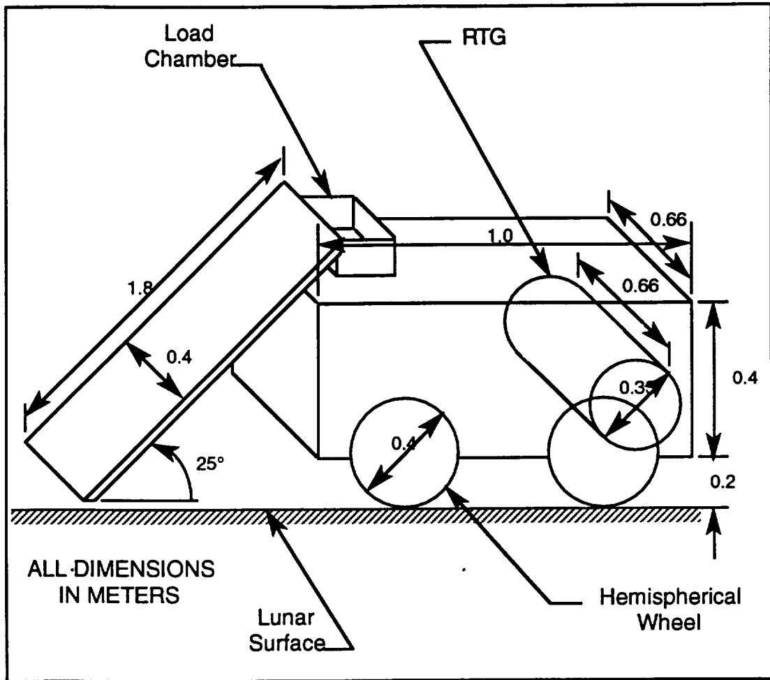
Figure 31. Scaled configuration for computer simulation
