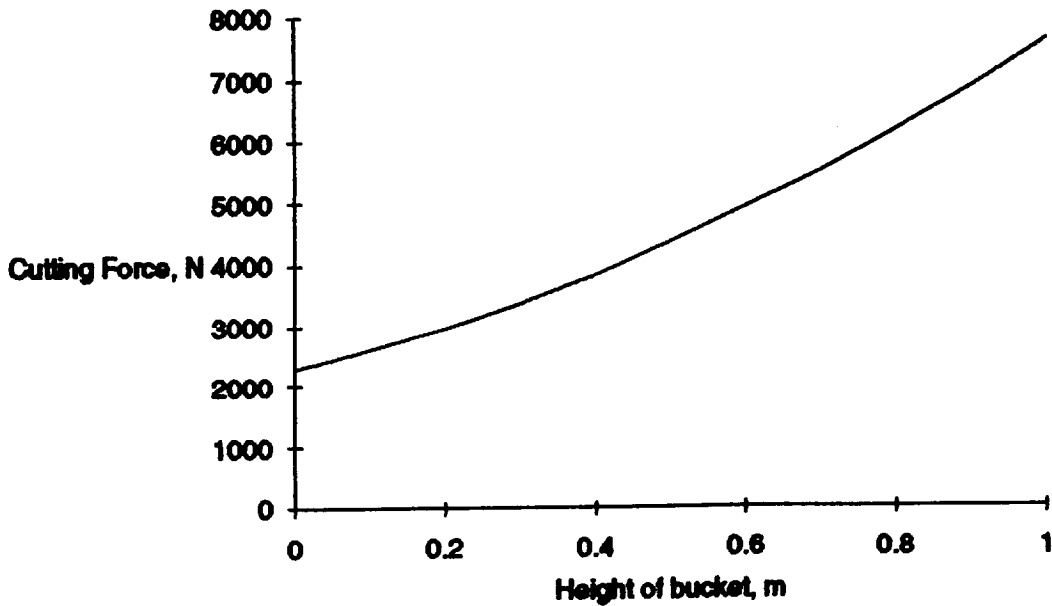
Figure J8. Cutting force as a function of bucket height.
