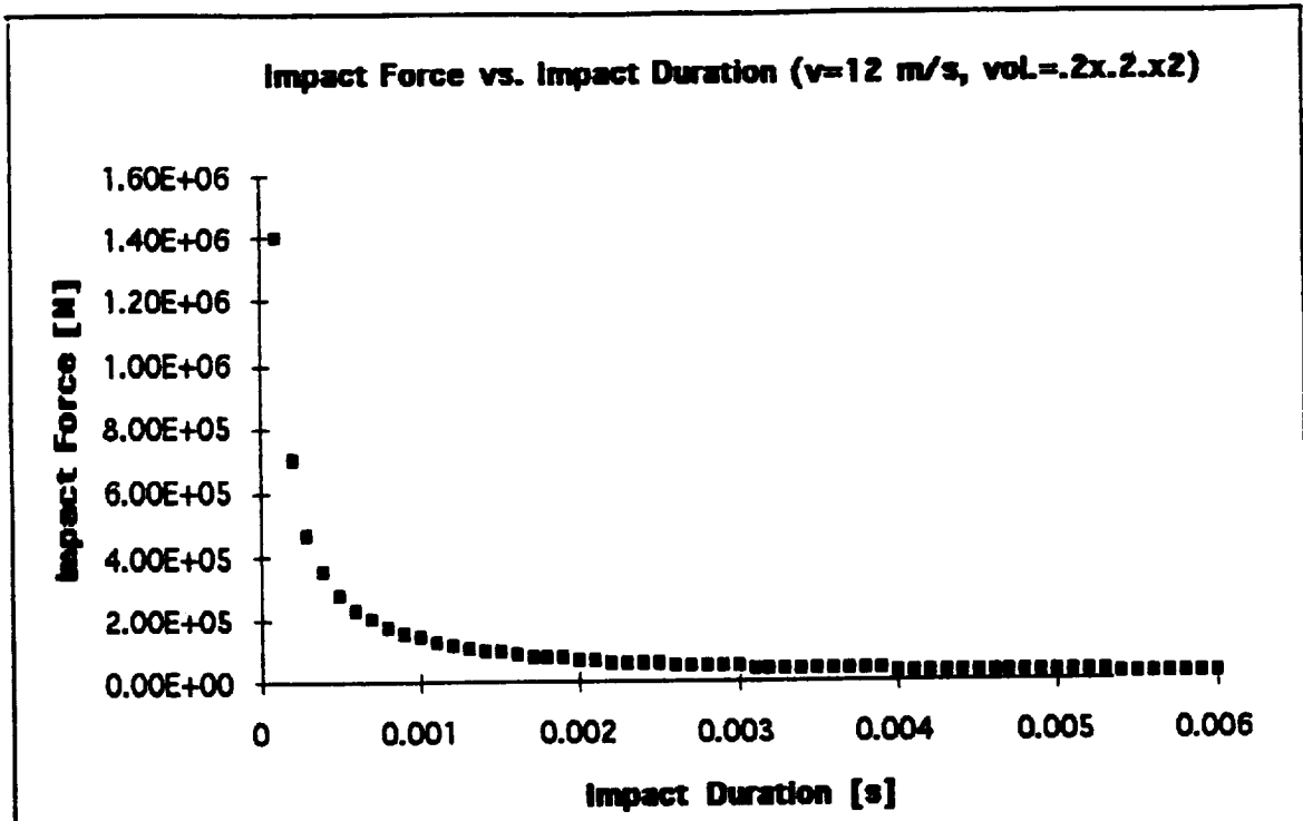
Figure B1. Impact force vs. Impact duration (Equation B1)
