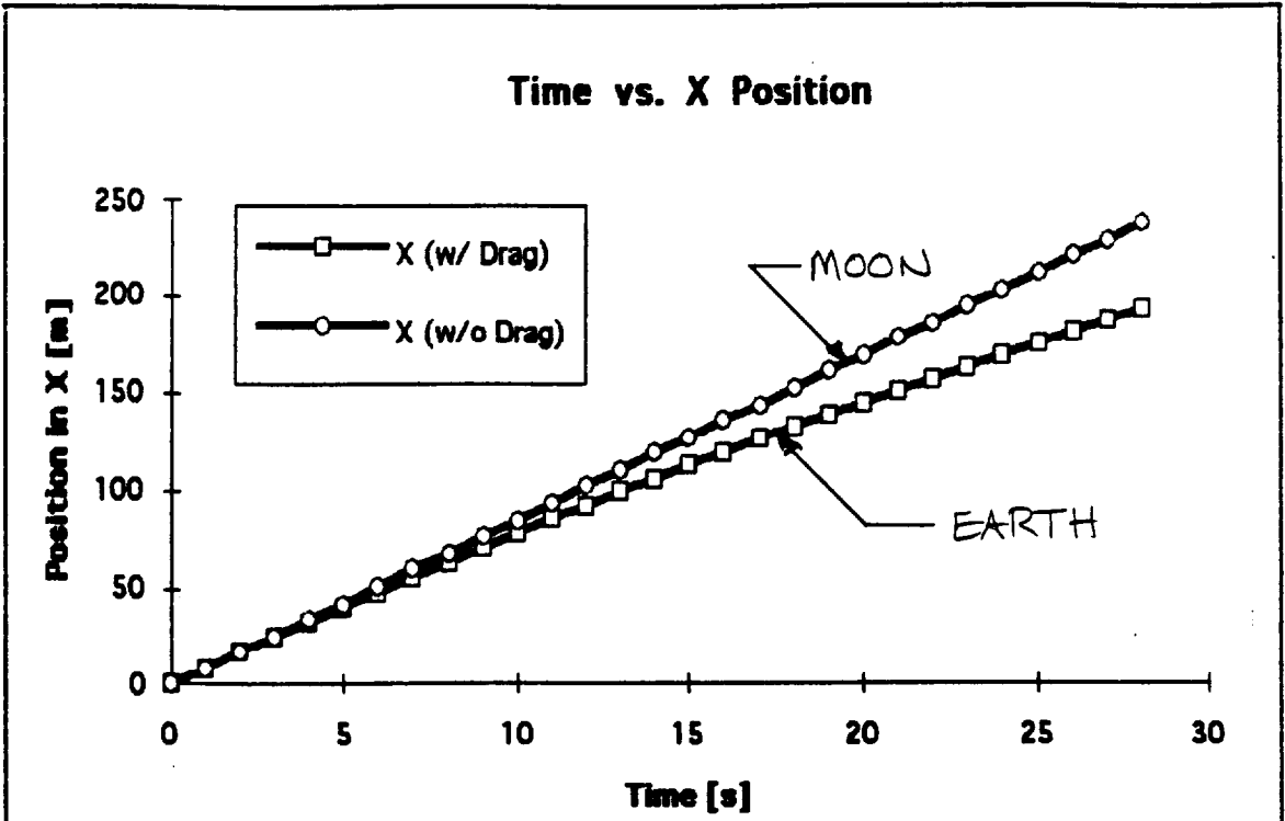
FIGURE C1. Horizontal position vs time (plot of Equation C2).
