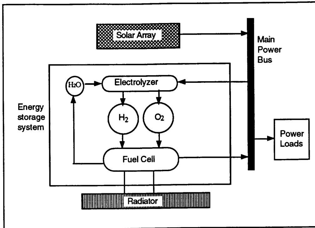
Figure 23. Regenerative fuel cell process description [34].
