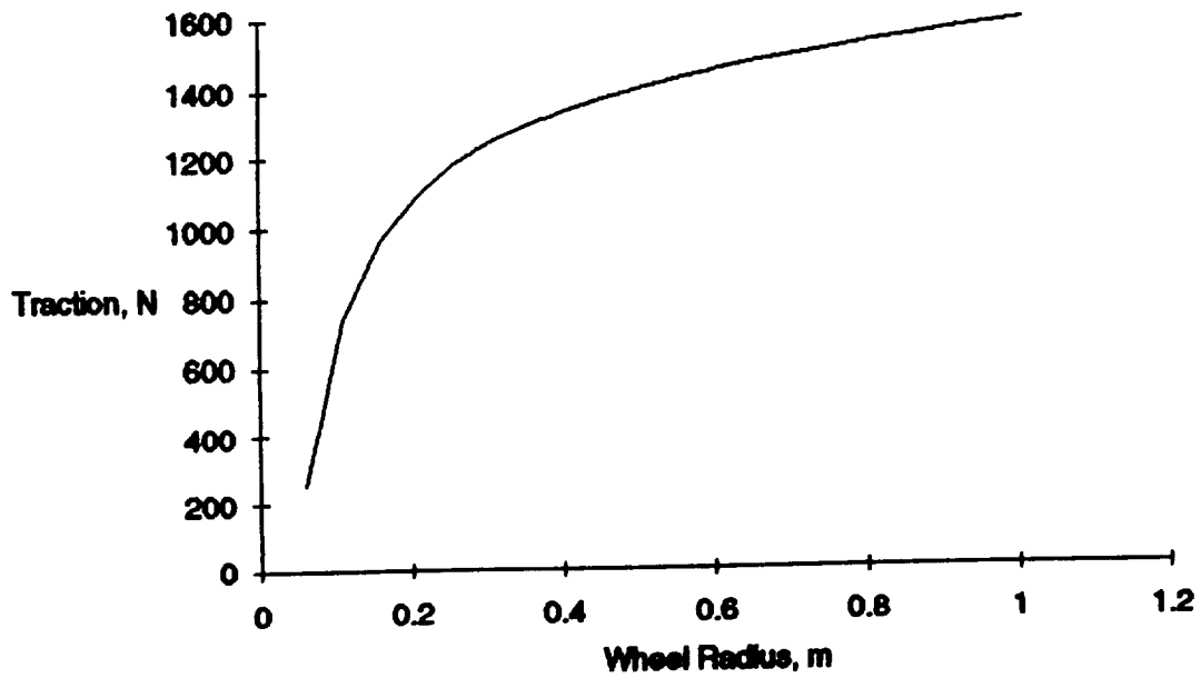
Figure J3. Traction as a function of wheel radius.
