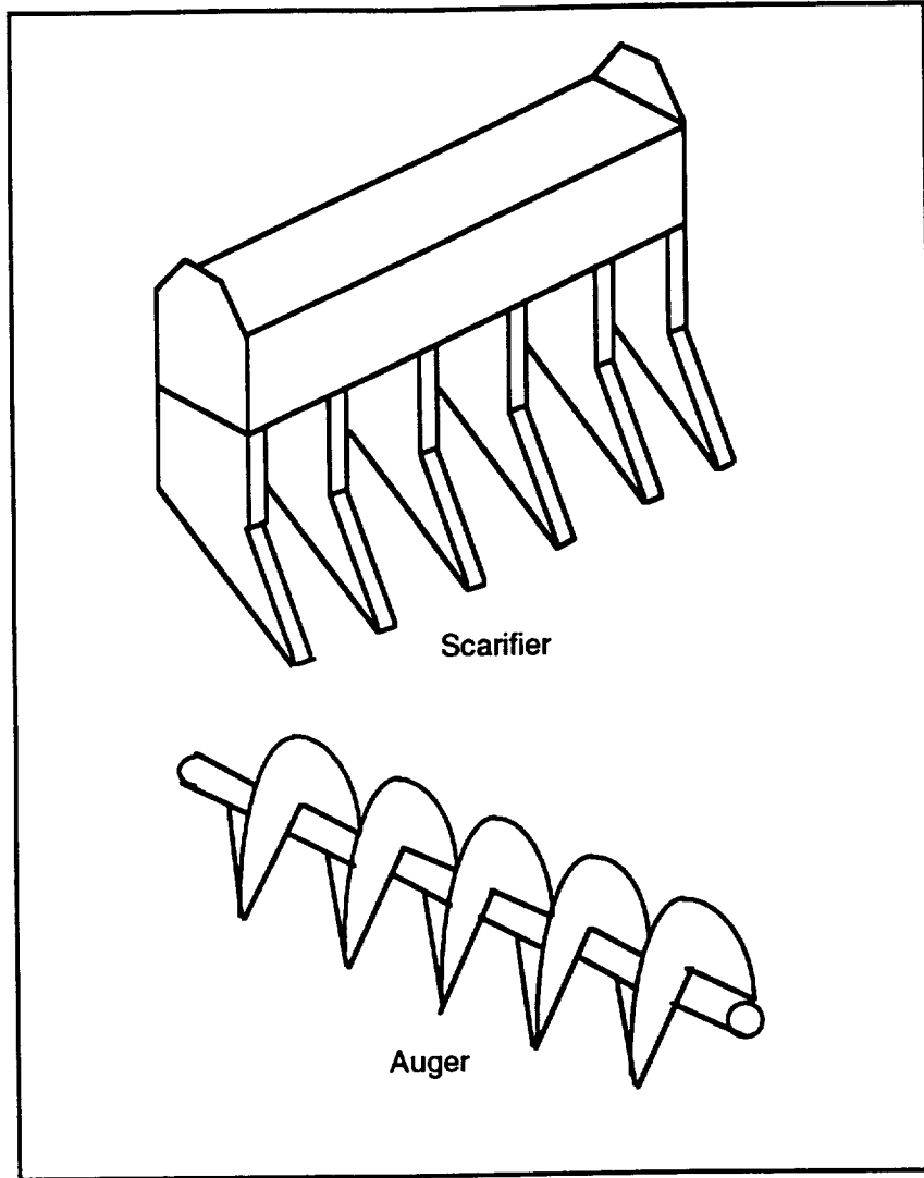
Figure 16. Scarifier and auger mechanisms.
