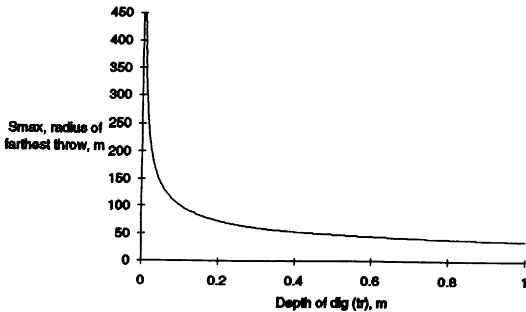
Figure D3. Radius of area that must be cleared as a function of Depth of dig.
