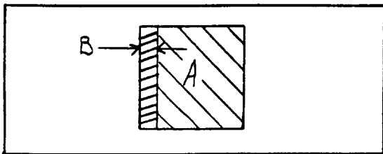
Figure J5. Width of cut, B , on Area, A .
