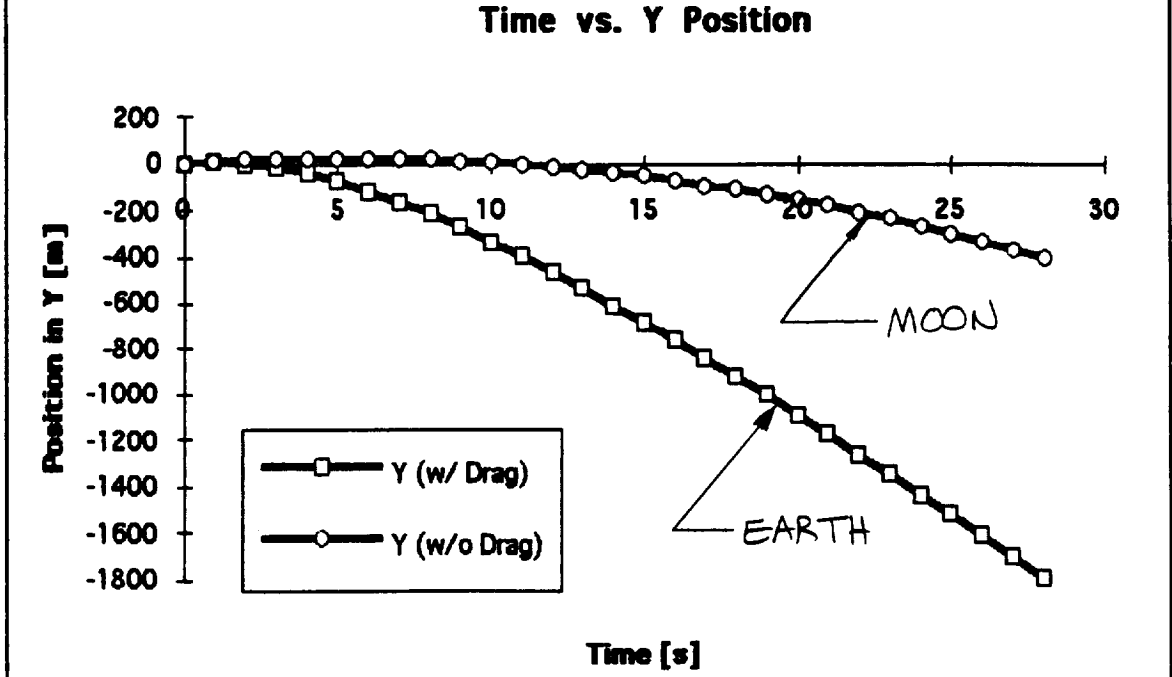
FIGURE C2. Vertical position vs. time (Equation C3)
