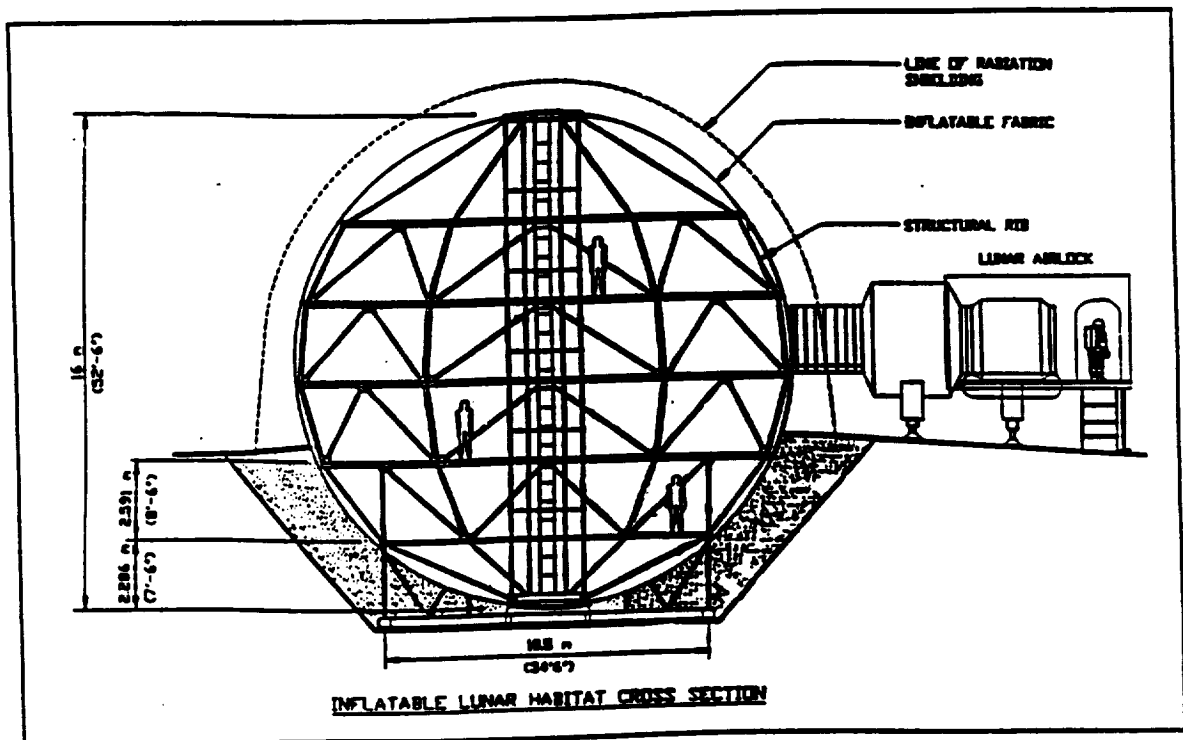
Figure 2. Cross-sectional view of proposed habitat. (Modified from [7])
