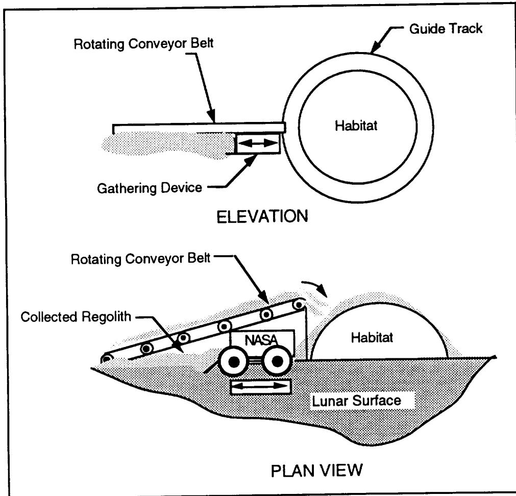
Figure 4. Circling conveyor belt mechanism.
