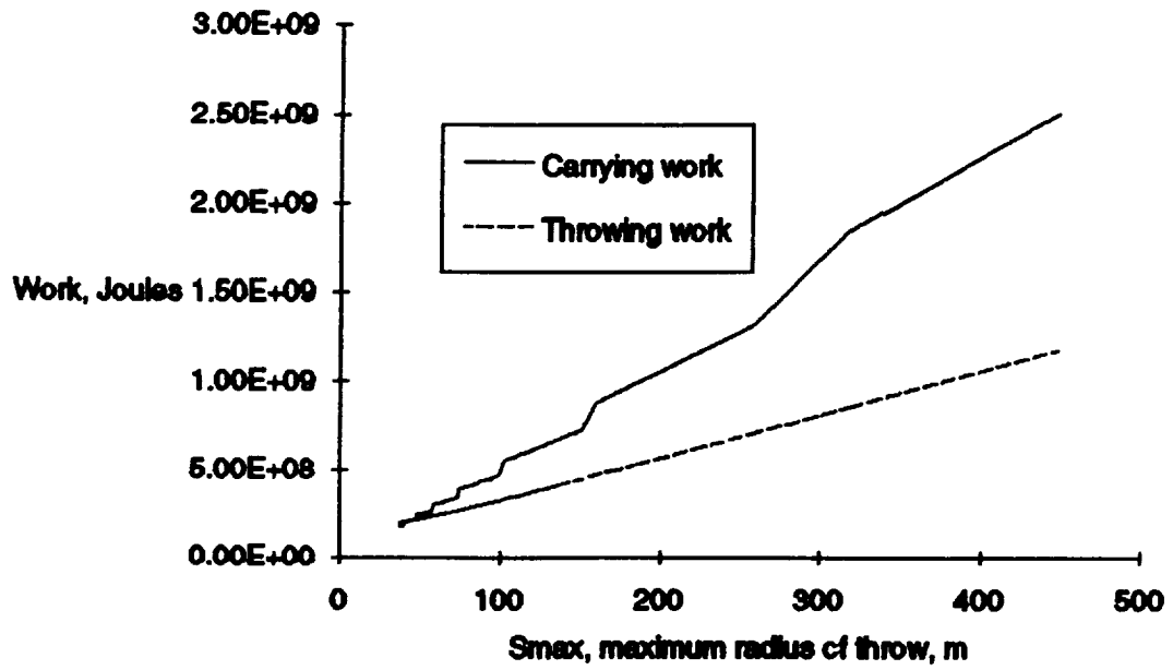
Figure D5 Work to move regolith as a function of surface area cleared
