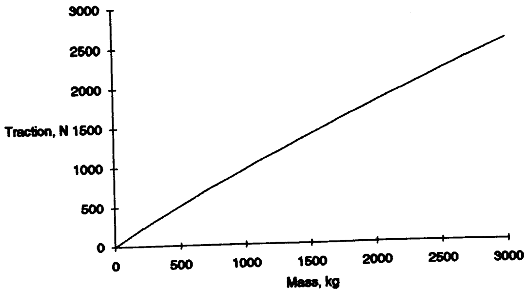
Figure J4. Traction as a function of device mass.
