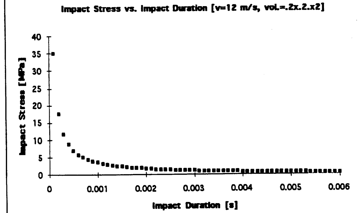
Figure B2. Impact Stress vs. Impact duration (Equation B2)
