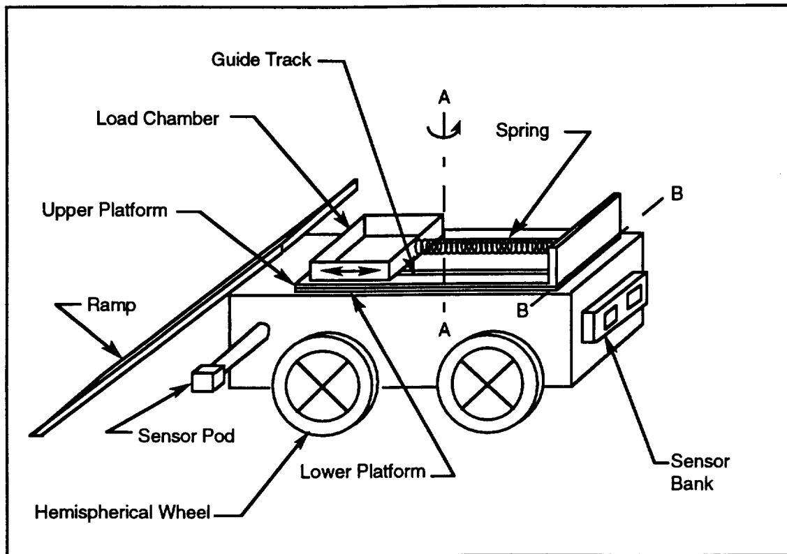
Figure 28. Overall Design Configuration #1.
