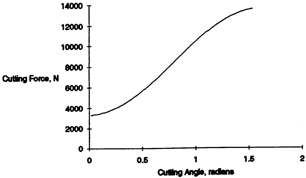
Figure J7. Cutting force as a function of cutting angle.
