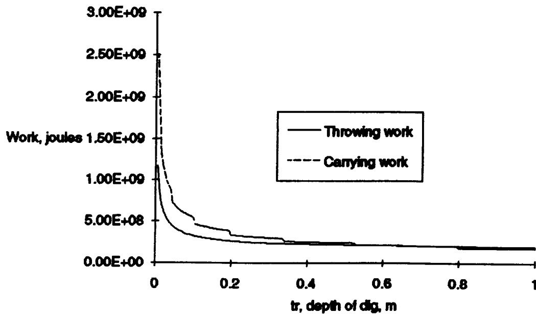
Figure D4. Work to move the regolith vs. depth of dig
