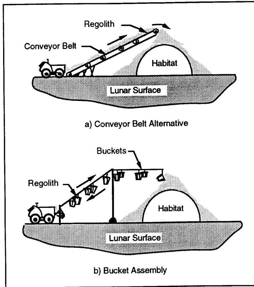
Figure 3. Conveyor belt and bucket assemblies.
