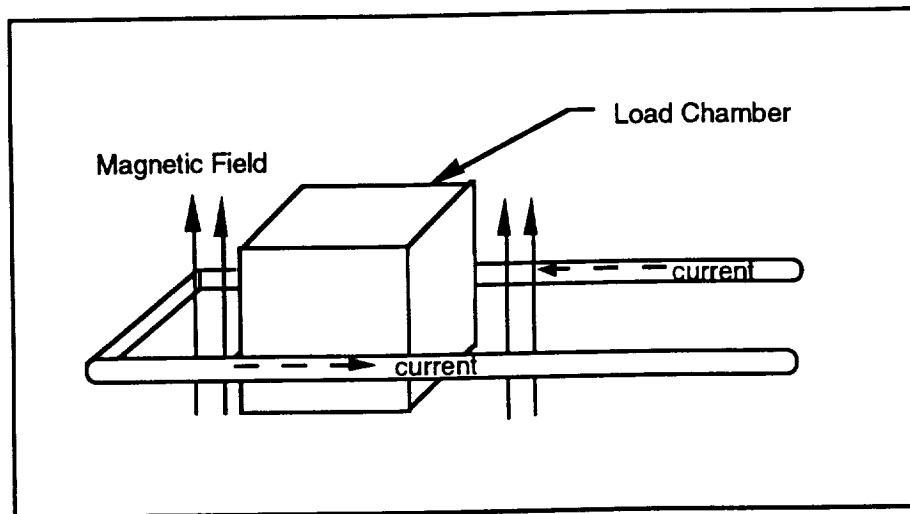
Figure 11. Railgun throwing mechanism
