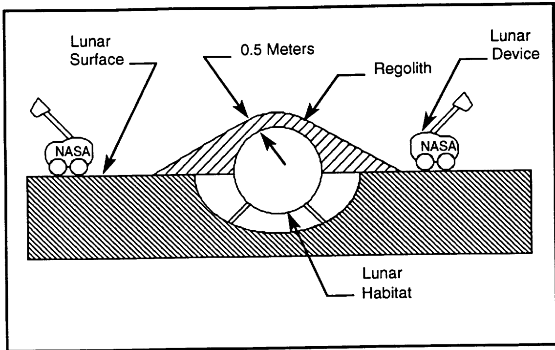
Figure 1. Schematic of Lunar Habitat.
