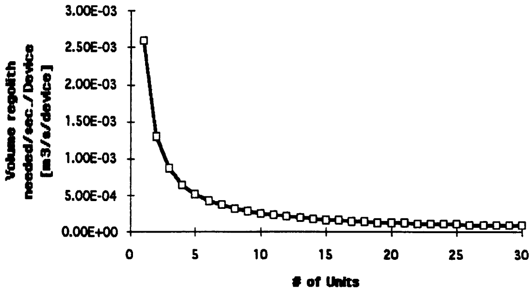
Volumetric Rate of Collection/Device vs. # of Devices
