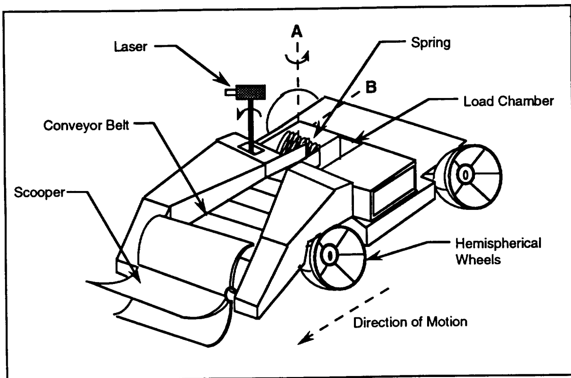
Figure 30. Overall Design Configuration #3.
