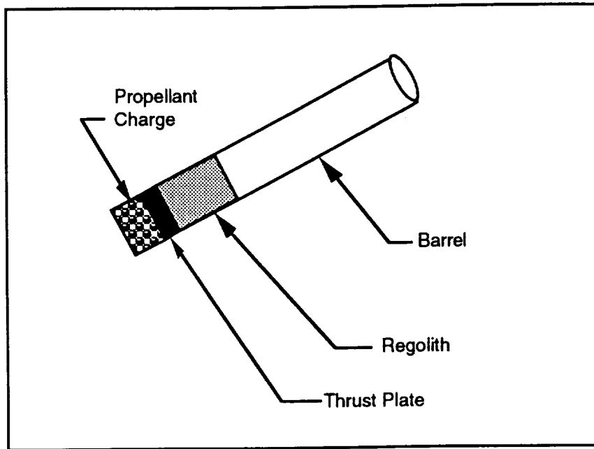
Figure 9. Impact mechanism.
