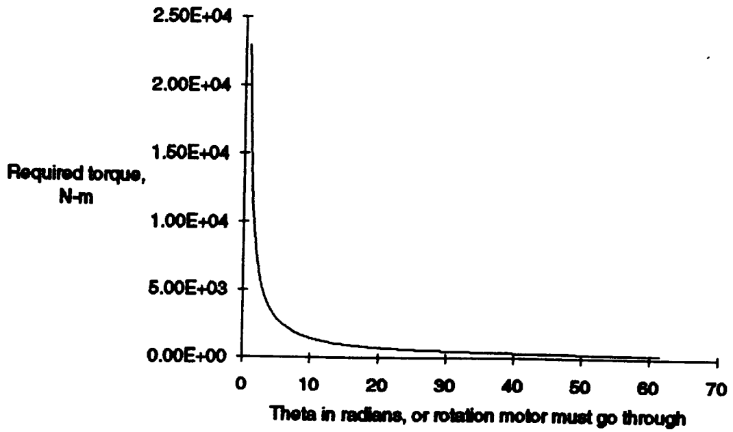
Figure F3. Required torque to compress spring as a function of the number of rotations it undergoes.
