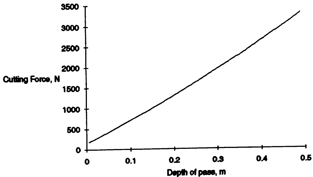
Figure J9. Cutting force versus depth of cut
