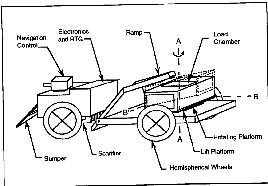
Figure 29. Overall Design Configuration #2.
