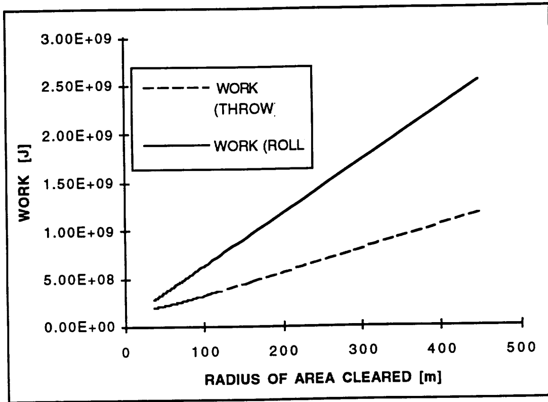
Figure 27. Work comparison between throwing and carrying
