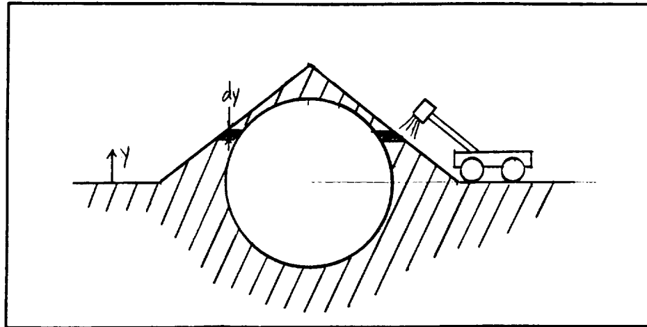
Figure D2. Method for positioning regolith on the habitat using a front loader
