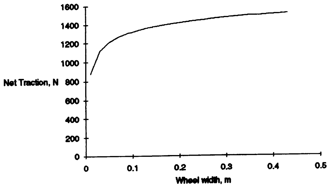
Figure J2. Net traction as function of wheel width.
