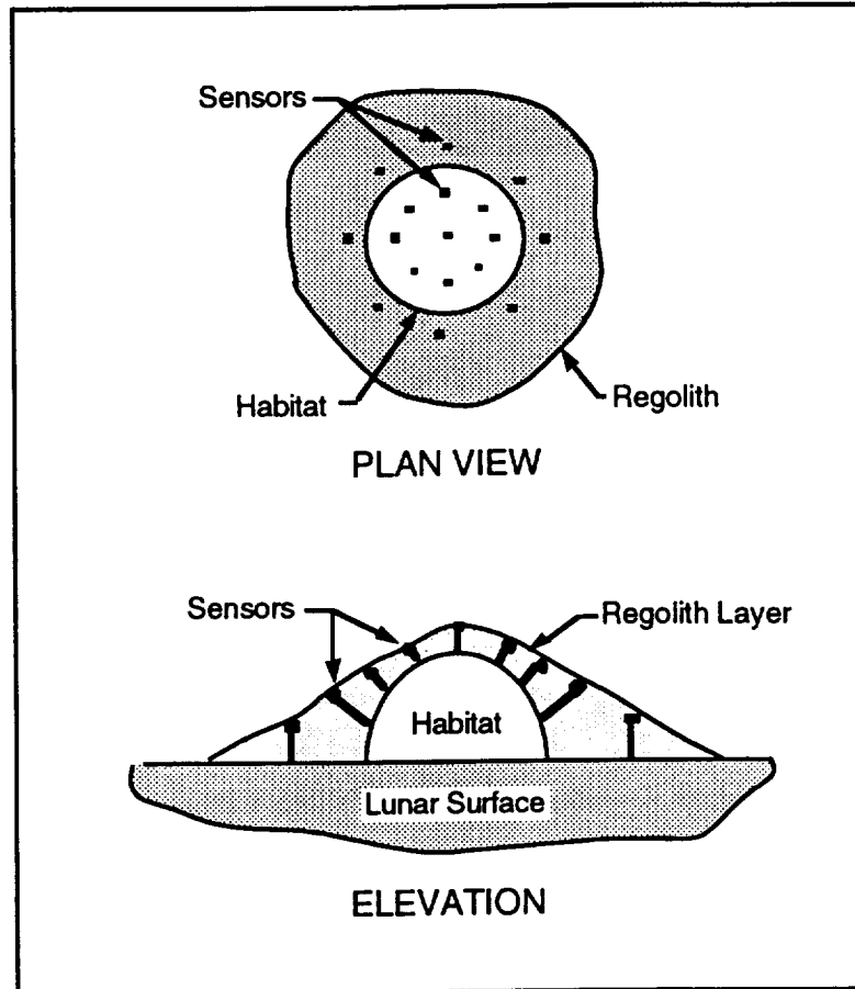
Figure 22. Configuration of sensors on poles.
