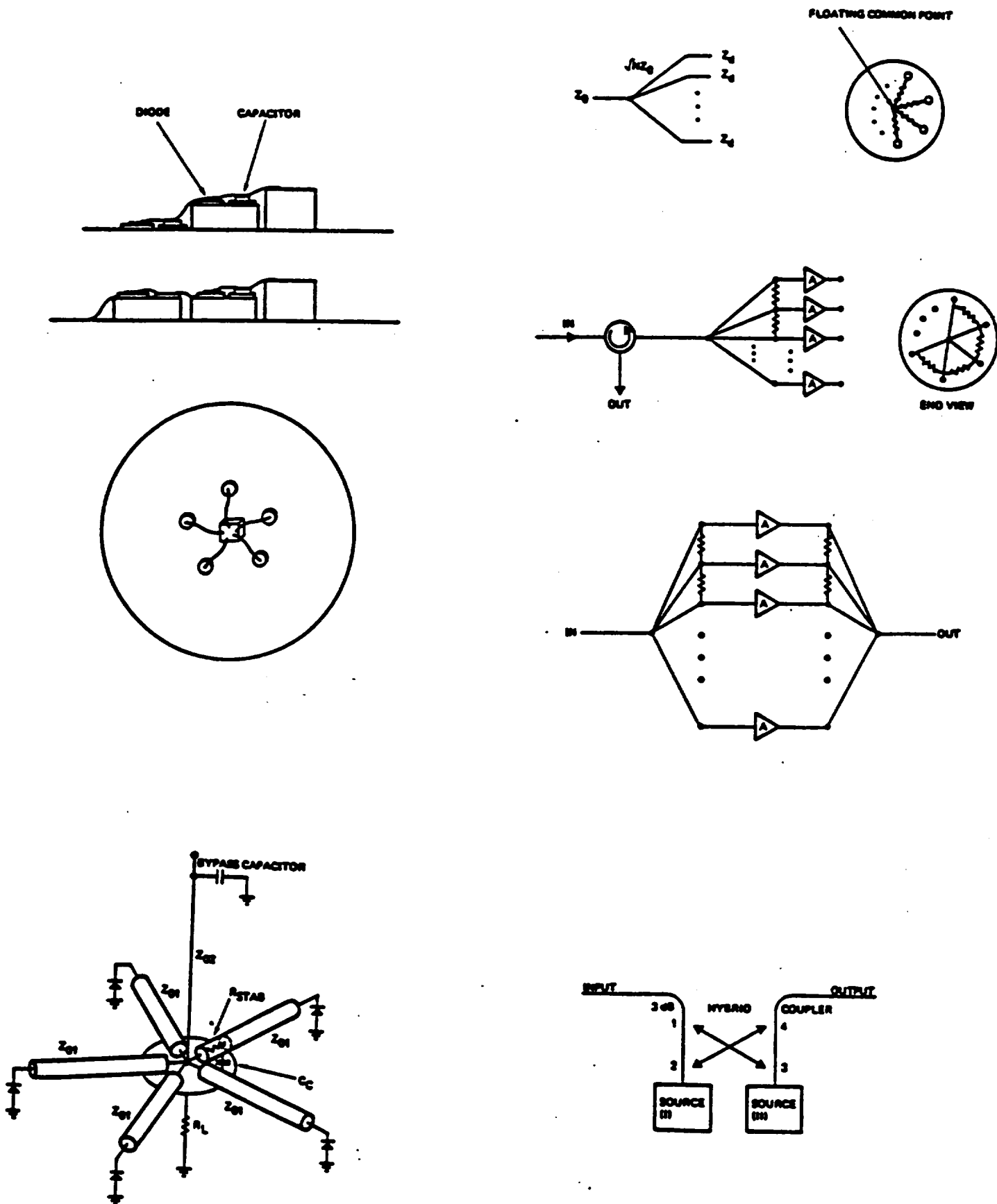
Figure 2.2 Various schemes for power combining using Gunn diodes (Ref.1)
