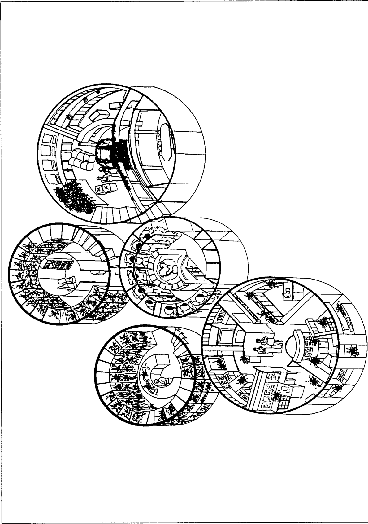
Figure 4.4.1-11. Axonometric drawing of main floor (entry level) of Pax, illustrating the embracing entry (center) and separation of laboratories from crew support facility (lower-left to upper right). The greenhouse modules are on the upper left.
