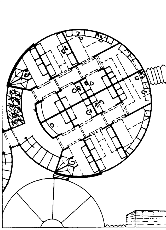
Figure 4.5.3.5-1. Upper level floor plan of the crew support module—the crew quarters and PHFs.
