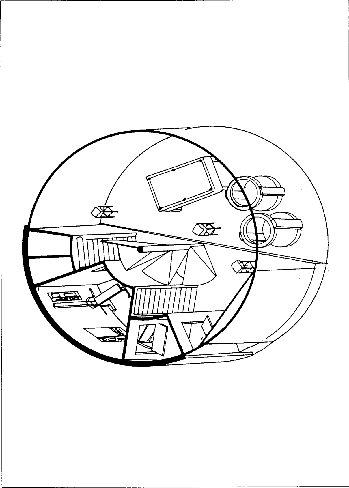
Figure 4.4.1-13. Axonometric of the lower level of the entry module (one level down from the entry level of Figure 4.4.1-11). Contained within is the active group recreation area and exercise facility.
