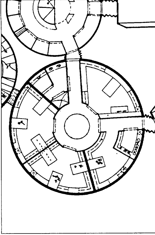
Figure 4.5.2.2-1. Floor plan of the main level of the laboratory module showing (from lower center, clock-wise) the general, chemistry, and biology labs.
