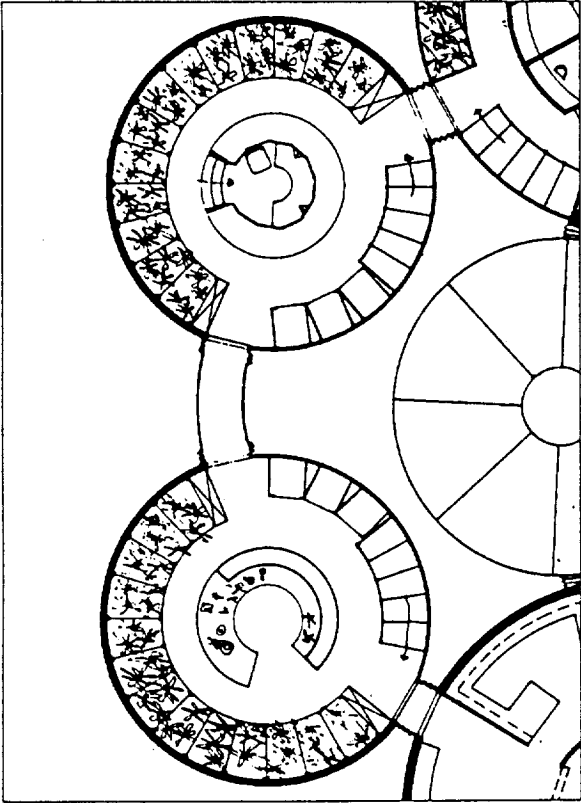
Figure 4.5.4-1. Floor plan of the upper level of the two greenhouse modules. Greenhouse accessibility is from the primary circulation space of the crew support module (upper level) and the botanical labs of the laboratory module (upper level).
