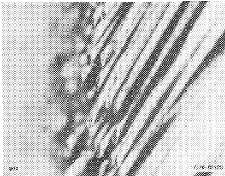
Figure 16.—Brush bristle tip wear patterns (test 2).
