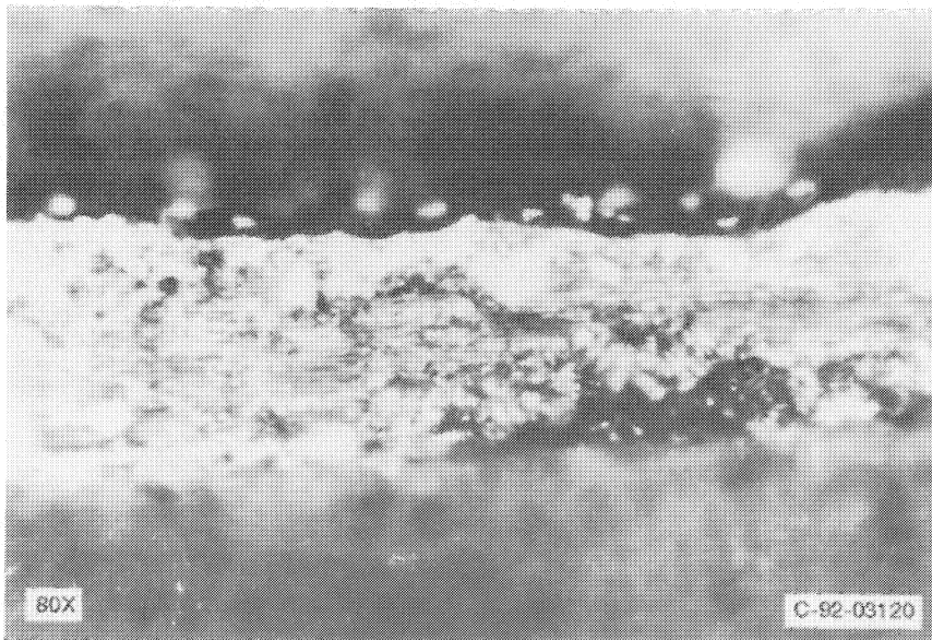
Figure 18.—Rotor trailing edge (test 3).
