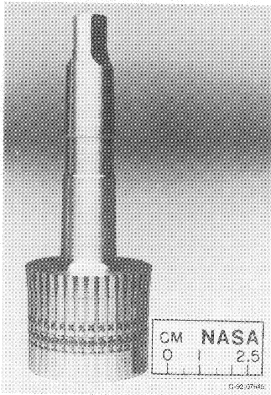
Figure 2.—Geometry of tapered, 40-tooth rotor.
