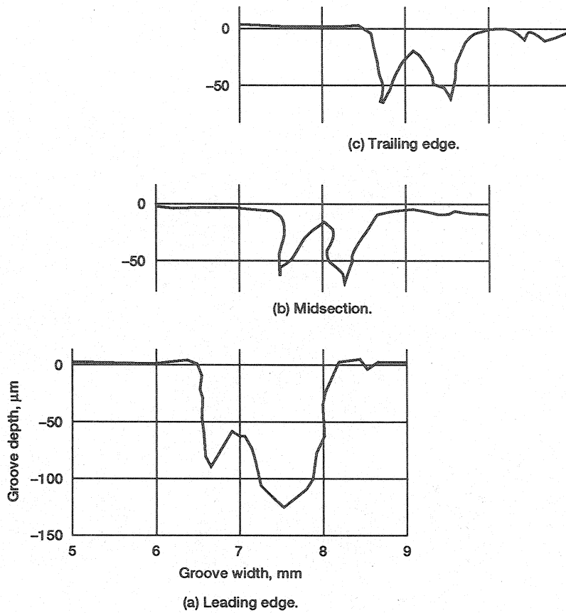
Figure 8.—Profilometer traces for 40-tooth rotor (test 2).
