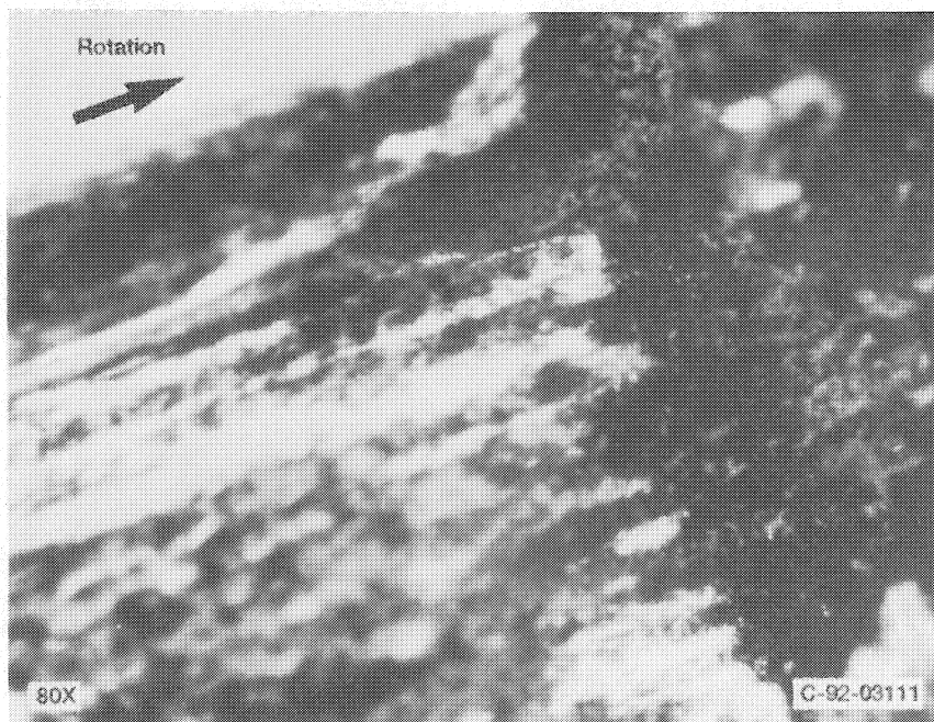
Figure 11.—Rotor leading-edge debris formation (test 2).
