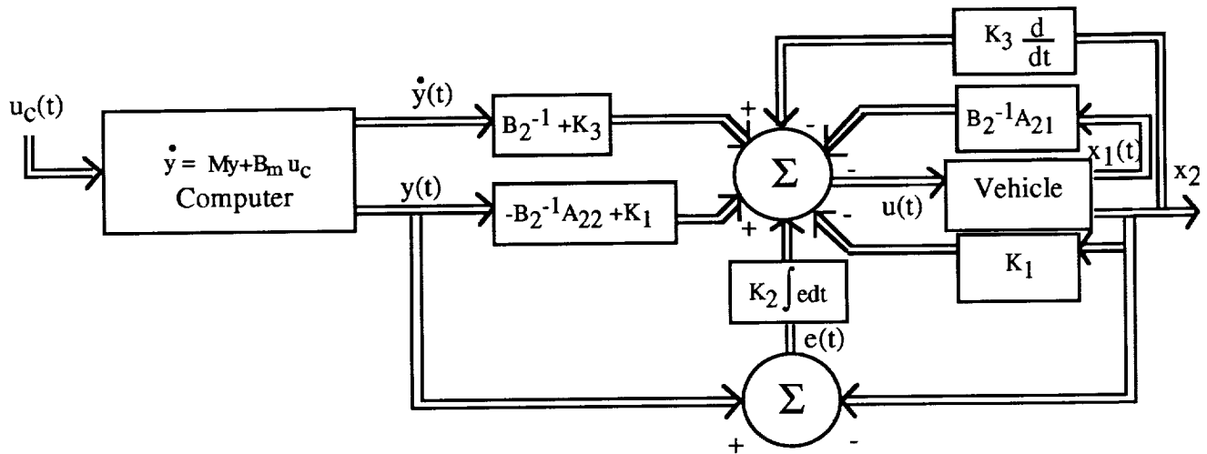
Figure 7 Robust Model Following Architecture
