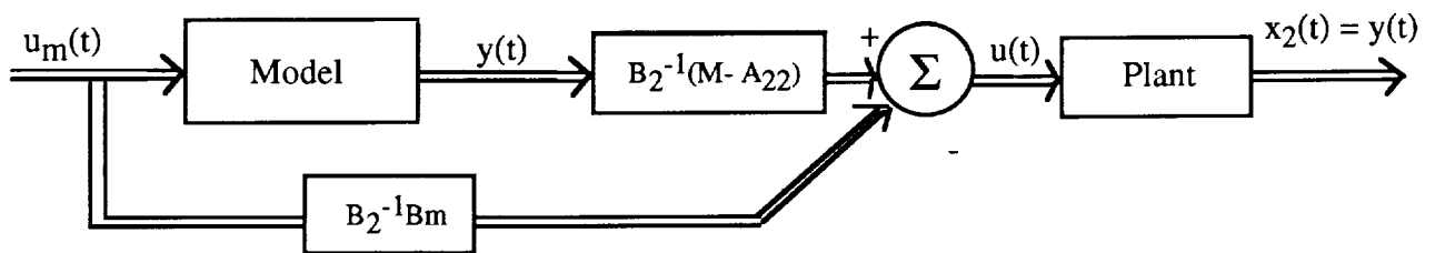
Figure 4 Alternate "Explicit" Model Following Architecture
