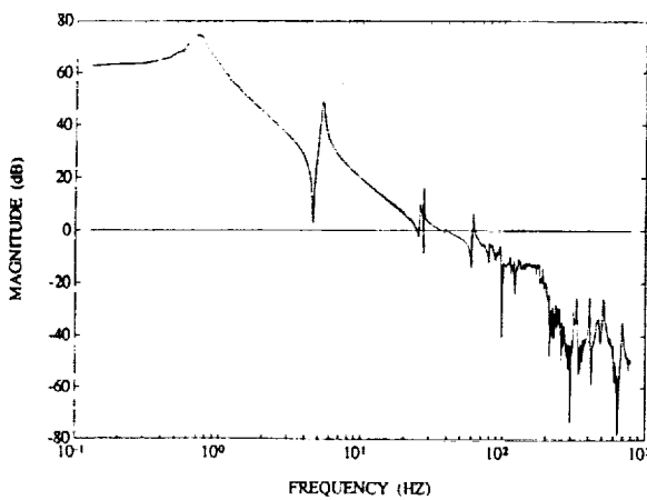
Figure 7. Voice Coil Loop Gain and Phase
