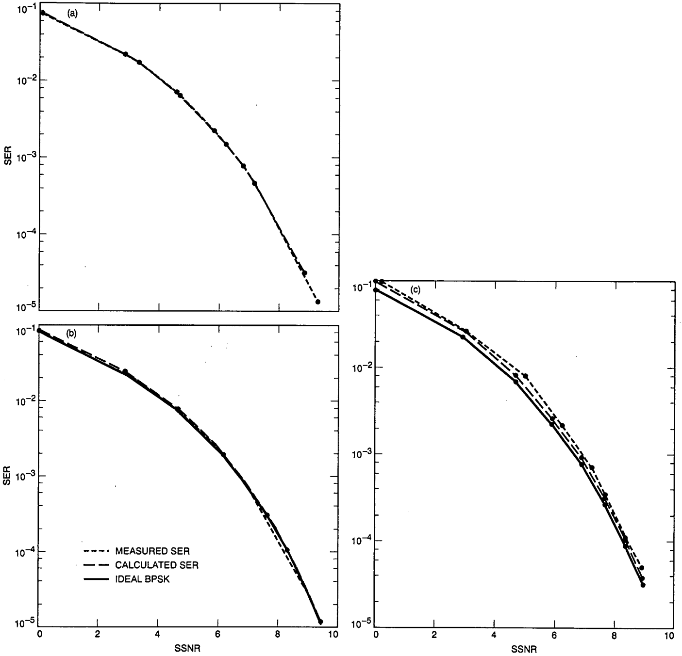
Fig. 15. Measured performance for PCM/PM/bi-phase: (a) ICR = -59.5 dB ( m = 1.1 rad, \gamma = 0.001 ); (b) ICR = -54.2 dB ( m = 1.3 rad, \gamma = 0.001 ); and (c) ICR = -40.2 dB ( m = 1.3 rad, \gamma = 0.005 ).
