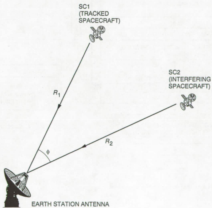
Fig. 2. Interference geometry for downlink.
