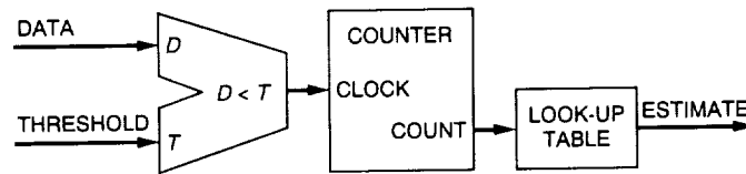
Fig. 2. Threshold-and-count estimator.
