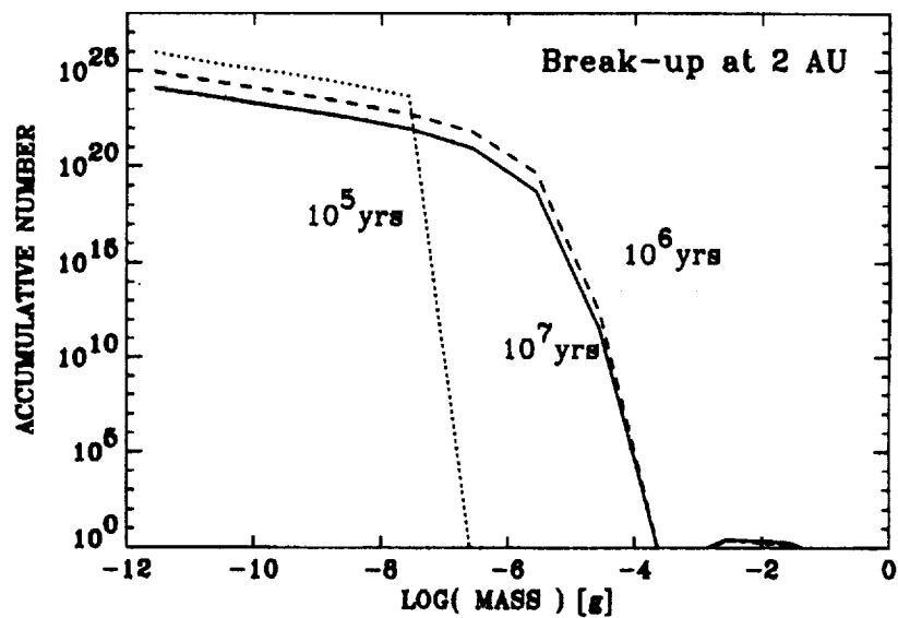
Figure 2. Size distribution at 1 AU of collisionally evolved debris from an asteroid that broke up near the inner edge of the asteroid belt. A nearly steady size distribution is attained within the first million years after the break-up. Meteoroids in the 10^{-2} g or 1 mm size range reach the Earth's orbit after 10^6 years but intermediate size particles are ground down before they reach the Earth.
