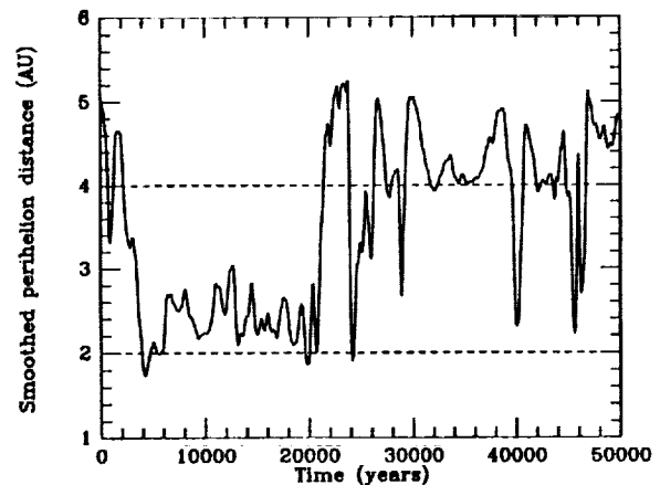
Figure 2. An example of orbital evolution for one comet. Plotted is the perihelion distance during 50000 years. The dashed lines show the chosen limits for the definition of a Jupiter family visit (see text).
