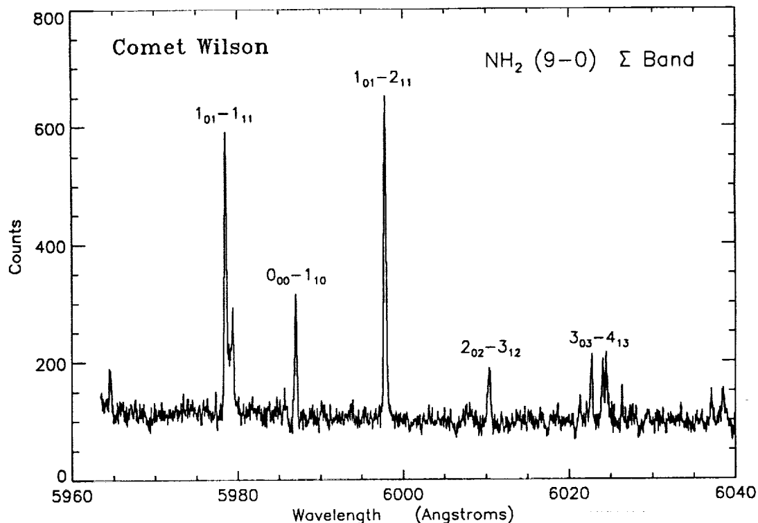
Figure 1. Spectra of the NH 2 (9-0) band for comet Wilson.
