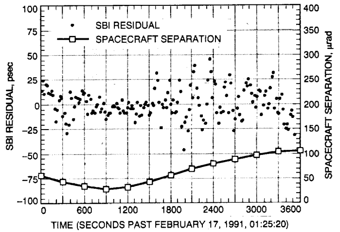
Fig. 6. Twenty-second MGN-PVO SBI residuals (S-band) for Goldstone-Canberra, February 17, 1991.
