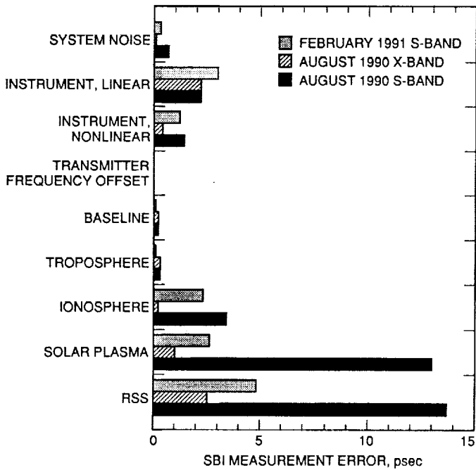
Fig. 2. Predicted SBI measurement errors for MGN-PVO for 5-min averages. Predicted X-band errors are shown for comparison only.
