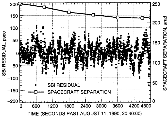
Fig. 5. Two-second MGN-PVO SBI residuals (S-band) for Goldstone-Canberra, August 11, 1990.
