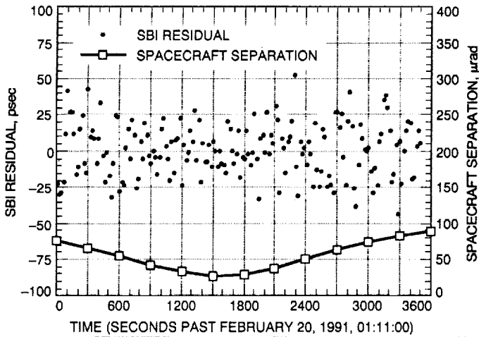
Fig. 7. Twenty-second MGN-PVO SBI residuals (S-band) for Goldstone-Canberra, February 20, 1991.
