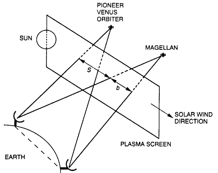
Fig. 3. Geometry of radio signals traversing the solar plasma.
