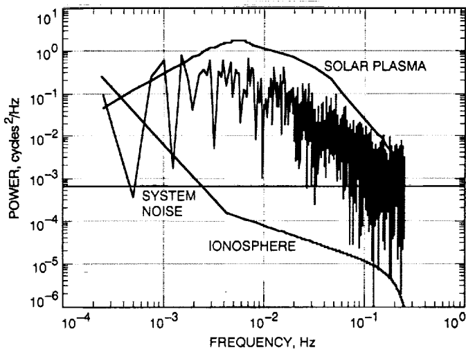
Fig. 8. Power spectrum of doubly differenced residual phase (S-band), observed and predicted, for Goldstone-Canberra, August 11, 1990.
