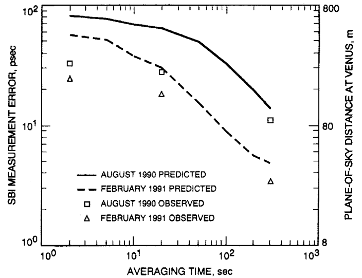
Fig. 10. Observed and predicted SBI measurement error (S-band) as a function of averaging interval.
