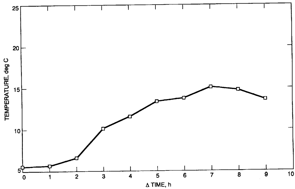
Fig. 5. Outdoor ambient temperature change during the 5 a.m.-2 p.m. run of Figs. 3 and 4.
