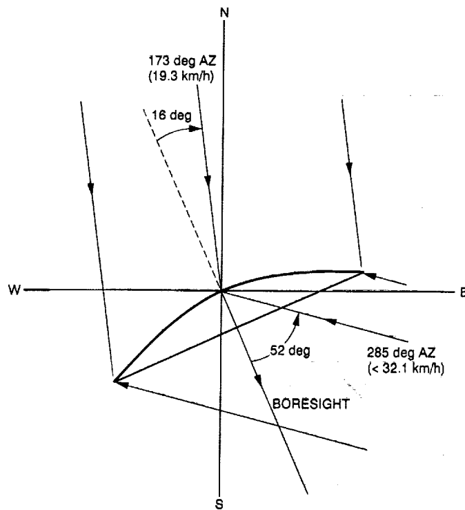
Fig. 7. Wind direction relative to the BWG antenna main axis during tests with the GSTAR I geostationary satellite.
