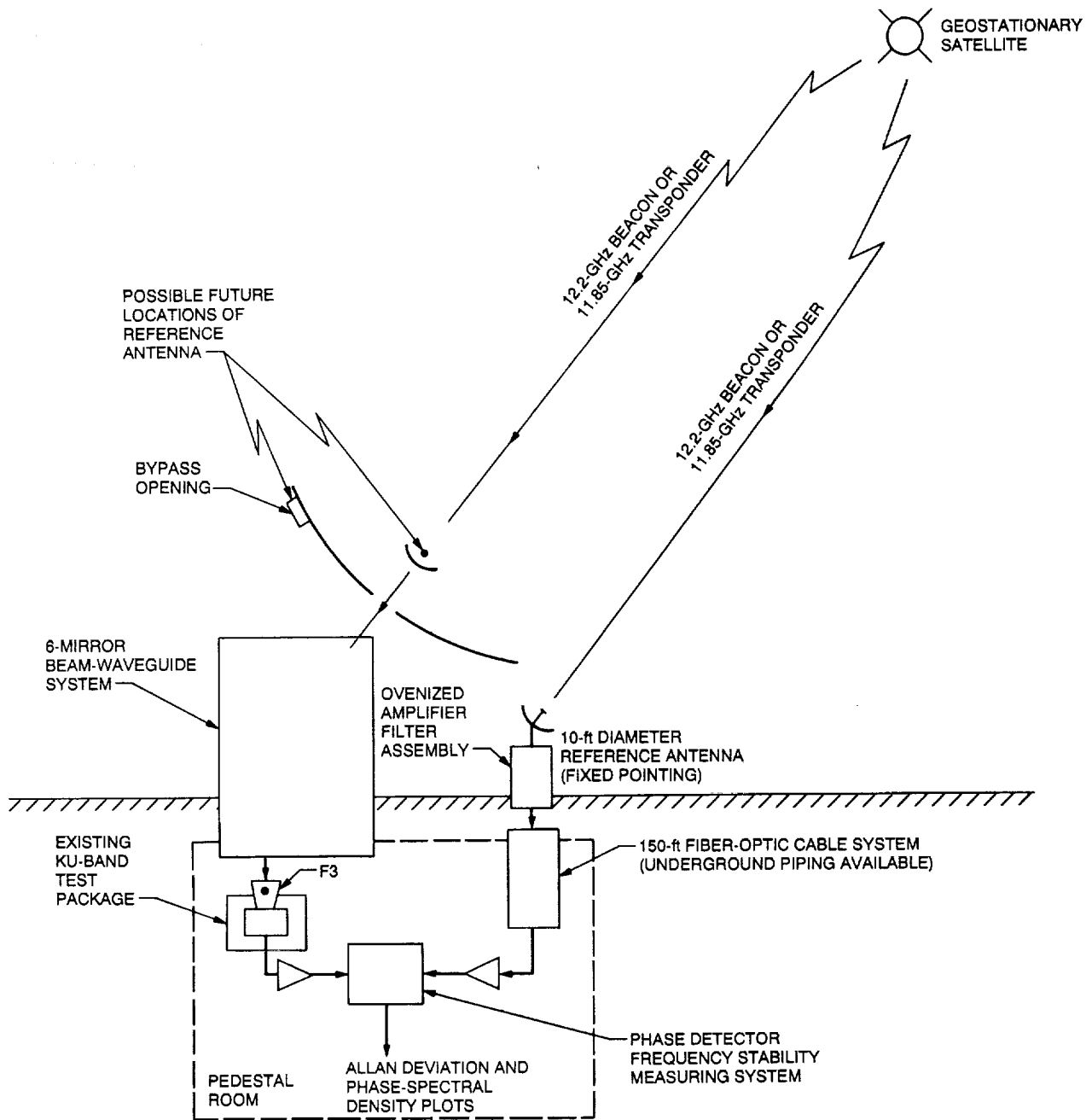
Fig. 1. Test configuration for measurement of the frequency stability of the DSS-13 BWG antenna.
