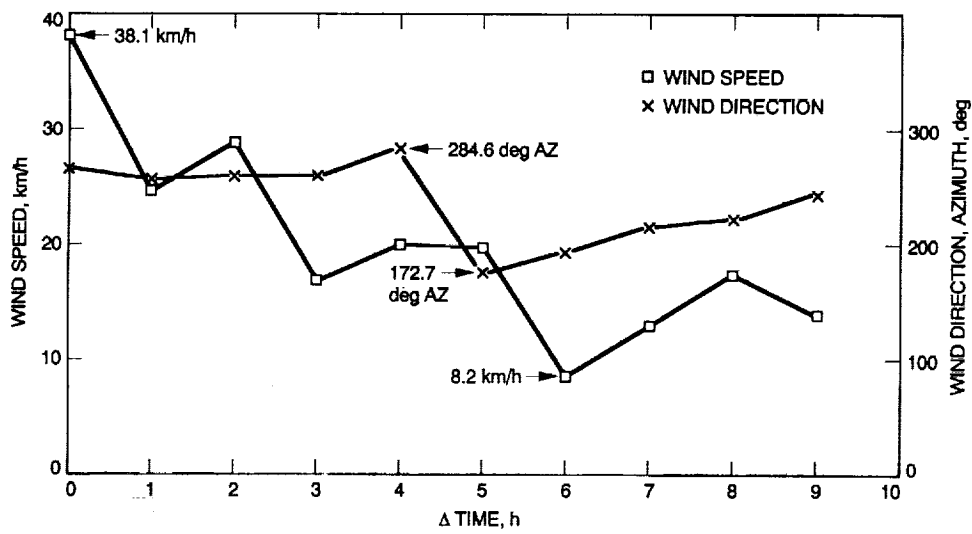
Fig. 6. Outdoor wind data during the 5 a.m.–2 p.m. run of Figs. 3 and 4.
