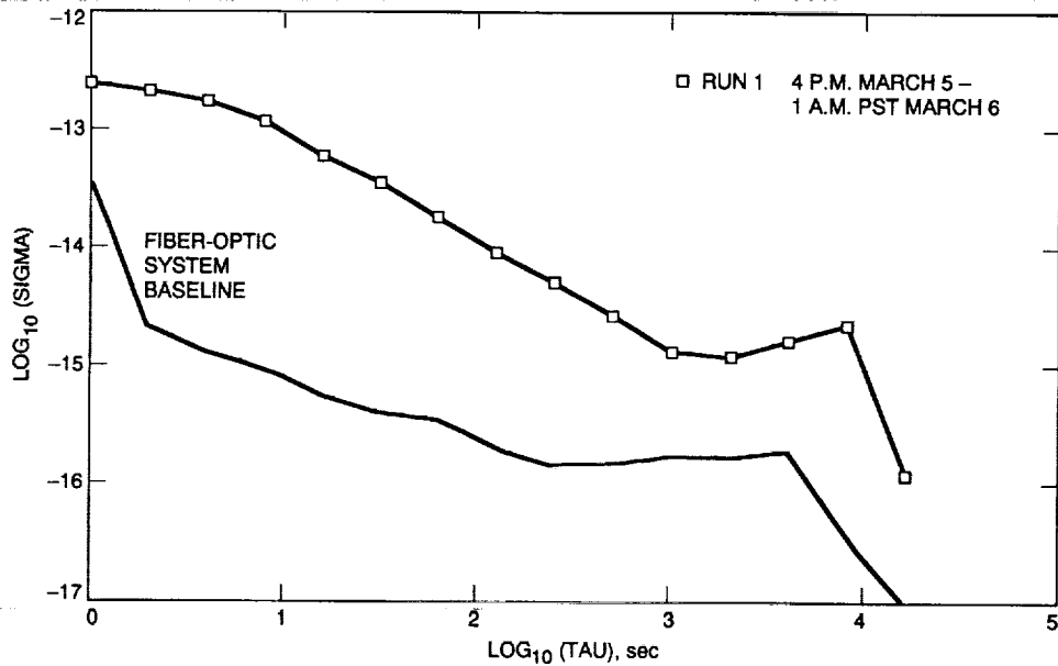
Fig. 10. Allan deviation plot of the DSS-13 BWG antenna stability on March 5 and 6, 1992. The DSS-13 BWG antenna was pointed at a 37-deg elevation angle and a 132.9-deg azimuth, receiving a 12.2-GHz beacon signal from Satcom K1.
