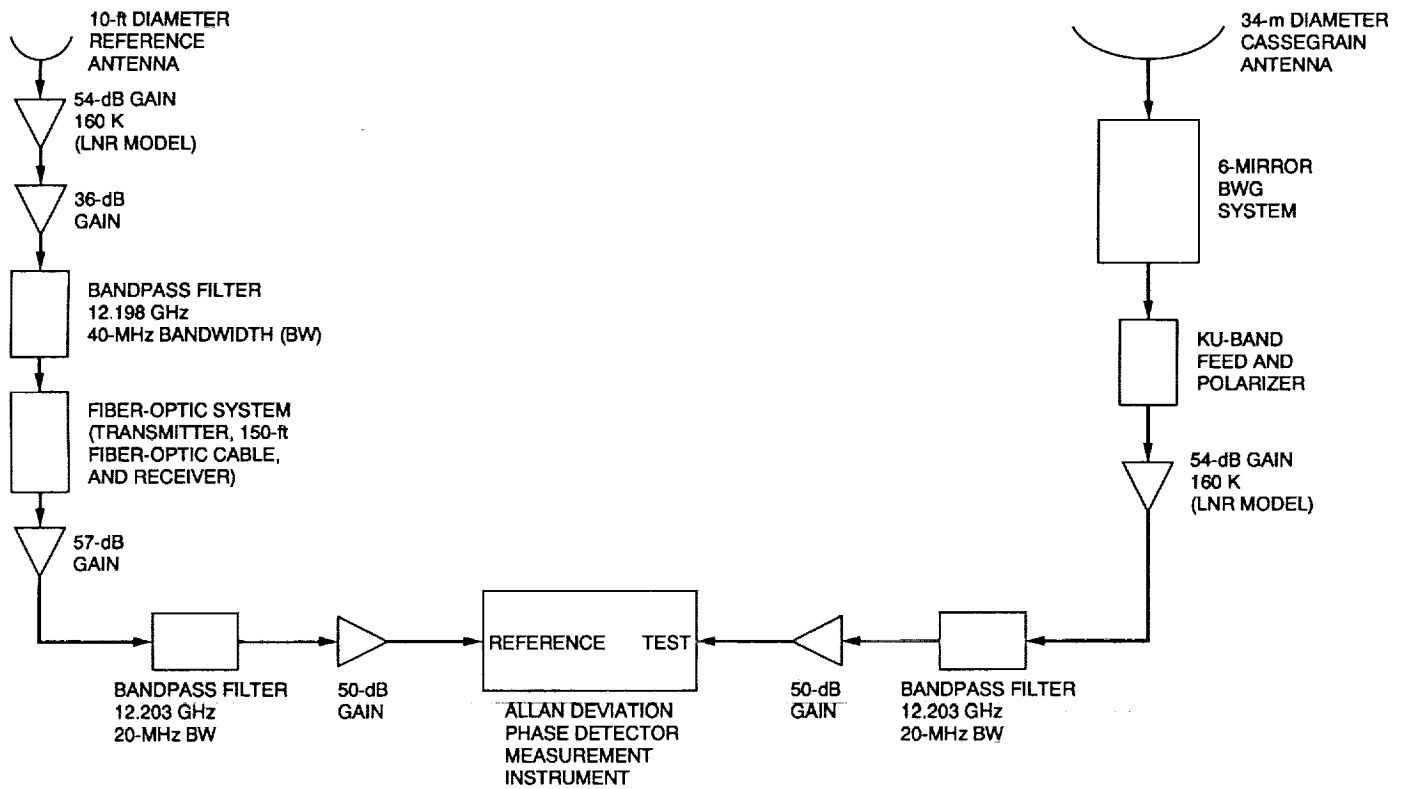
Fig. 2. The test configuration involving the use of the 12.2-GHz beacon signal from the GSTAR I geostationary satellite at a 46.5-deg elevation angle.
