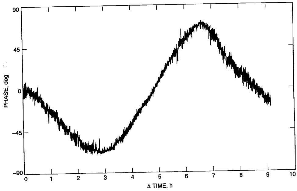
Fig. 11. Phase change plot corresponding to the 4 p.m.-1 a.m. run of Fig. 10.
