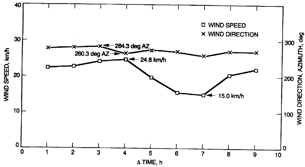
Fig. 13. Outdoor wind data during the 4 p.m.–1 a.m. run of Figs. 10 and 11.
