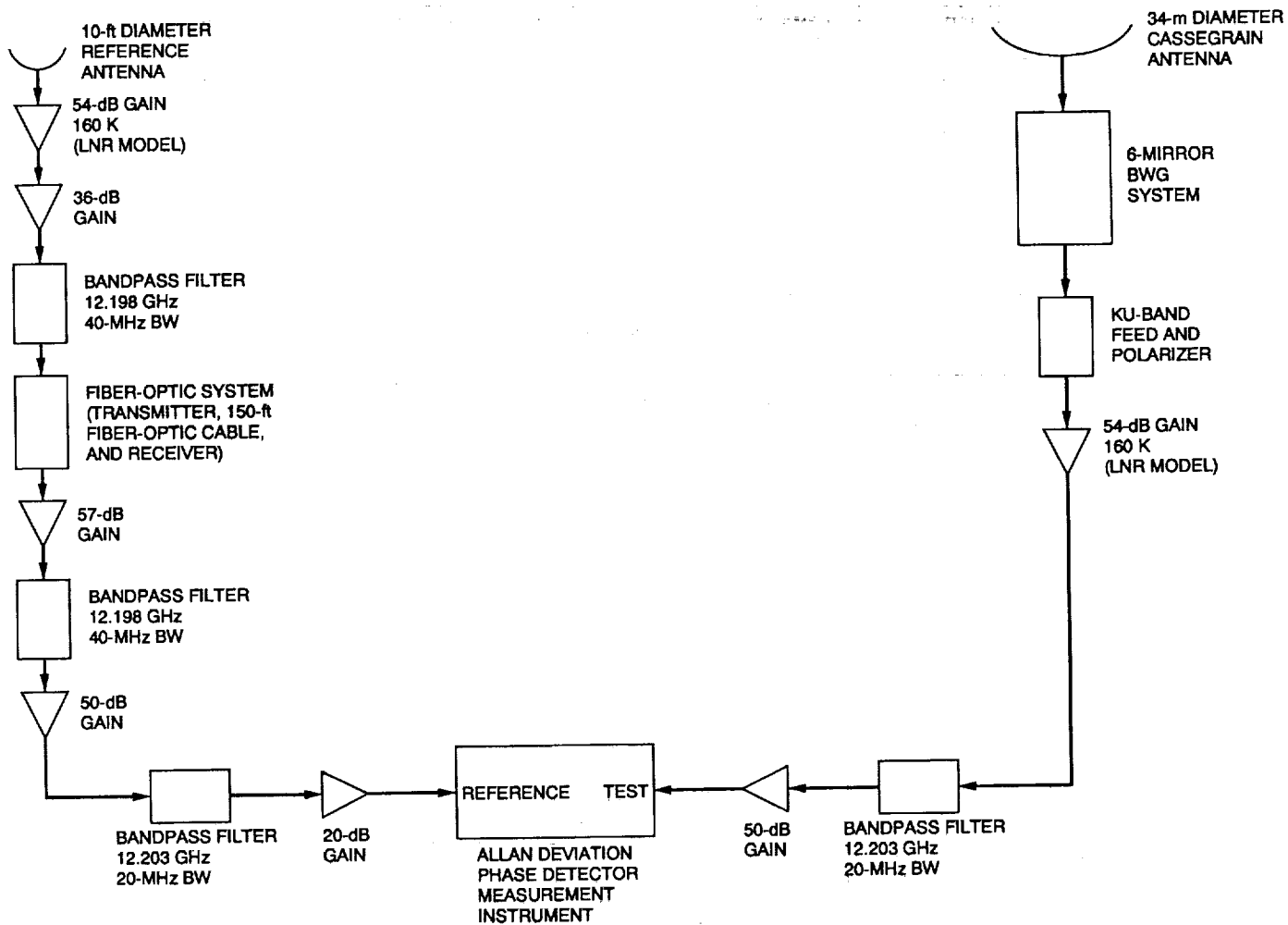
Fig. 8. The test configuration involving the use of the 12.2-GHz beacon signal from the Satcom K1 geostationary satellite at a 37-deg elevation angle.
