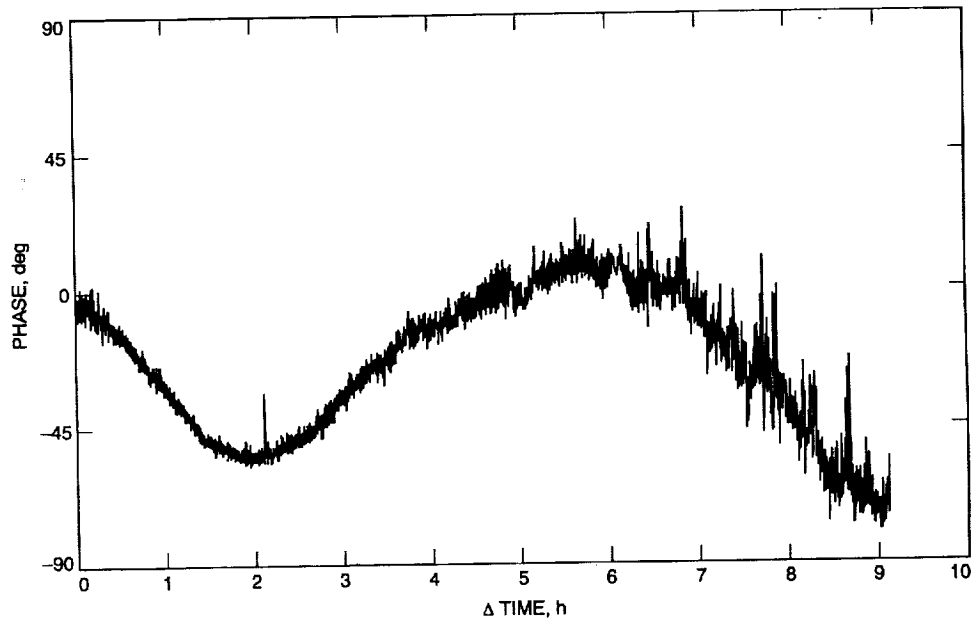
Fig. 4. Phase change plot corresponding to the 5 a.m.-2 p.m. run of Fig. 3.
