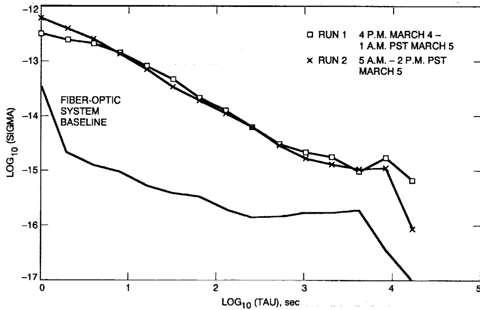
Fig. 3. Allan deviation plots of the DSS-13 BWG antenna stability on March 4 and 5, 1992. The DSS-13 BWG antenna was pointed at a 46.5-deg elevation angle and a 156.9-deg azimuth, receiving a 12.2-GHz beacon signal from GSTAR I.
