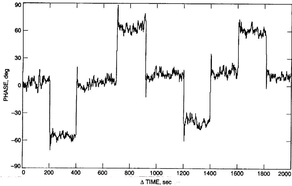
Fig. 9. Subreflector phase change plot as part of the precalibration procedure to verify test setup on 1992 day of year 66. The DSS-13 BWG antenna was pointed at a 37-deg elevation angle and a 132.9-deg azimuth, receiving a 12.2-GHz beacon signal from Satcom K1.
