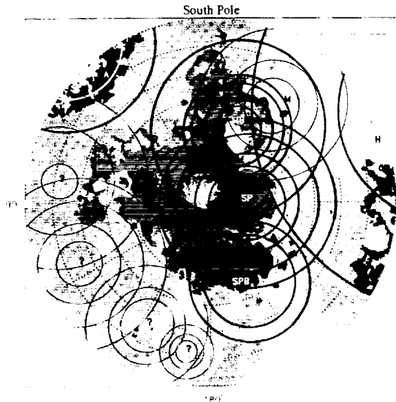
Fig. 1. Candidate large impact basins in the south polar region. Of particular interest are Malea B (MB), South Polar (SP), and South Polar B (SPB), which may have some control over the distribution of polar layered terrain ( Apl ) and other polar deposits ( Hdl , Hdu ). Also shown for reference are Argyre (A), Hellas (H), and Malea (M), as well as several much less certain candidates for which there is only weak and indirect evidence (?). Note the polar layered terrain ( Apl , shown as dark gray) lies within the extended influence of South Polar Basin, as inferred from concentric structures. Chasma Australe lies on an arc concentric to Malea B that also seems to control narrow valleys in the residual ice terrain ( Api , white inside dark gray), a distorted rim of a large crater near the Dorsa Argentea, and several very long ridges in Malea Planum (see text for details).
