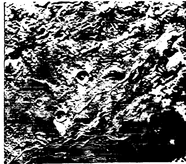
Fig. 2. Another view of Dorsa Argentea, showing also adjoining areas of etched terrain near latitude 76°S, longitude 30°. Solar illumination from top. Scene width 357 km. VO 421B16.
