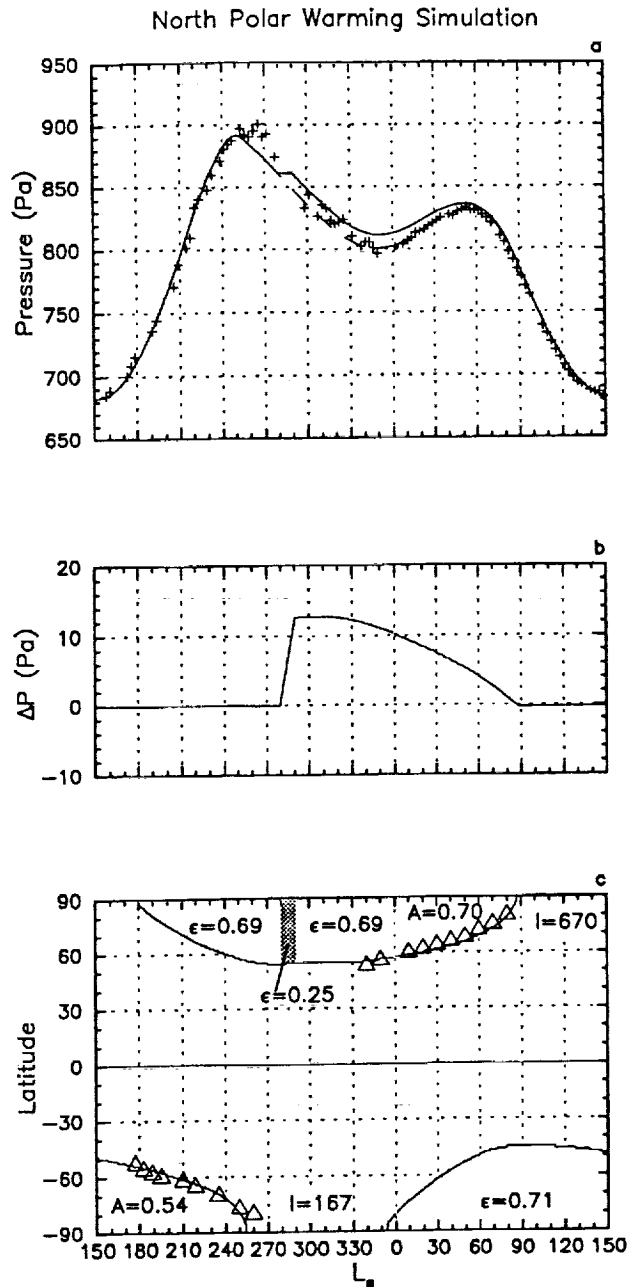
Fig. 1. (a) Model-calculated surface pressures (solid line) compared to VL1 year 3 binned data (pluses). The "standard best-fit" parameters [ A = frost albedo, \epsilon = frost emissivity, I = soil thermal inertia (MKS)] were used until the last year when the north seasonal polar cap \text{CO}_2 frost emissivity was lowered to 0.25 from L_s 280 to 290.5 to simulate north polar warming during the 1977B global dust storm. Dashed line indicates unperturbed "standard best-fit" pressure curve. (b) Interannual variation in atmospheric pressure calculated by subtracting the best-fit pressure curve from the perturbed model-calculated pressures. The pressure difference increased at a constant slope until the emissivity was reset to 0.69. (c) Latitudinal extent of model-calculated seasonal polar caps and Viking Orbiter observations (triangles) of the retreating cap edges in 1977 [27,28] shown for comparison.
