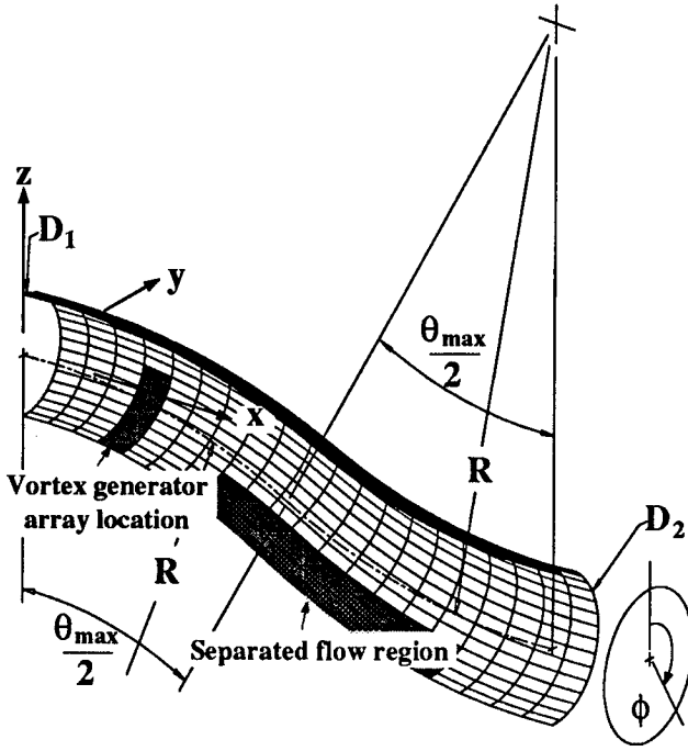
Fig. 1 Geometry of the diffusing S-duct Experimental Facilities and Techniques
