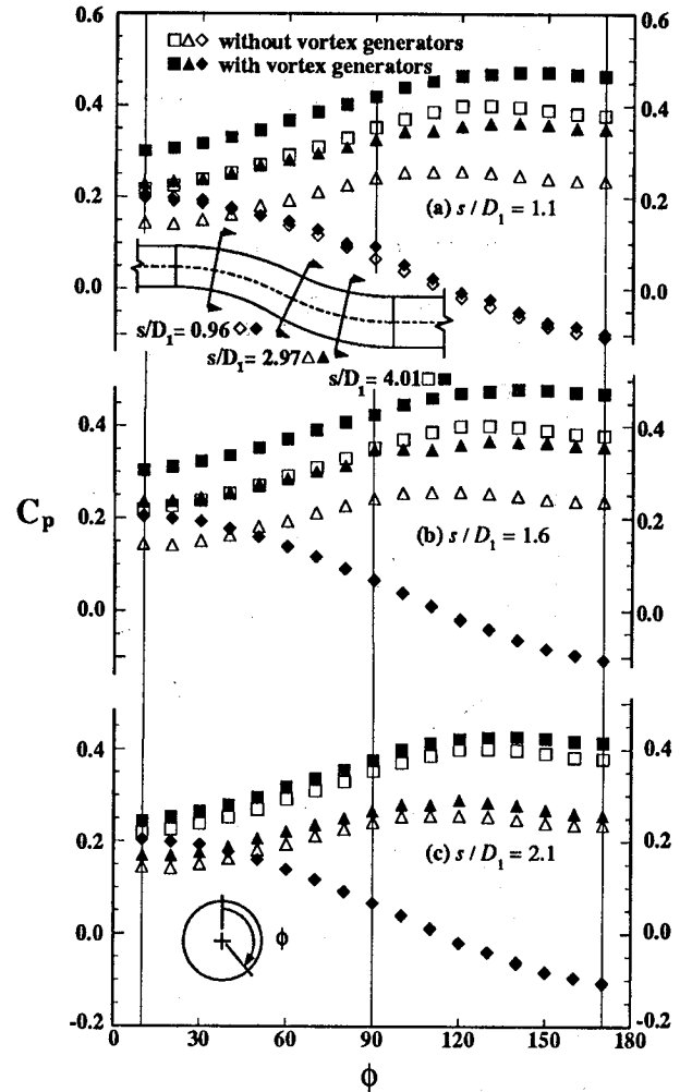
Fig. 9 Circumferential static pressure coefficient for variation of axial location of vortex generator
