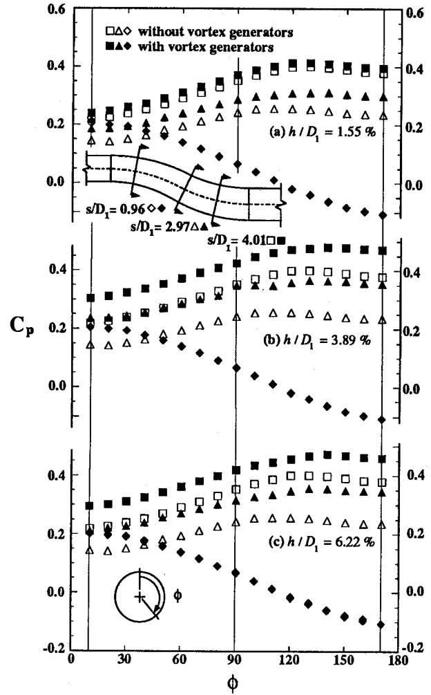
Fig. 5 Circumferential static pressure coefficient for variation of vortex generator height
