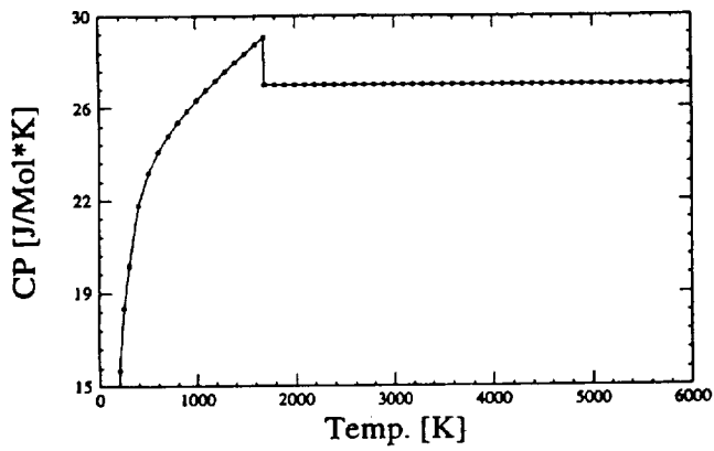
Original Data for Si (cr, \ell )
