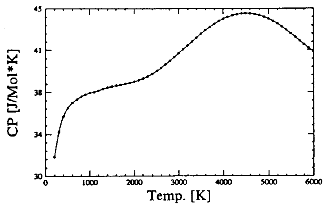
Coef Data for Cl 2
