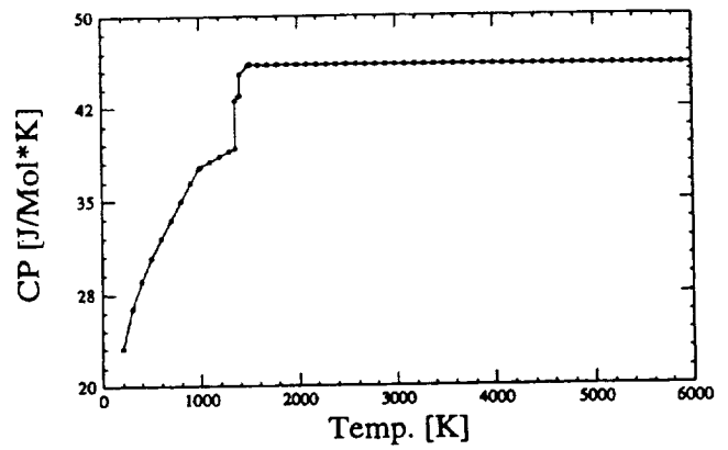
Coef Data for Mn ( \alpha, \beta, \gamma, \delta, \ell )
