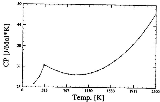
Coef Data for Na (cr, \ell )
