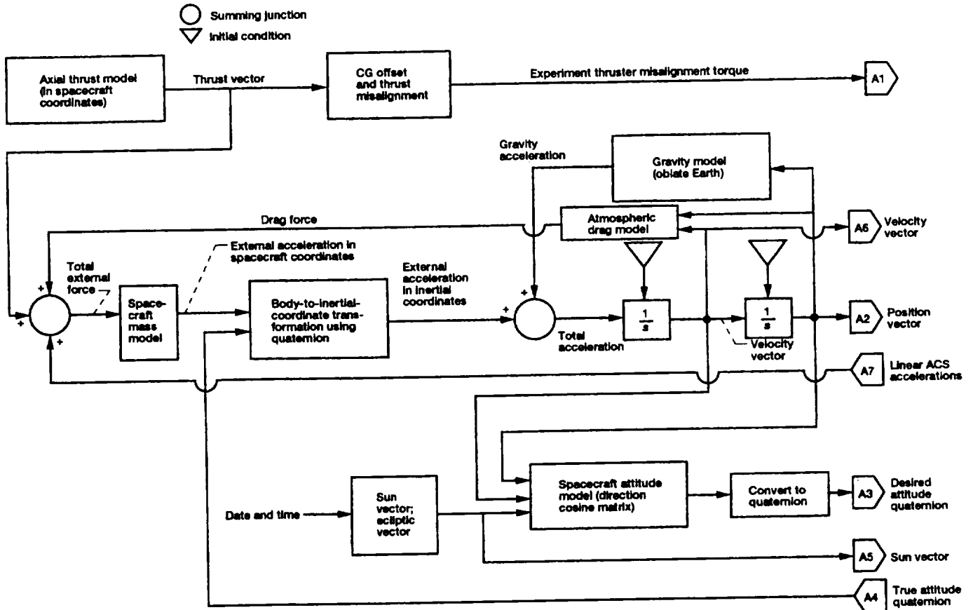
Figure 1.2.—Translation model.
