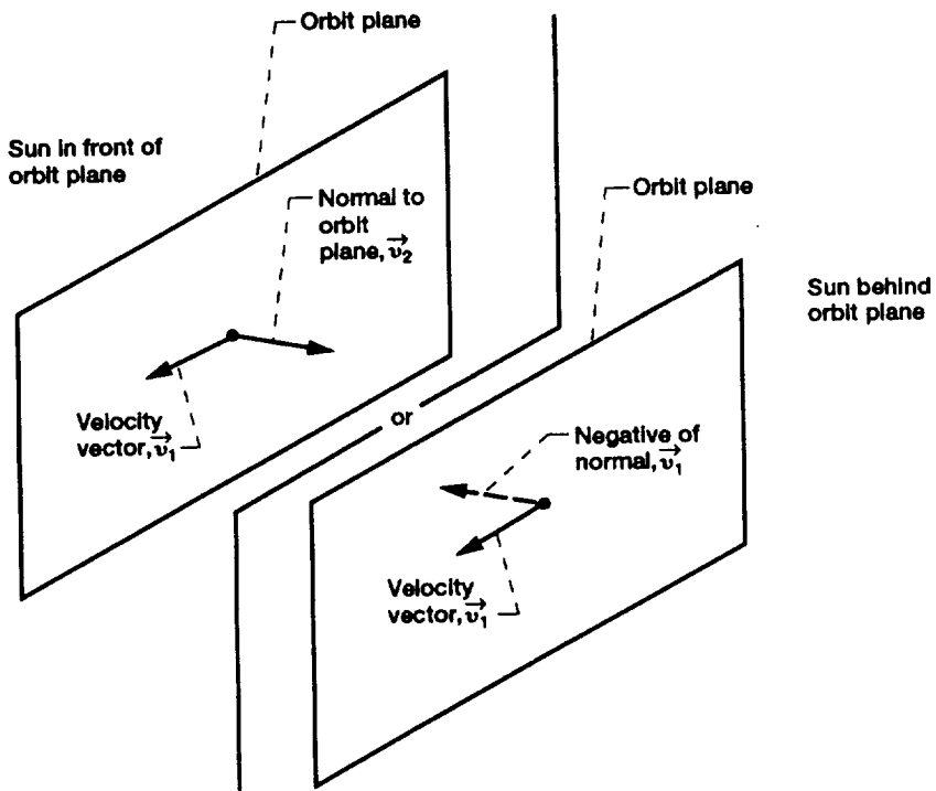
Figure 2.11.—Attitude option 8. (When the Sun crosses the orbit plane, the spacecraft rotates 180° about the velocity vector.)
