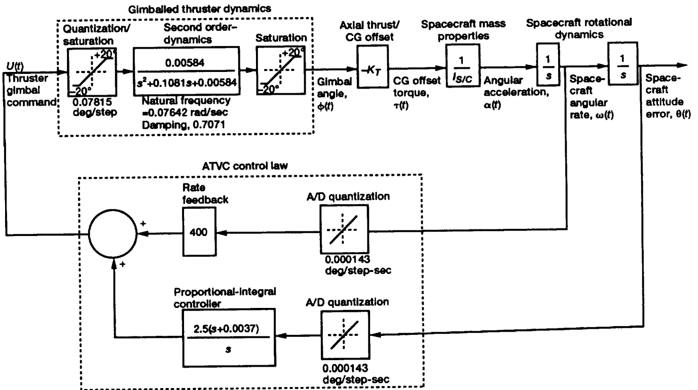
Figure 3.13.—Gimbaled thruster control loop (linearized, one axis).
