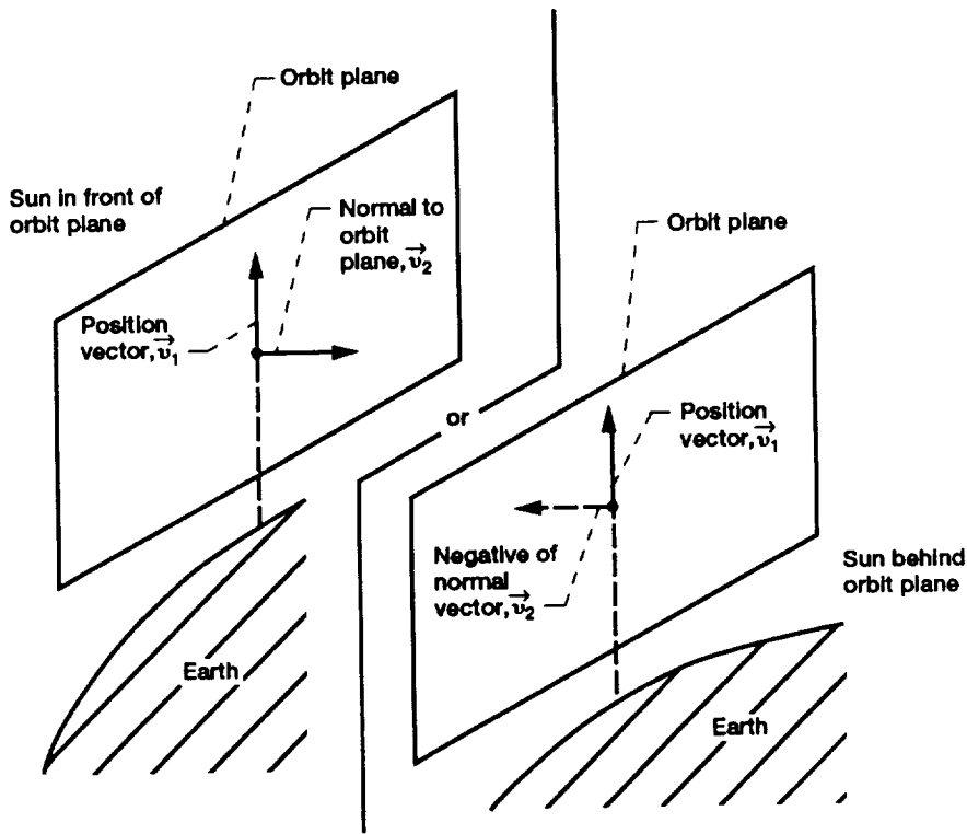
Figure 2.10.—Attitude option 7. (When the Sun crosses the orbit plane, the spacecraft rotates 180° about the velocity vector.)
