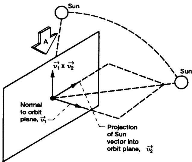
Figure 2.8.—Attitude option 5.
