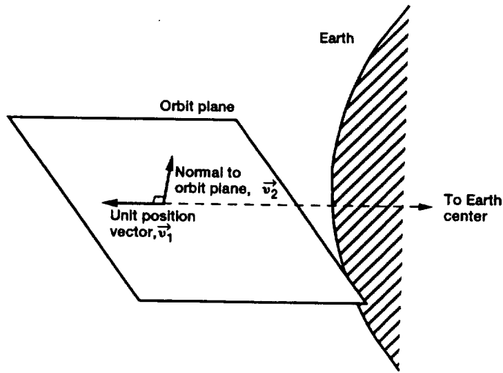
Figure 2.5.—Attitude option 2.
