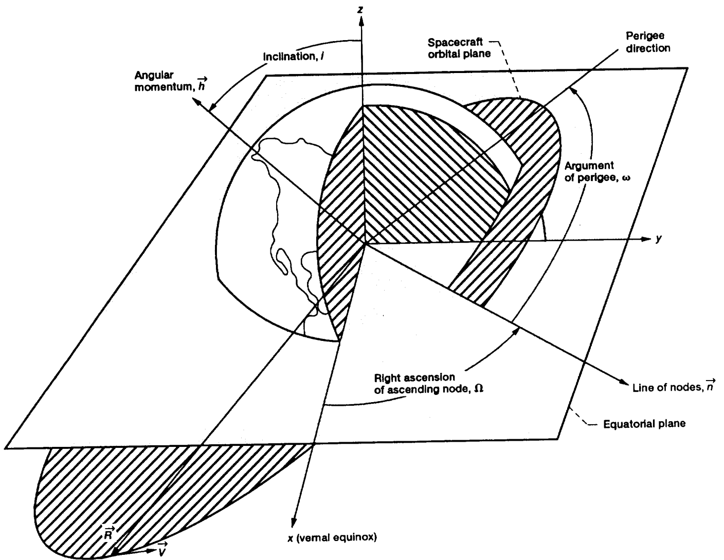
Figure 2.2.—Orbital elements.
