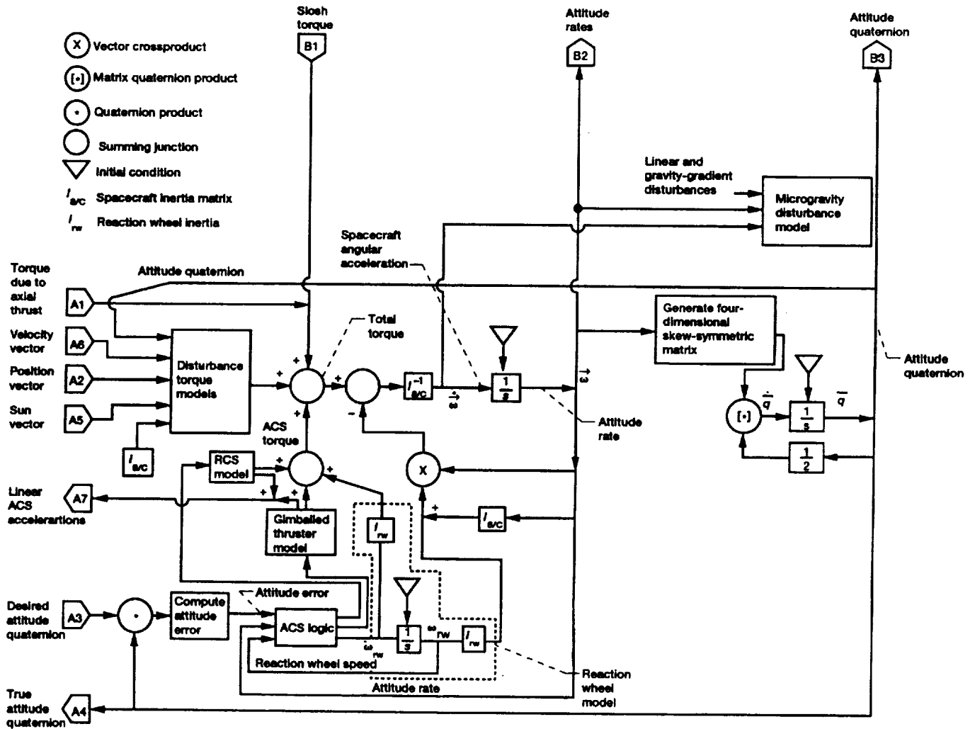
Figure 1.3.—Rotation model.
