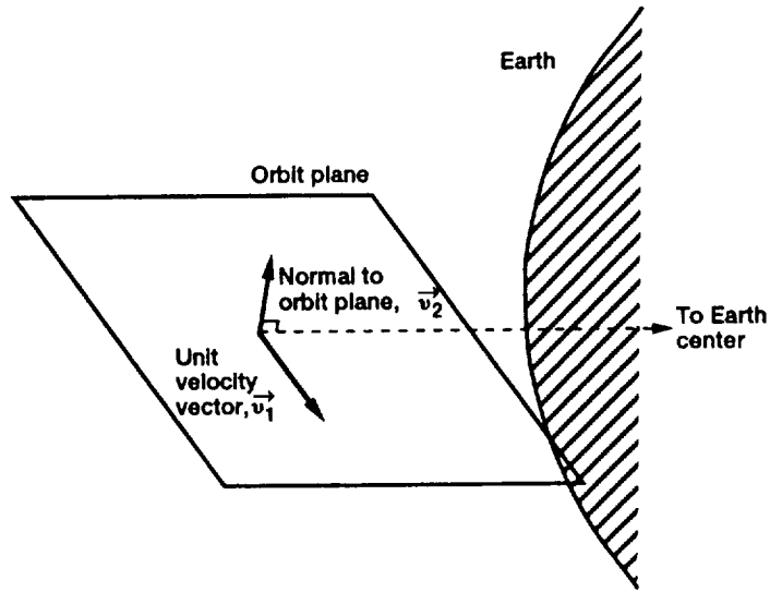
Figure 2.6.—Attitude option 3.
