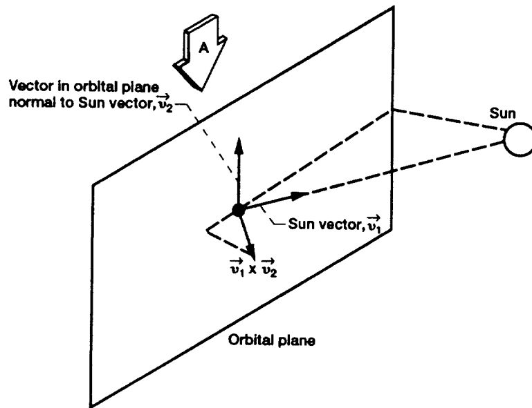
Figure 2.12.—Attitude option 9.
