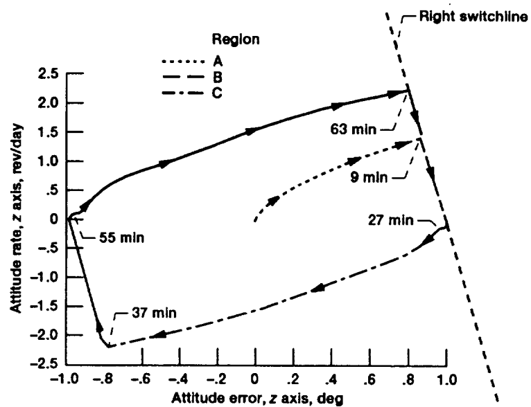
Figure 3.12.—Attitude-error and attitude-rate phase-plane trajectory.
