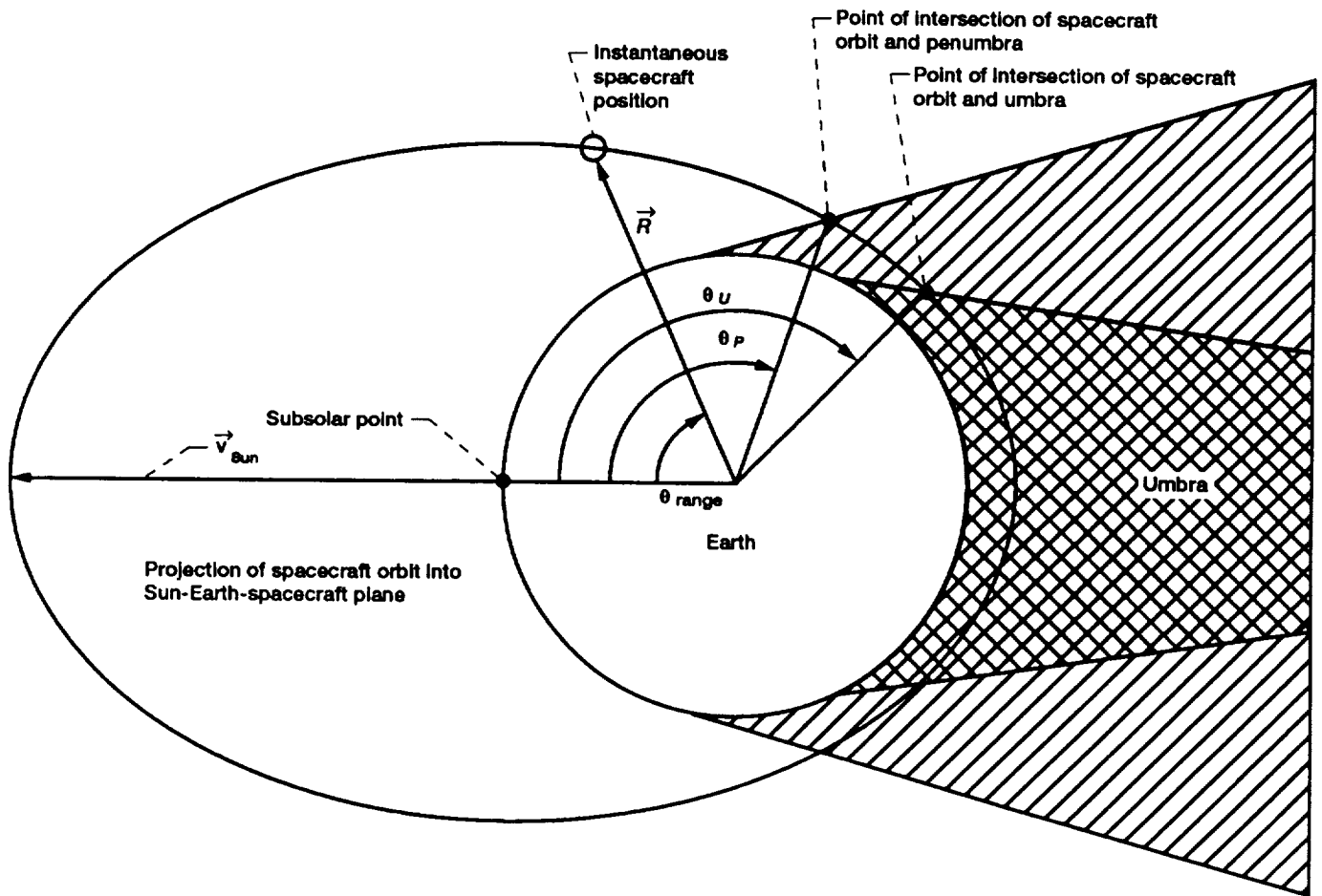
Figure 3.6.—Sun blockage.
