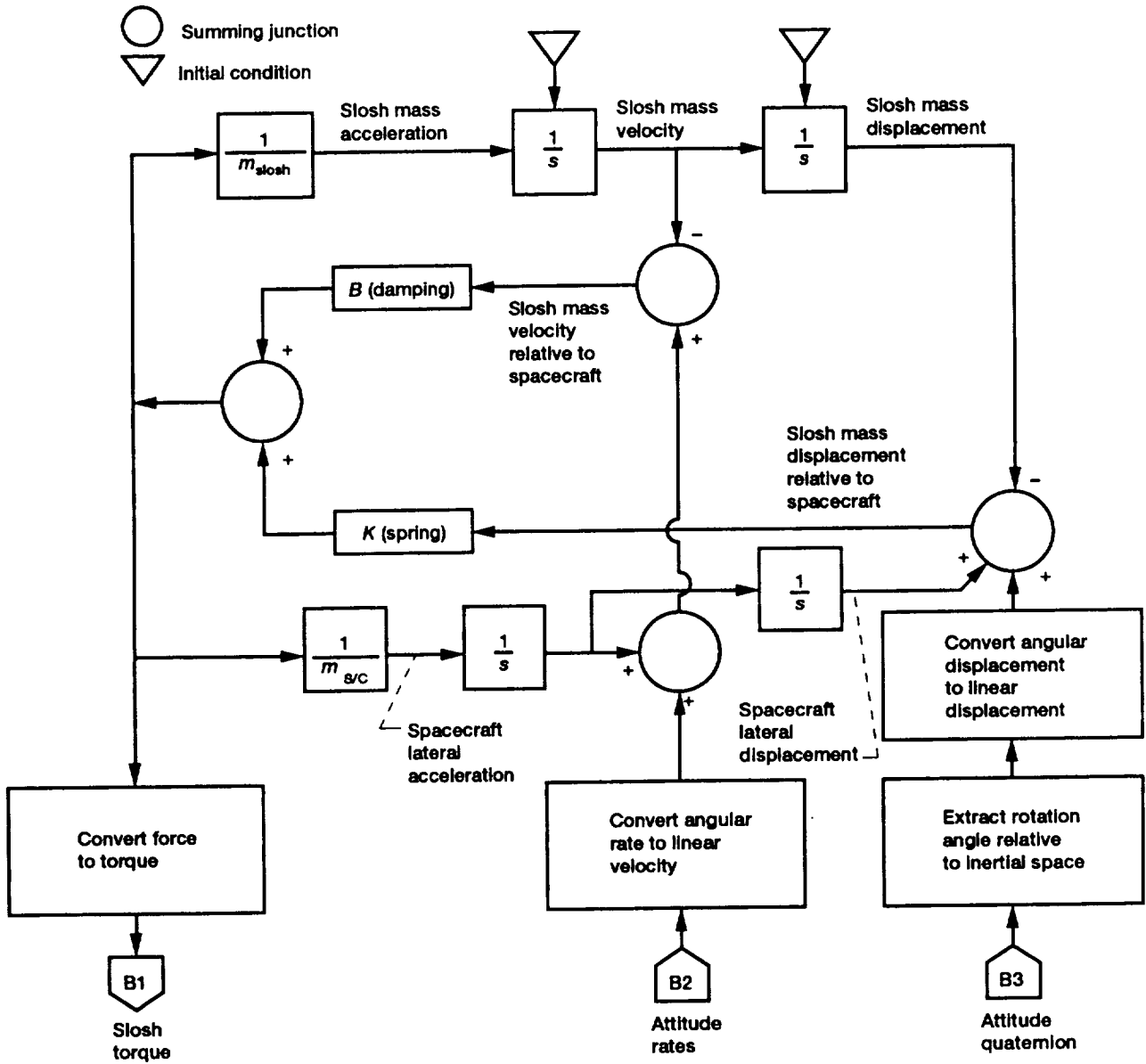
Figure 1.4.—Siosh model.
